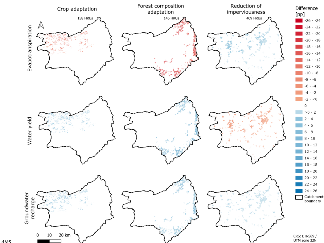
Figure 8: Differences in water flux coefficients between baseline and adaptation scenario by change categories, area-weighted, catchment outline based on GSK3E (LANUV, 2019)
