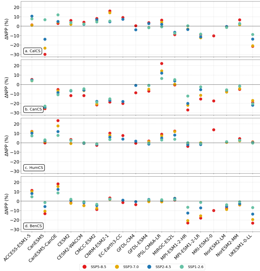
Figure 5. CMIP6 ensemble-mean NPP anomalies exhibit greater model uncertainty than scenario uncertainty. For each CMIP6 model, each point represents the NPP show regionally-contrasting trends within individual EBUS anomaly, with consistent patterns projected across models. Ensemble-mean averaged over the final 30 years of simulations (13 models) NPP anomalies (2071–2100–2071–2100 relative to 1985–2014) and spatially averaged across the entire system domains, under SSP5-8.5 in the four eastern boundary upwelling systems SSPs. Stippling highlights areas of high model agreement. The poleward and equatorward sub-EBUS are indicated in each map by black lines at the latitudes of 30° N (CalCS), 22° N (CanCS), 32° S (HumCS), and 24° S (BenCS).
