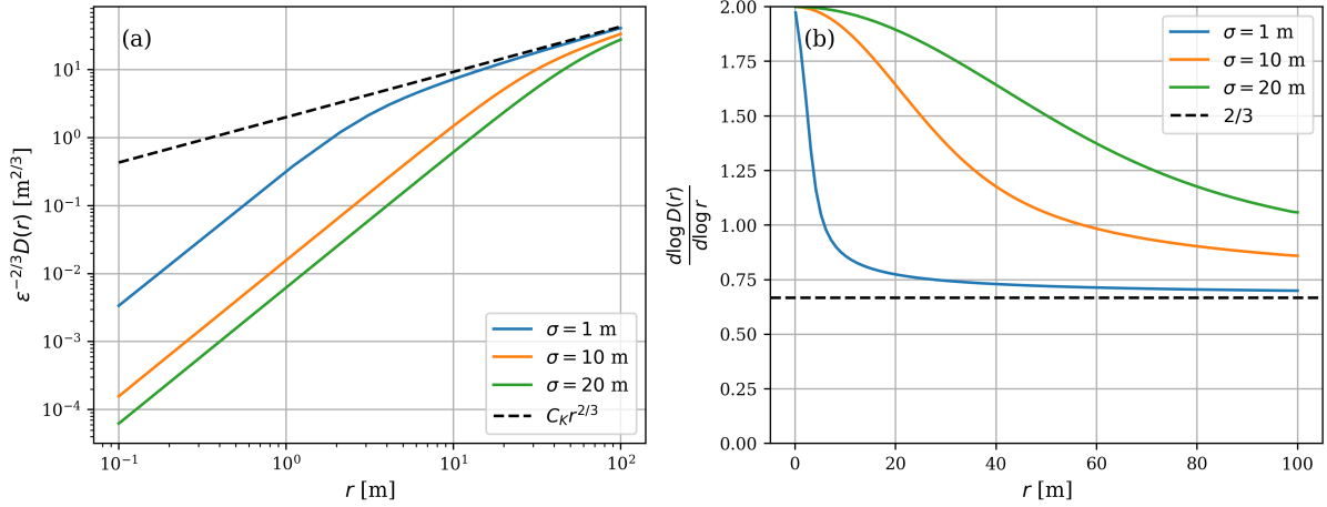
Figure 1. (a) Normalized structure function \varepsilon^{-2/3} D_{\text{lidar}}(r) (from Eq. 6) as a function of the separation distance r for three different values of \sigma : 1 m, 10 m, and 20 m. A C_K r^{2/3} reference line is also added. (b) d \log D(r) / d \log r as a function of r . The dashed black line represents a slope value of 2/3 .
