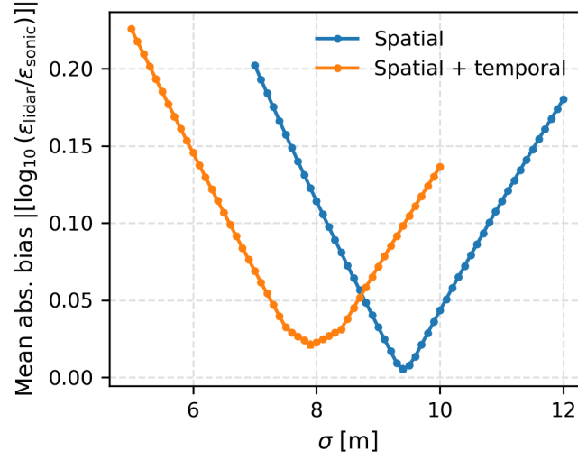
Figure 4. Mean bias or systematic error produced by fitting the modeled structure function over a range of \sigma values for the D_{\text{lidar}} models presented in Eq. (6) (spatial) and Eq. (7) (spatial+temporal averaging), respectively.
