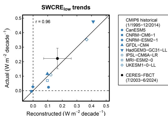
Figure 4. Comparison of actual and reconstructed trends in \text{SWCRE}_{\text{low}} . Blue symbols denote trends from individual CMIP6 models in the historical simulations during January 1995 to December 2014. The black circle shows CERES-FBCT values for July 2003 to June 2024, with error bars denoting \pm 1\sigma confidence intervals. The one-to-one line is shown in solid black.
