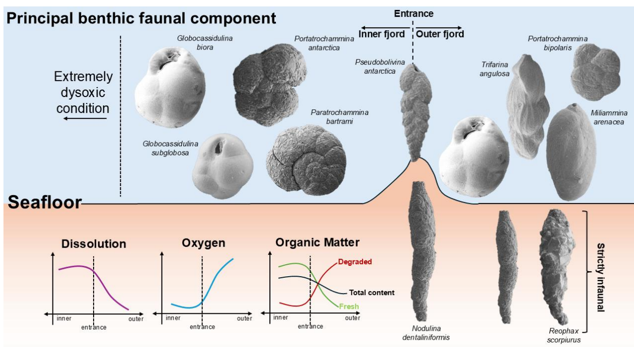
Figure 9. Conceptual cartoon of the Edisto Inlet benthic foraminiferal fauna and the major environmental factors (Dissolution, Oxygen, Organic Matter) that affects the benthic community and how they are distributed along the fjord transect, from innermost to outermost part. Species that have been found only below 1-cm were considered as strictly infaunal and are depicted inside the sediments. For a more detailed discussion readers are referred to the section 4.2. SEM photos of selected foraminifera are not in scale.
