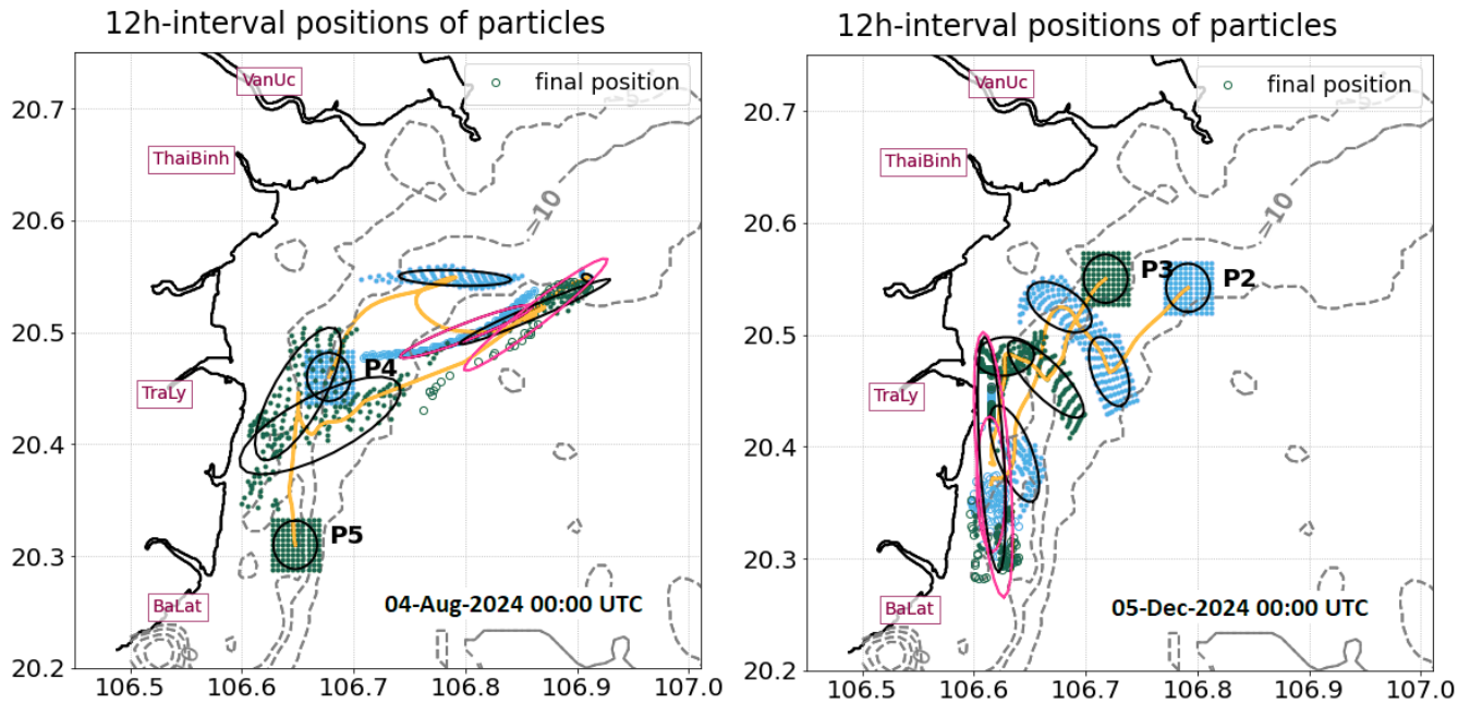
400 Figure 9: Positions of virtual particles at 12 h intervals for releases on 4 August (Case 1; a) and 5 December (Case 2; b). Solid dots indicate intermediate positions, and hollow dots indicate the final positions. Green and turquoise colors illustrate P4, P5 in (a); and P2, P3 in (b), respectively. Dispersion ellipses illustrate the spreading of particles. The ellipse representing the spreading at the final positions is shown in pink.
