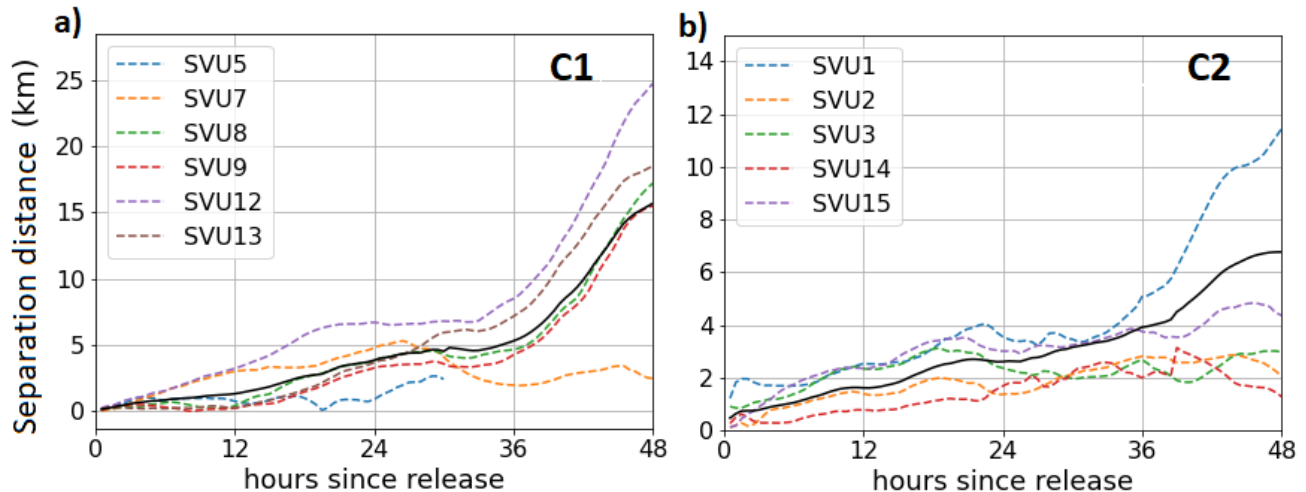
Figure 6: Separation distances between virtual and real trajectories for C1 (a) and C2 (b), black solid lines are separation distances averaged over all buoys within each cluster.
