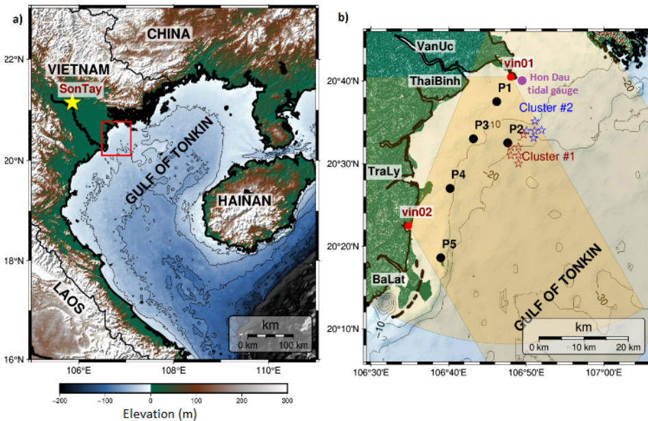
165 Figure 1: a) Map of the GoT, Son Tay hydrological station is marked by the yellow star, the red rectangular shows the RR plume domain; b) Map of RR plume area, Yellow areas indicate the coverage of the two HFR stations. Drifter locations are denoted by red stars for C1, released on 30 November 2024, and blue stars, for C2 released on 3 December 2024. Black dots show locations of virtual clusters selected for particle tracking. Red dots are locations of two radar stations (vin01, vin02). The purple dot represents the Hon Dau tidal gauge. Names of main rivers are highlighted with white boxes. Black solid lines indicate depth contours of 10, 20, and 30 m.
