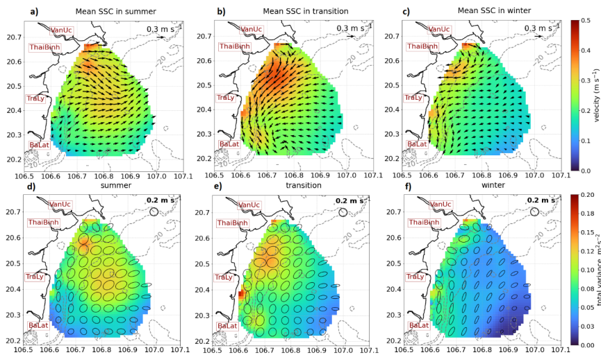
Figure 8: Mean surface current velocity fields (a, b, c) during summer (August 2024), transition period (mid-September – October 2024), and winter (December 2024), respectively; and ellipses of current velocity variance superimposing total variance of surface current velocity (d, e, f).
