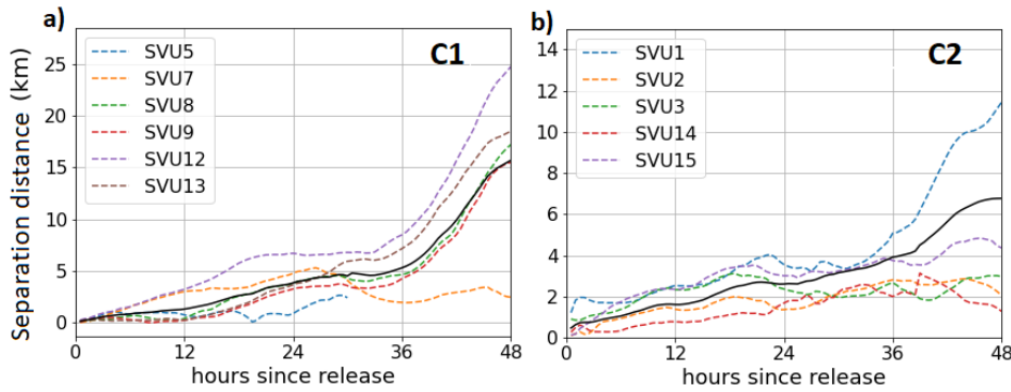
400 Figure 6: Separation distances between virtual and real trajectories for C1 (a) and C2 (b), black solid lines are separation distances averaged over all buoys within each cluster.
