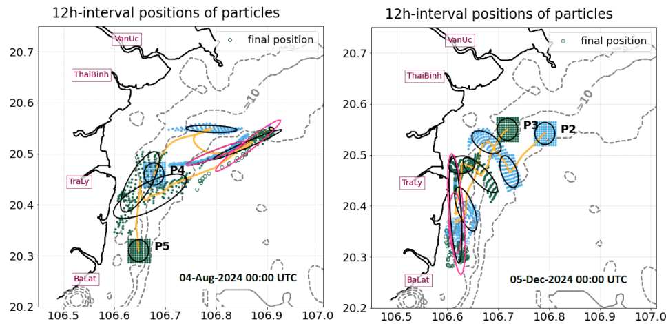
Figure 9: Positions of virtual particles at 12 h intervals for releases on 4 August (Case 1; a) and 5 December (Case 2; b). Solid dots indicate intermediate positions, and hollow dots indicate the final positions. Green and turquoise colors illustrate P4, P5 in (a); and P2, P3 in (b), respectively. Dispersion ellipses illustrate the spreading of particles. The ellipse representing the spreading at the final positions is shown in pink.
