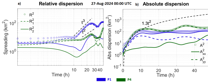
Figure 13: Relative (a) and absolute (b) dispersion of particles in clusters P1 (blue) and P4 (green) on August 27 (Case 3). Black dashed lines represent curves of different regimes: ballistic ( \delta^2 \sim t^3 ), Richardson super-diffusive dispersion ( \delta^2 \sim t^2 ), and ballistic regime for absolute dispersion ( A(t)^2 \sim at^2 ).
