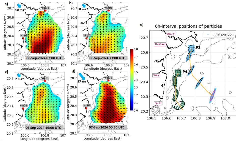
Figure 14: Surface current velocity fields at 6 h interval on September 6, before Yagi typhoon landfall (Case 4), colorbar in m s -1 , upper-left blue arrows demonstrate wind direction and speed (a-d); Accordingly, (e) Positions of particles at 6 h intervals, released off the river mouths: P1 (Van Uc, turquoise ) and P4 (Tra Ly, green)
