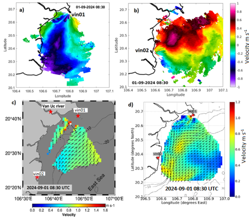
200 Figure 4: Radial current velocity fields obtained from MIO software at Vin01 (a) and Vin02 (b) stations. Surface current velocity maps before (c) and after applying radar processing procedure (d).
