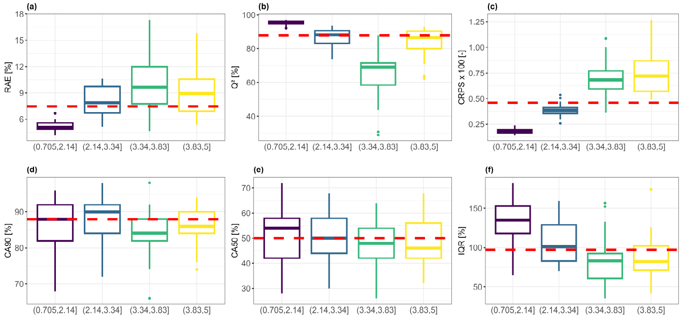
285 Figure 5: Boxplot of the RAE (a), Q^2 (b), CRPS (c), CA at level 90% (d), CA at level 50% (e), and IQR (f) performance criterion for different ranges of GSAT values (indicated on the x-axis). The performance statistics are computed over test samples unseen during emulator training by applying the validation procedure described in Sect. 2.4.1 repeated 25 times. The horizontal red dashed line indicates the median value calculated over all validation tests considering the whole range of GSAT.
