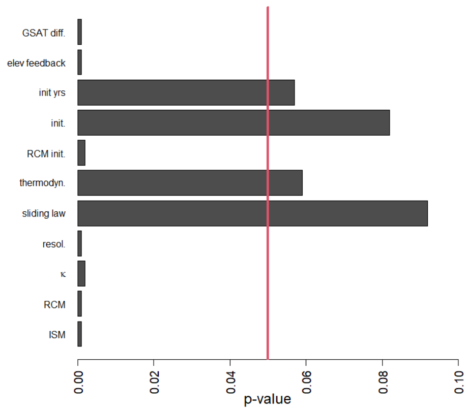
795 Figure C1: Screening analysis showing the p-values of the RF variable importance-based test of independence of Altmann et al. (2010). The vertical red line indicates the significance threshold at 5%. When the p-value is below 5%, it indicates that the null hypothesis should be rejected, i.e., the considered variable has a significant influence, and should be retained in the RF construction.
