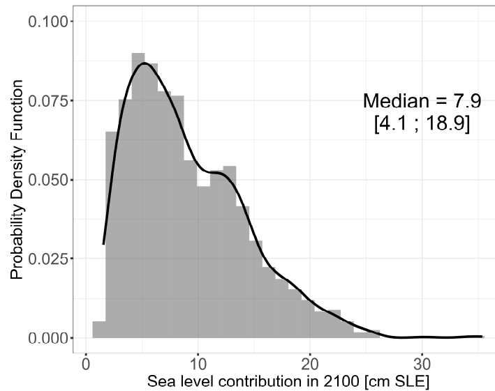
Figure 4: (a) Probability density function of the sea level contribution of the Greenland ice-sheet in 2100, with respect to 2014, based on the raw MME ensemble data considered in this study assuming that each member has the same weight. The black straight line provides the smoothed density function. The median value and the likely range (66% confidence interval) are also indicated.
