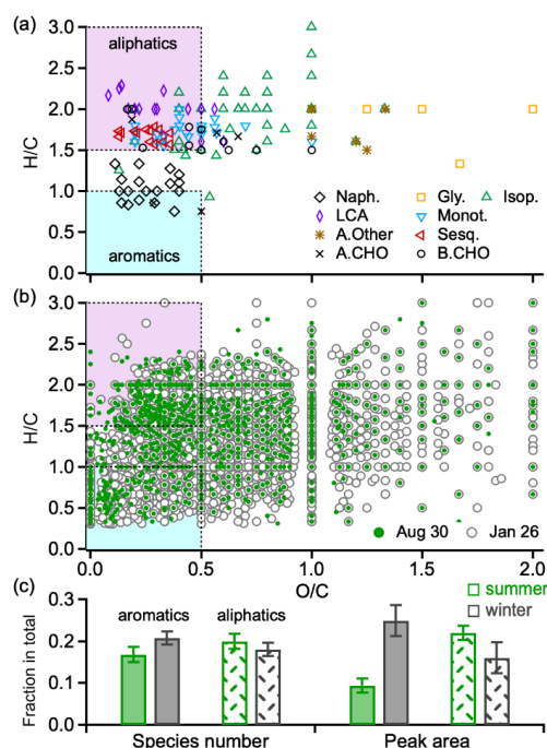
Figure 8. van Krevelen diagrams plotting of (a) organic tracer species derived from anthropogenic and biogenic precursors (as listed in Table S1–S3) and (b) organic molecular species identified on a summer day (August 30) and a winter day (January 26) in negative ESI mode. (c) Averaged number and peak area fractions of organic species in aromatic and aliphatic molecular structures for summer and winter samples. In panels (a, b), the shaded pink ( H/C \geq 1.5 , O/C \leq 0.5 ) and cyan ( H/C \leq 1.0 , O/C \leq 0.5 ) areas represent aliphatic and aromatic regimes, respectively. The O/C was replaced by (O-3S)/C or (O-3S-2N)/C in the case of organosulfates or nitrooxy-organosulfates. The error bars in panel (c) represent 1\sigma standard deviations for all the samples in each season.
