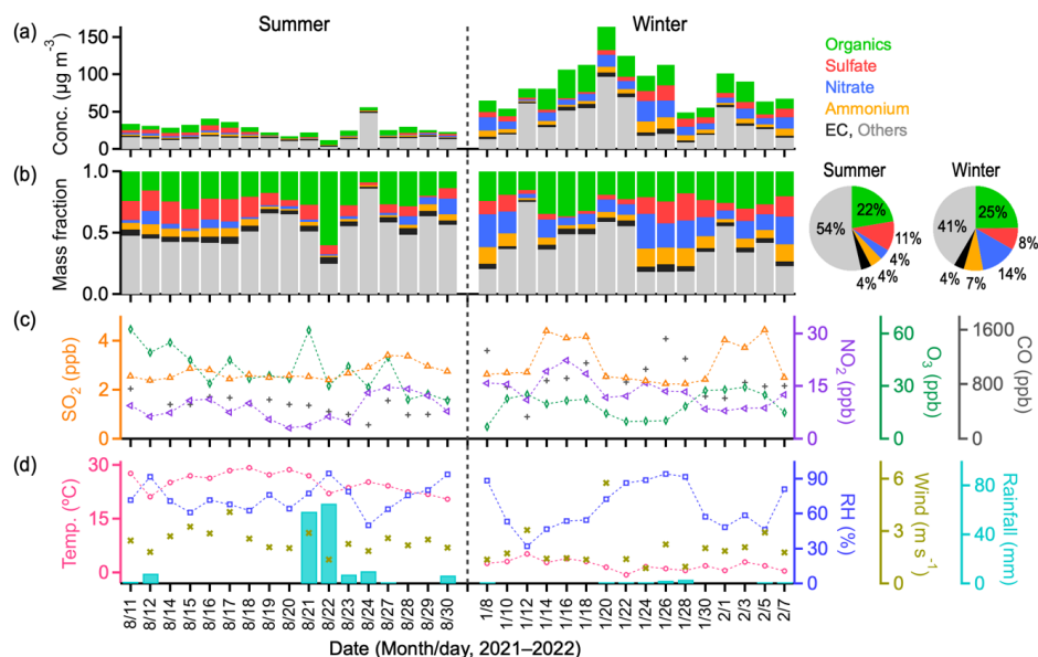
Figure 2. Temporal variations of the (a) mass concentrations and (b) mass fractions of chemical components in ambient PM_{2.5} , (c) gas pollutant concentrations, and (d) meteorological factors over the studied periods in 2021/2022. The two pie charts in panel (b) represent the averaged mass fractions of PM_{2.5} components in summer and winter periods.
