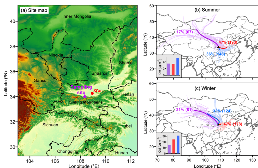
95 Figure 1. (a) A map showing the sampling site at northern foothill of the Qinling Mountains region in central China. (b, c) Back trajectories of air masses arrived at 500 m above the ground level over the sampling site and their cluster analysis (represented by the thick solid lines with percentages and numbers) during the summer and winter periods. The bottom left panels in panels (b, c) present the mass concentrations of organic matter in the corresponding air mass directions.
