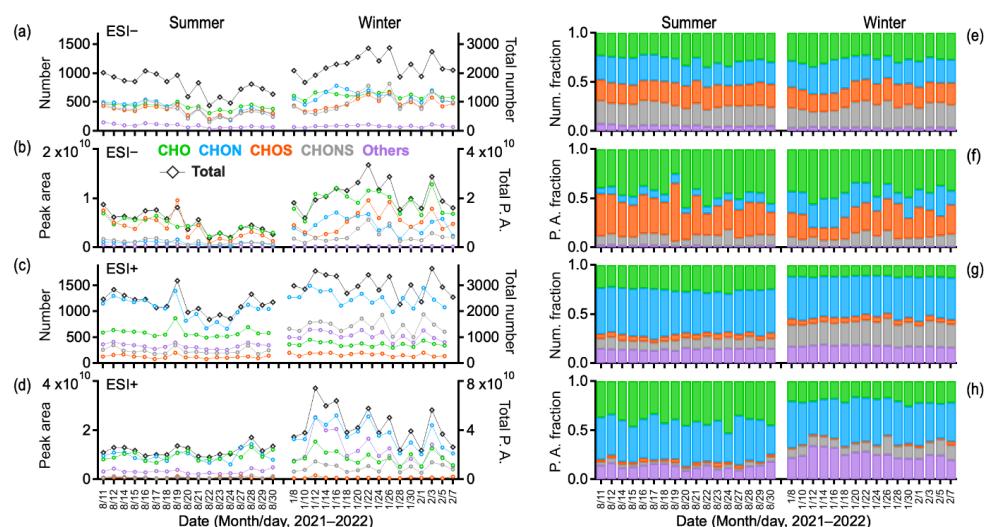
Figure 3. (a, c) Species number and (b, d) peak area intensity of organic molecular composition (including each subgroup and total species), along with their corresponding number and peak area fractions (e–h), obtained from the UHPLC–HRMS analysis in negative and positive ESI modes over the study periods.
