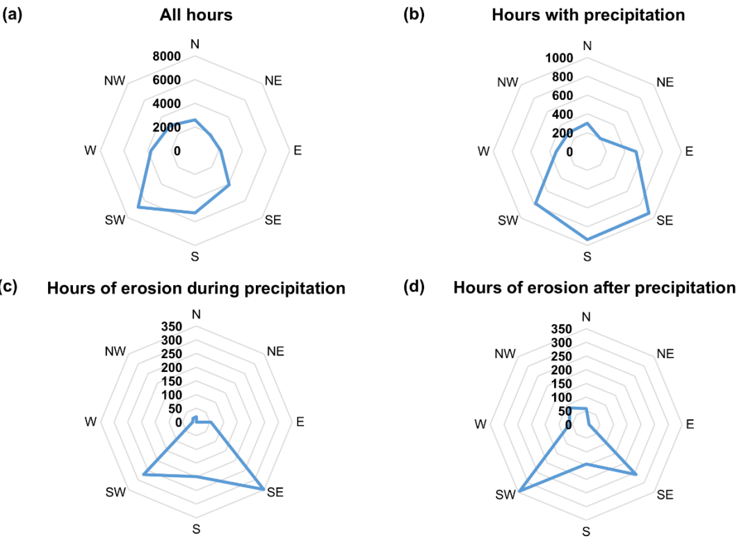
Figure 3: Frequency of wind direction for (a) all hours of observations, (b) hours with precipitation, (c) hours of erosion during precipitation, and (d) hours of erosion after precipitation.
