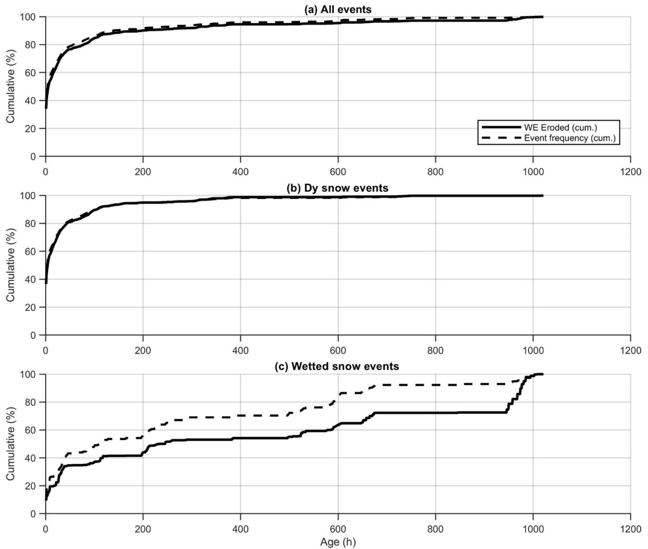
370 Figure 8: Cumulative relative frequency distributions and cumulative relative SWE eroded as a function of layer age. Panels show (a) all events, (b) dry snow events, and (c) wetted snow events.
