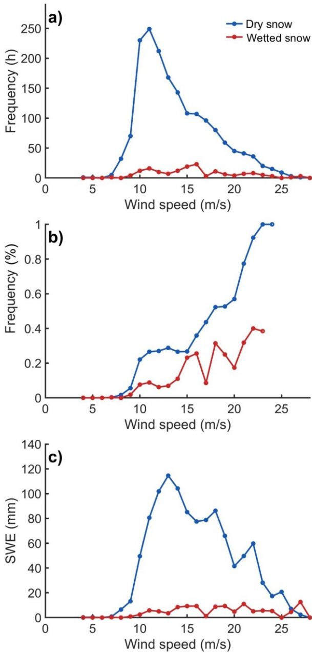
Figure 9: (a) Frequency (hours) of wind speed during modelled erosion for dry snow and wetted snow; (b) relative frequency of wind speed during modelled erosion for dry snow and wetted snow (hours with erosion divided by all hours at that wind speed and at the same time dry or wetted snow at the surface); (c) total SWE (mm) eroded per wind speed class for dry and wetted snow.
