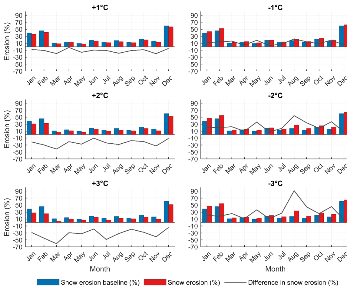
445 Figure 13: Modelled monthly snow erosion (percentage of monthly snow accumulation) for the baseline and temperature change scenarios (−3 °C to +3 °C).
