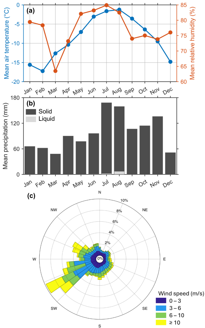
Figure 2: Monthly means of (a) air temperature and (b) precipitation in the period between September 2011 and June 2015 at the Mt. Ortles automatic weather station site (3830 m a.s.l.). The frequency distribution of wind direction and wind speed in the same period is reported in panel (c). Air temperature and wind data come directly from the automatic weather station at 3830 m a.s.l., whereas precipitation is calculated from the data recorded at the Solda village, right below Mt. Ortles, at 1907 m a.s.l.
