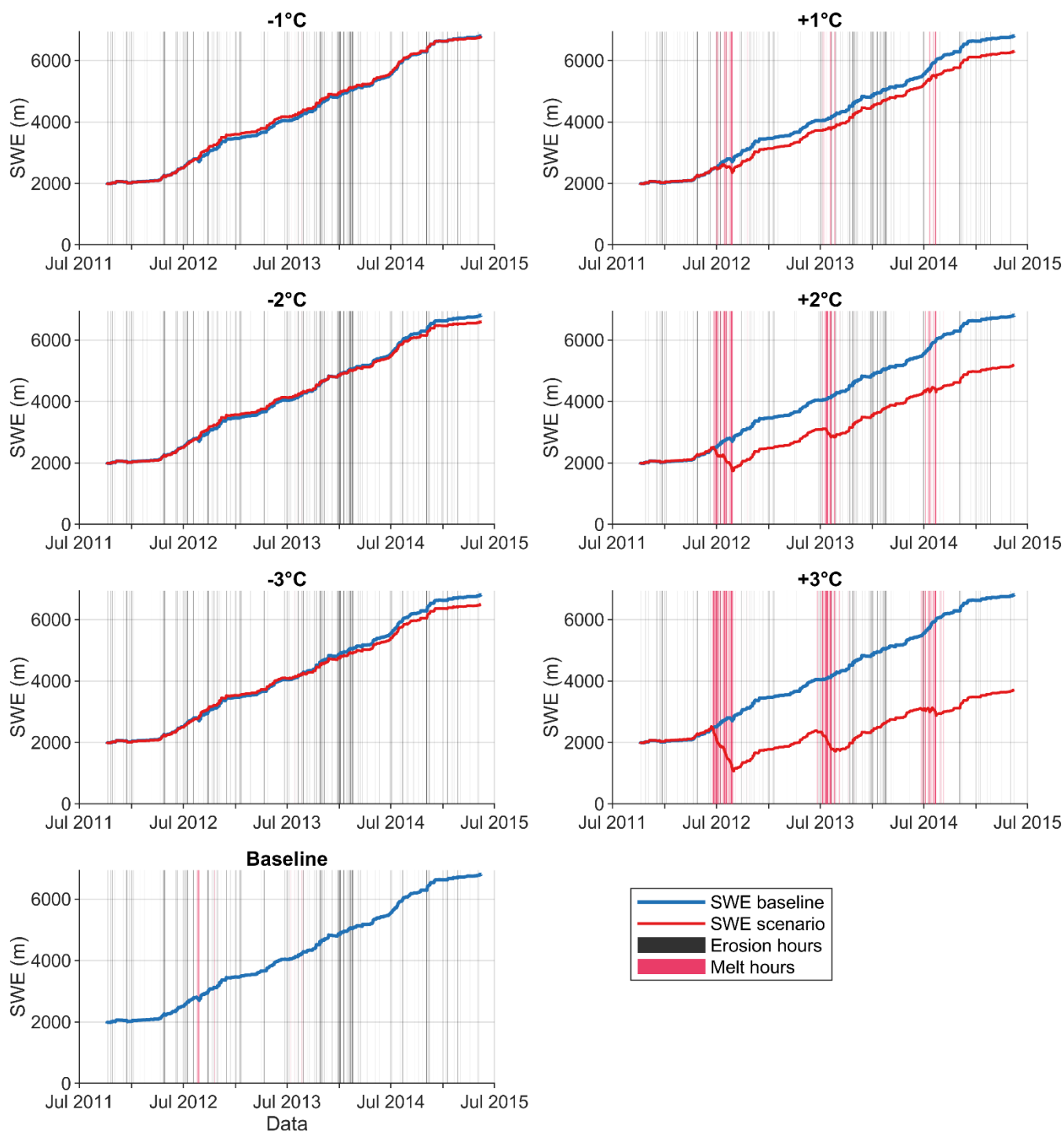
410 Figure 11: Modelled SWE at the AWS site for the baseline and temperature change scenarios (-3°C to +3°C). Vertical bars indicates melt and erosion hours.
