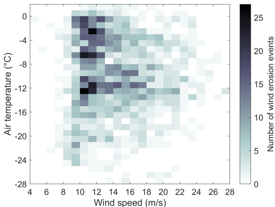
380 Figure 10: Two-dimensional scatterplot showing the frequency of wind erosion events (dry and wetted snow, color coded) for bins of air temperature and wind speed.
