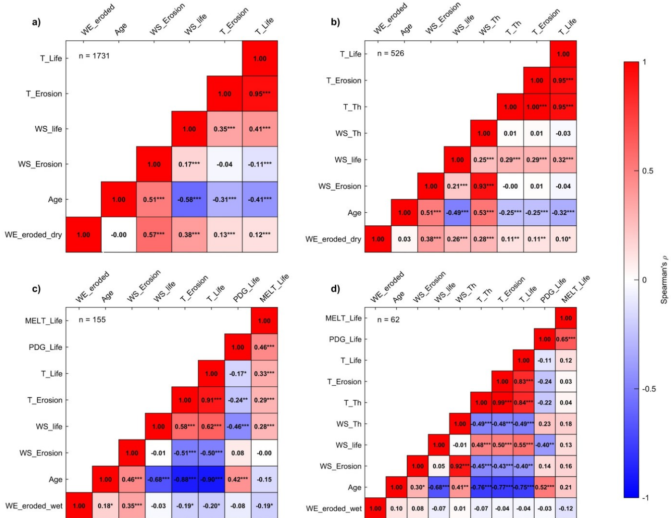
Figure 6: Spearman correlation matrix among erosion-event descriptors for (a) all dry-snow hourly erosion events, (b) dry-snow hourly erosion events, restricted to hours when erosion starts, (c) all wetted snow hourly erosion events, and (d) wetted snow hourly erosion events, restricted to hours when erosion starts. Colour encodes sign and magnitude of correlation coefficients (blue = negative, red = positive). Asterisks indicate significance (* p < 0.05 , ** p < 0.01 , *** p < 0.001 ).
