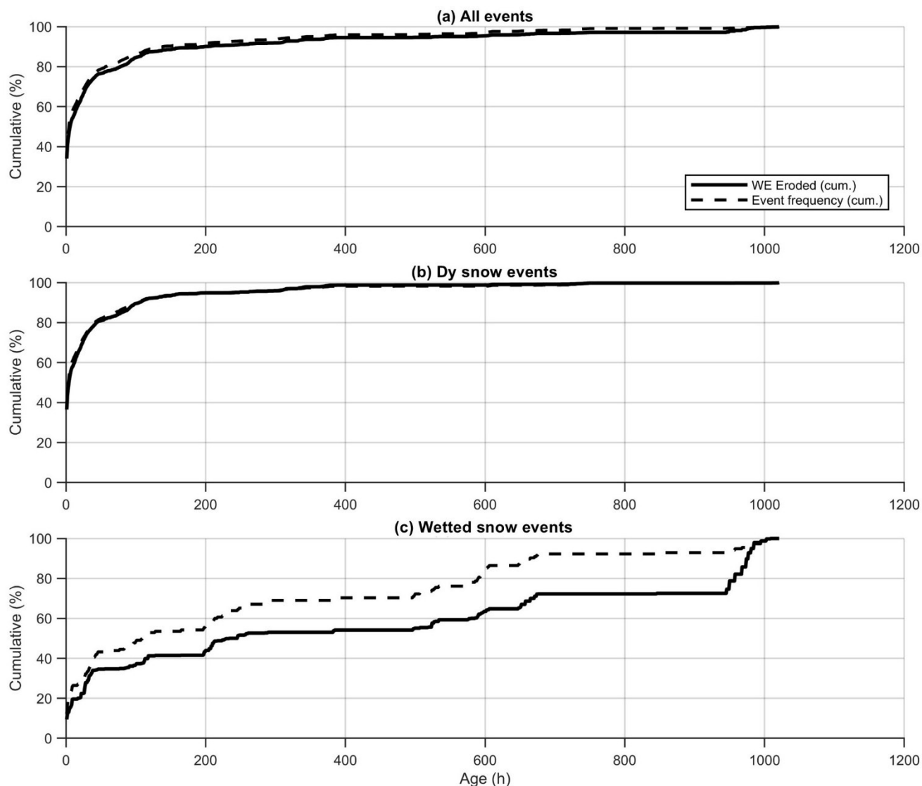
Figure 7: Cumulative relative frequency distributions and cumulative relative SWE eroded as a function of layer age. Panels show (a) all events, (b) dry snow events, and (c) wetted snow events.
