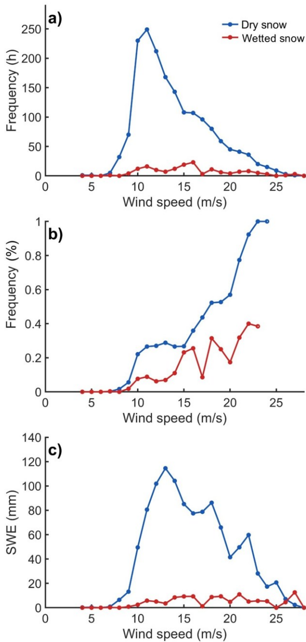
365 Figure 8: (a) Frequency (hours) of wind speed during modelled erosion for dry snow and wetted snow; (b) relative frequency of wind speed during modelled erosion for dry snow and wetted snow (hours with erosion divided by all hours at that wind speed and at the same time dry or wetted snow at the surface); (c) total SWE (mm) eroded per wind speed class for dry and wetted snow.
