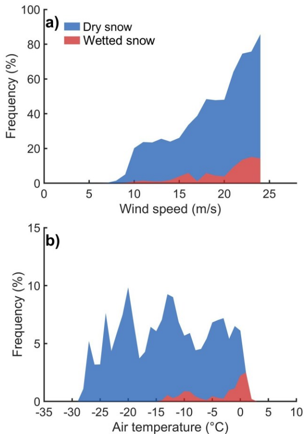
370 Figure 9: (a) Stacked area graph showing the relative frequency of occurrence of snow erosion for dry and wetted snow at various wind speeds (hours with erosion divided by all hours at that wind speed; wind speed \geq 25 \text{ m s}^{-1} is not shown because the sample size was smaller than 10 hours); (b) stacked area graph showing the relative frequency of occurrence of snow erosion for dry and wetted snow at various air temperatures (hours with erosion divided by all hours at that air temperature; air temperature bins with sample size < 10 hours are not shown).
