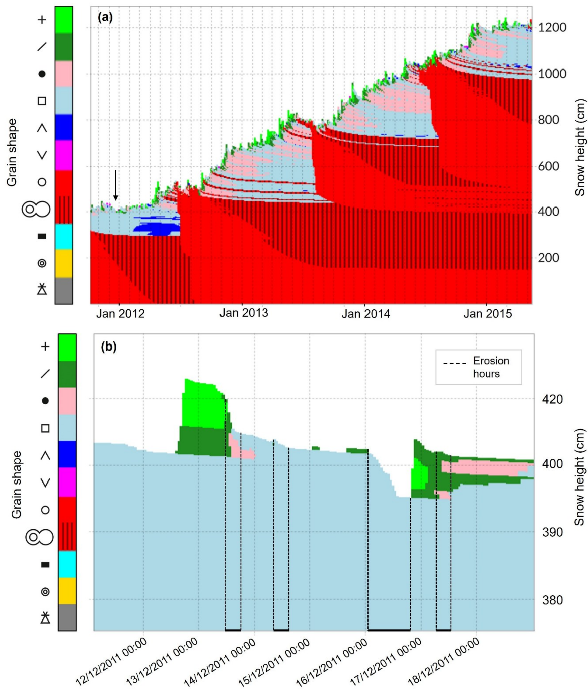
Figure 4: (a) Snow pack build up and evolution on the Mt. Ortles AWS site from 7 September 2011 to 14 of June 2015, modelled by the SNOWPACK model. Panel (b) shows a close-up of the snow erosion events between 13 and 17 December 2011, indicated by the black arrow in (a).
