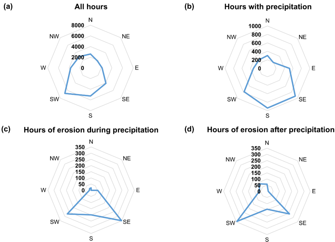
Figure 13: Frequency of wind direction for (a) all hours of observations, (b) hours with precipitation, (c) hours of erosion during precipitation, and (d) hours of erosion after precipitation.
