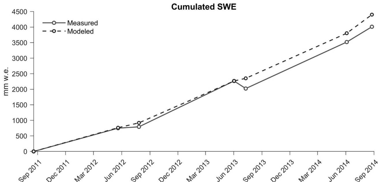
Figure 55: Comparison between modelled and measured snow water equivalent (SWE) at the Mt. Ortles AWS site.
