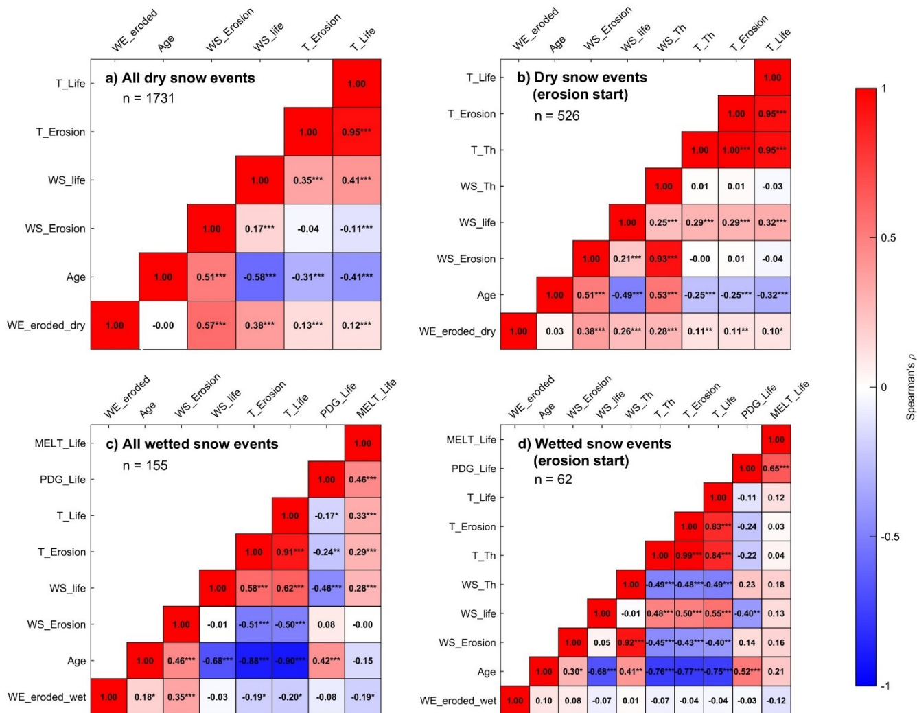
Figure 67: Spearman correlation matrix among erosion-event descriptors for (a) all dry-snow hourly erosion events, (b) dry-snow hourly erosion events, restricted to hours when erosion starts, (c) all wetted snow hourly erosion events, and (d) wetted snow hourly erosion events, restricted to hours when erosion starts. Colour encodes sign and magnitude of correlation coefficients (blue = negative, red = positive). Asterisks indicate significance (* p < 0.05 , ** p < 0.01 , *** p < 0.001 ).
