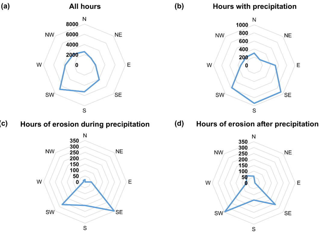
Figure 43: Frequency of wind direction for (a) all hours of observations, (b) hours with precipitation, (c) hours of erosion during precipitation, and (d) hours of erosion after precipitation.
