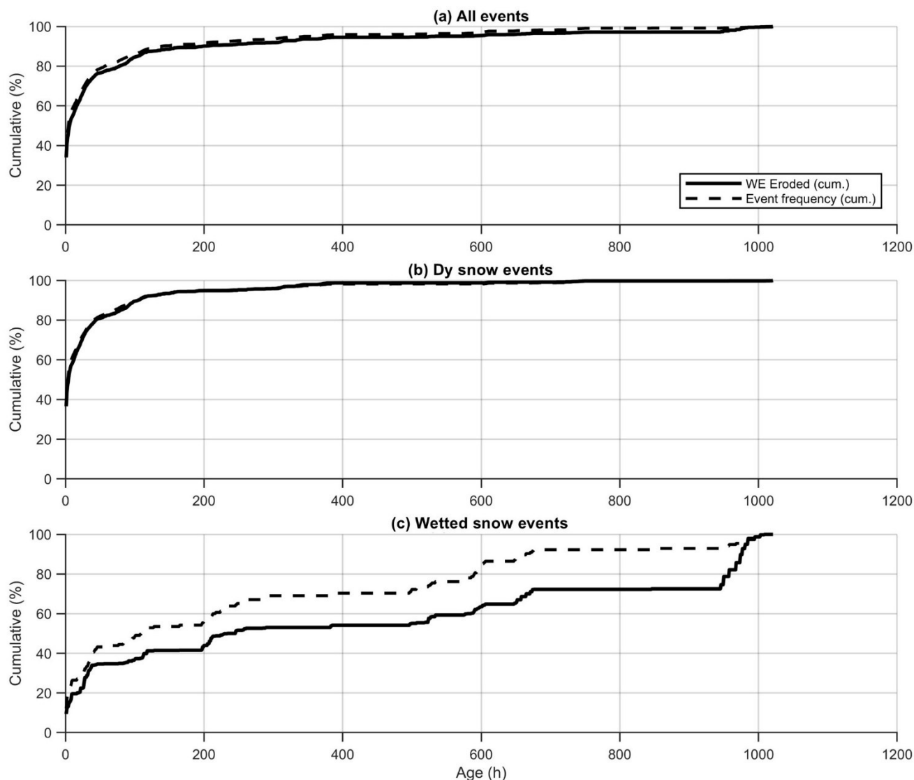
Figure 78: Cumulative relative frequency distributions and cumulative relative SWE eroded as a function of layer age. Panels show (a) all events, (b) dry snow events, and (c) wetted snow events.
