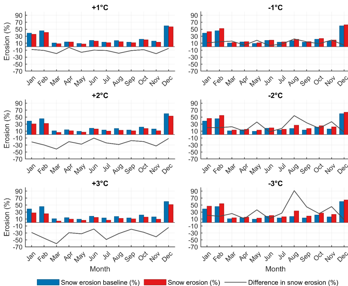
Figure 1213: Modelled monthly snow erosion (percentage of monthly snow accumulation) for the baseline and temperature change scenarios ( -3^{\circ}\text{C} to +3^{\circ}\text{C} ).
