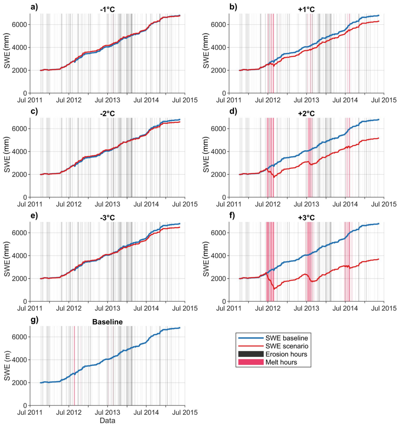
450 Figure 4-12: Modelled SWE at the AWS site for the baseline and temperature change scenarios (-3°C to +3°C). Vertical bars indicates melt and erosion hours.
