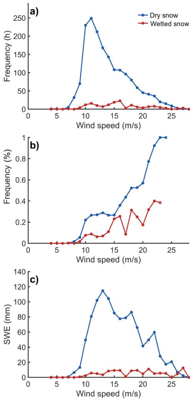
405 Figure 89: (a) Frequency (hours) of wind speed during modelled erosion for dry snow and wetted snow; (b) relative frequency of wind speed during modelled erosion for dry snow and wetted snow (hours with erosion divided by all hours at that wind speed and at the same time dry or wetted snow at the surface); (c) total SWE (mm) eroded per wind speed class for dry and wetted snow.
