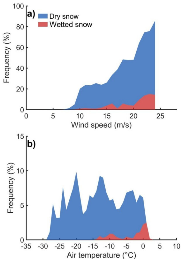
Figure 89: (a) Stacked area graph showing the R relative frequency of occurrence of snow erosion for dry and wet ted snow at various wind speeds (hours with erosion divided by all hours at that wind speed; wind speed \geq 25 \text{ m s}^{-1} is not shown because the sample size is was smaller than 10 hours); (b) stacked area graph showing the relative frequency of occurrence of snow erosion for dry and wet snow at various air temperatures (hours with erosion divided by all hours at that air temperature; air temperature bins with sample size < 10 hours are not shown).
