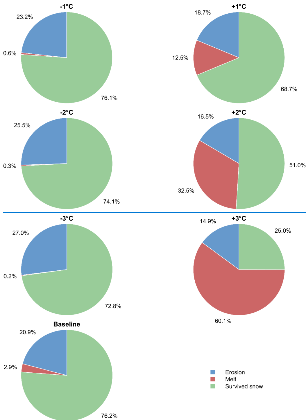
Figure 11: Modelled partitioning of total precipitation into net accumulation (survived snow), wind-driven erosion, and melt for baseline and temperature change scenarios ( -3^{\circ}\text{C} to +3^{\circ}\text{C} ). Percentages (%) refer to the total accumulated snowfall.
