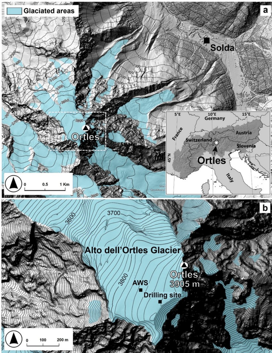
Figure 1: Location of the ice core drilling site and the automatic weather station (AWS) on Mt. Ortles. The background hill-shaded DEM (2017 lidar survey) and 2017 glaciers' outlines is are from https://mapview.civis.bz.it (last access: 15 September 2025) (Agenzia per la Protezione civile, Autonomous Province of Bolzano).
