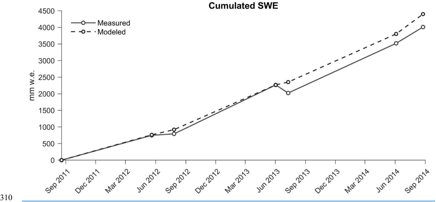
Figure 5: Comparison between modelled and measured snow water equivalent (SWE) at the Mt. Ortles AWS site.
