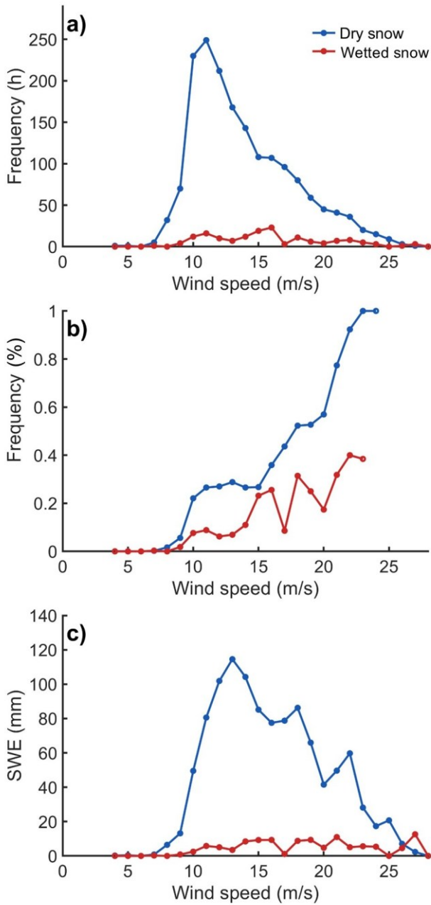
Figure 78: (a) Frequency (hours) of wind speed during modelled erosion for dry snow and wetted snow; (b) relative frequency of wind speed during modelled erosion for dry snow and wetted snow (hours with erosion divided by all hours at that wind speed and at the same time dry or wetted snow at the surface); (c) total SWE (mm) eroded per wind speed class for dry and wetted snow.
