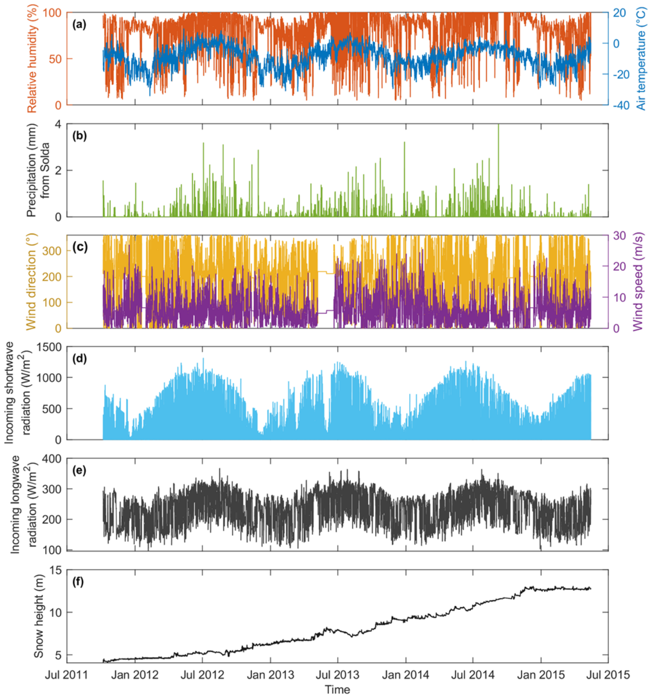
Figure 3: Hourly values of nivo-meteorological data recorded by the Ortles AWS (3830 m a.s.l.) from September 2011 to June 2015: (a) air temperature and relative humidity, (b) precipitation, (c) wind speed and direction, (d) incoming shortwave radiation, (e) incoming longwave radiation, (f) snow height. Please note that precipitation data were not measured at the same AWS, but come from the nearby village of Solda (1907 m a.s.l.).
