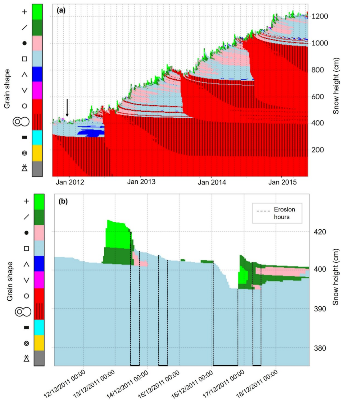
Figure 4: (a) Snow pack build up and evolution on the Mt. Orles AWS site from 7 September 2011 to 14 of June 2015, modelled by the SNOWPACK model. Panel (b) shows a close-up of the snow erosion events between 13 and 17 December 2011, indicated by the black arrow in (a).
