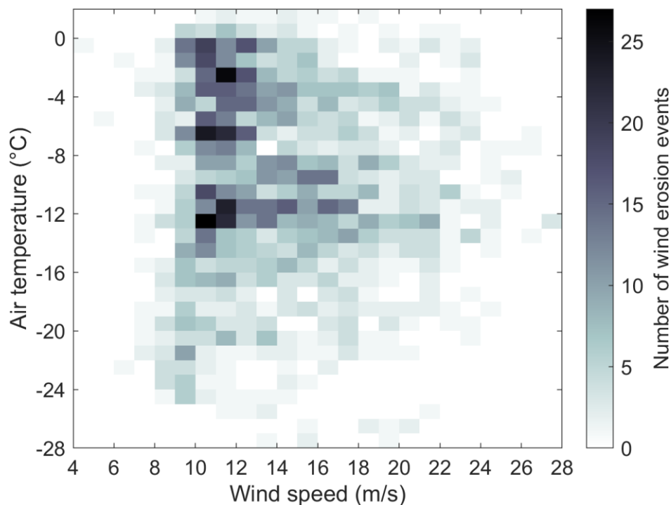
425 Figure 910: Frequency distributions of the threshold wind speed for erosion for dry and wet snow eventsTwo-dimensional scatterplot showing the frequency of wind erosion events (dry and wetted snow, color coded) for bins of air temperature and wind speed.
