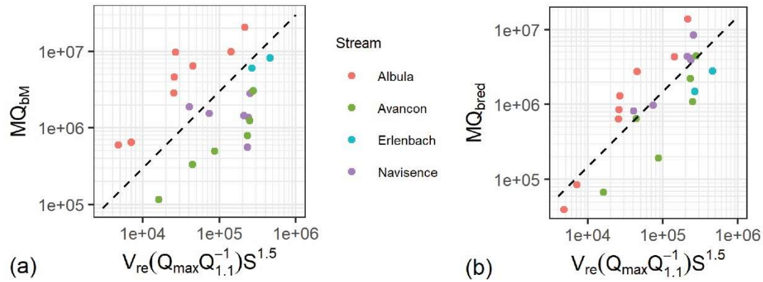
Figure 12. Yearly bedload masses vs. a simple measure of flow strength, as V_{\text{re}}(Q_{\text{max}}/Q_{1.1})S^{1.5} . (a) for the measured yearly bedload mass, \text{sum}(Q_{\text{bm}}) , and (b) for the calculated yearly bedload mass using eq. (9), \text{sum}(Q_{\text{bred}}) . The dashed black lines indicate a linear relation, the position of which was chosen to approximately fit the trend defined by the data of the four streams.
