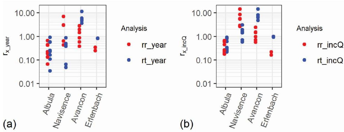
Figure 7. Variability of (a) r_{x\_year} and (b) r_{x\_incQ} , separately for the analysis with the Q_{tot} calculations ( x=t ) and for the Q_{bred} calculations ( x=r )
