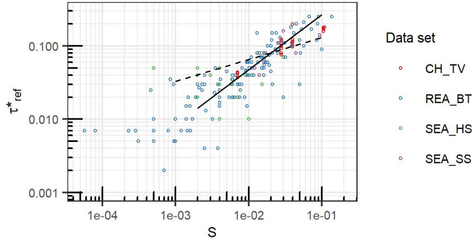
Figure 9. Optimized values of \tau_{\text{ref}}^* vs. channel slope S , for various datasets. For the CH-TV, SEA_SS and SEA_HS data, \tau_{\text{ref}}^* was determined based on a W_{\text{tot}}^* analysis. For the REA_BT data, \tau_{\text{ref}}^* was derived from the Recking equation assuming a fixed exponent \beta=4 (case 1 analysis). The solid black line is eq. (33) derived from the REA_BT data with a plane-bed morphology. The dashed black line is eq. (32) from Recking et al. (2016) based on flume experiments and used in their case-2 analysis.
