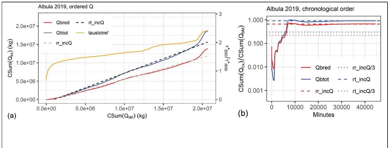
Figure C1. Albula, summer 2019. Example of a good agreement of a linear model (dashed black and gray lines) for the cumulative sum of calculated ( Csum(Q_{bx}) ) vs. measured ( Csum(Q_{bm}) ) bedload masses. In (a) the values were ordered according to increasing discharge Q , and the increase in relative flow intensity is shown with the ratio \tau_{D50}^*/\tau_{RD50}^* (taustotref). In (b) the values are summed up in chronological order.
