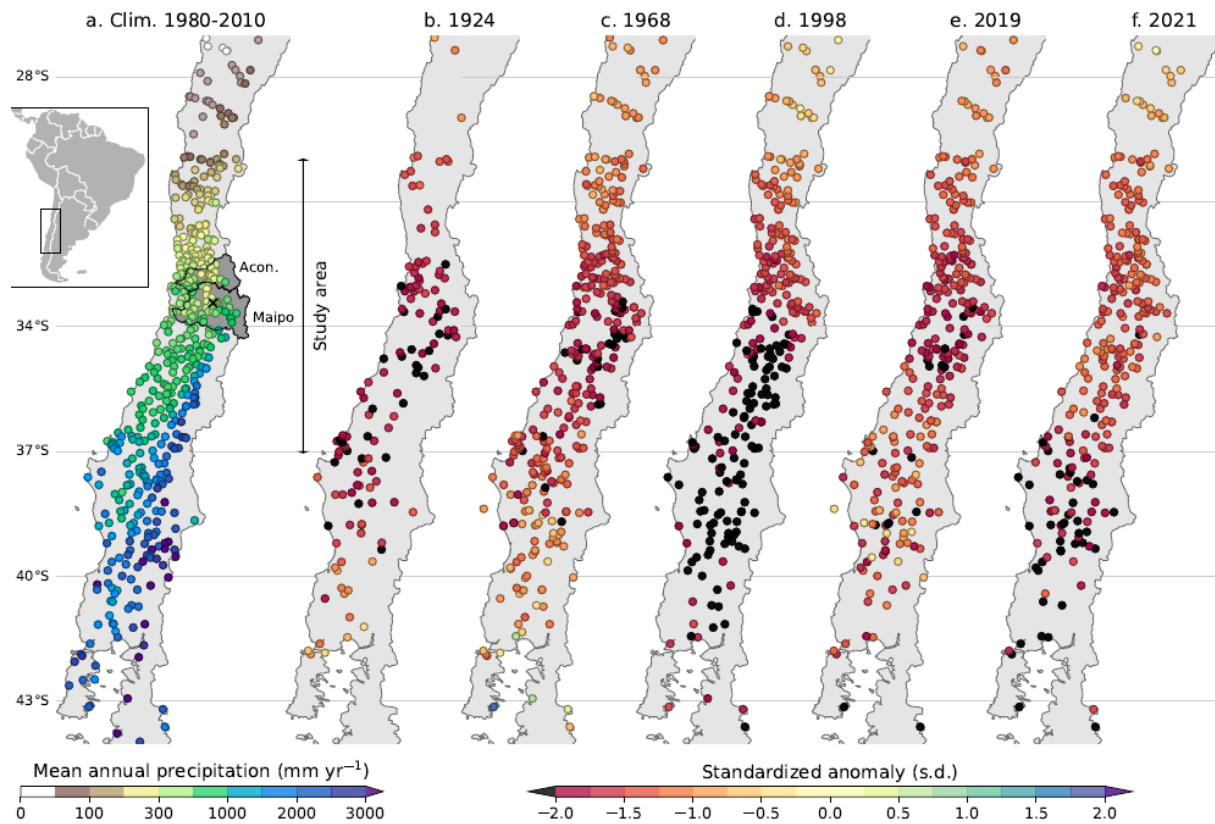
70 Figure 1. Panel (a) shows the climatological annual mean precipitation in stations along Chile. The study area and the outlines of the Aconcagua and Maipo basins are also indicated. The rest of the panels (b-f) show the standardized precipitation anomalies during the HD years of 1924, 1968, 1998, 2019, and 2021.
