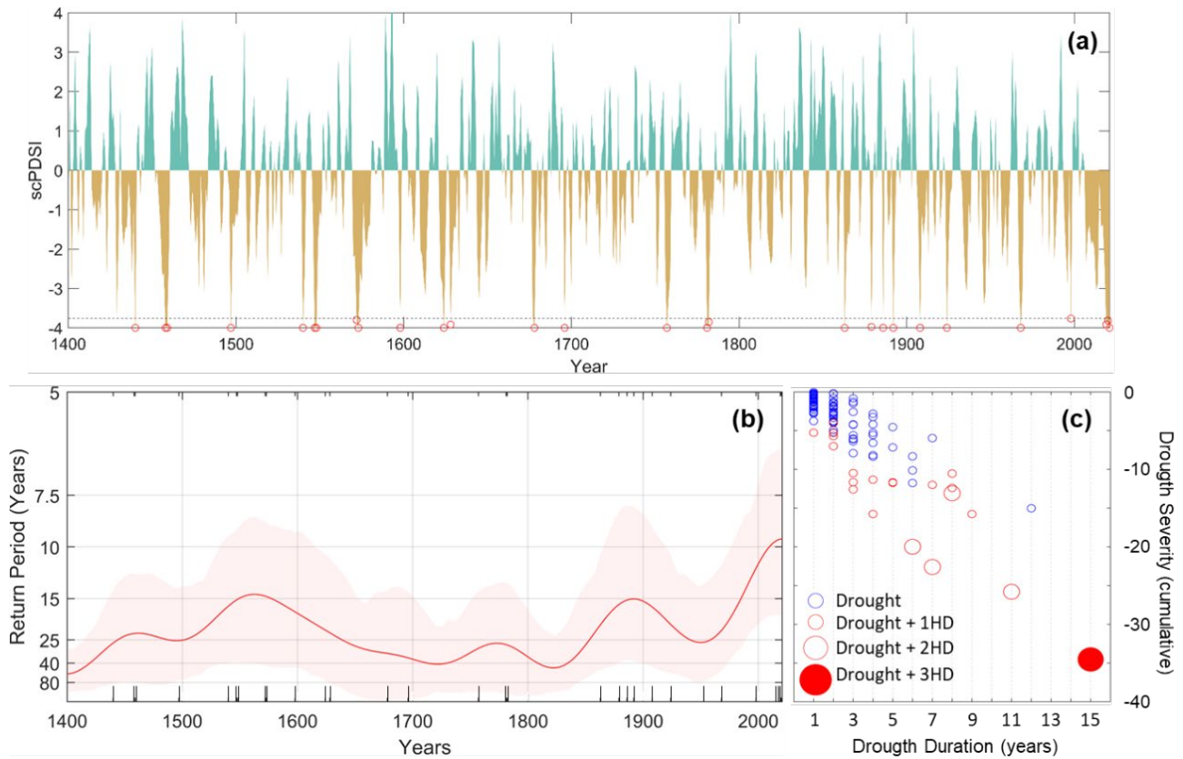
Figure 3. (a) Central Chile scPDSI reconstruction. The red dots at the bottom indicate the reconstructed hyperdroughts (RHD) according to the scPDSI threshold (see section 2.5). (b) The time-varying frequency of RHD events between 1400 and 2021 is indicated with ticks at the x-axis. The shaded pink area represents 95% confidence intervals based on 1,000 bootstrap simulations. (c) Severity-duration analysis of RHD and droughts events during the 1400-2021 period. Circles indicate individual drought events of the duration indicated by the x-axis and a cumulative severity shown on the left y-axis. The left and bottom histograms show the distribution of cumulative severity and duration, respectively. The blue and red contour dots indicate drought periods with and without RHD events. The size of the dots indicates if a given drought contains one, two, or three HD events. The solid red dot coincides with the recent megadrought period 2007-2021.
