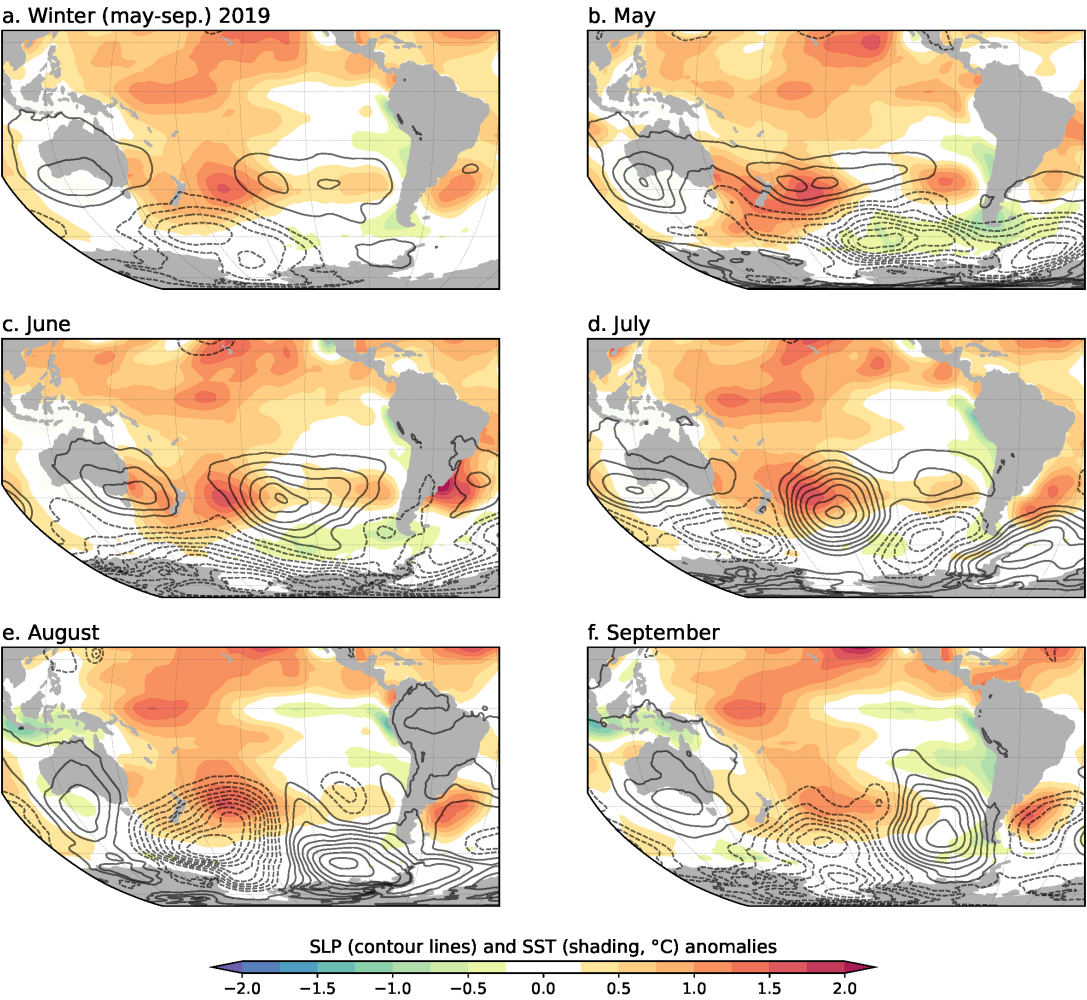
355 Figure 6. (a) Sea surface temperature (SST) and sea level pressure (SLP) anomalies for the extended winter (May-September) of 2019. Panels (b-f) indicate the individual monthly mean SST and SLP anomalies of that winter. Positive and negative SLP anomalies are shown by solid and dashed contour lines, respectively, draw every 1.5 hPa.
