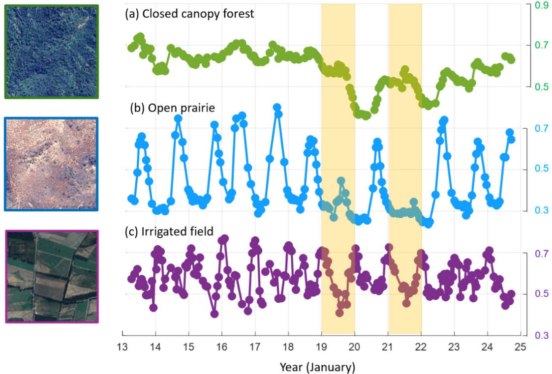
480 Figure 11. 16-day Landsat 8 surface reflectance over three sites in north-central Chile from January 2013 to September 2024. In all | cases, we averaged the original pixel (30 m resolution) within 90-150 \times 90-150 m 2 sites characterized by (a) close-canopy forest (centered at 32.99°S, 71.09°W), (b) open prairie (centered at 33.00°S, 71.15°W), and (c) irrigated field (centered at 32.80°S, 70.86°W).
