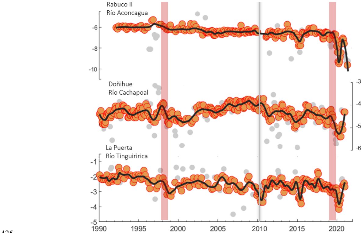
Figure 8. Groundwater levels (relative to ground surface) at three wells in central Chile: Rabuco (Aconcagua basin), Doñihue (Cachapoal basin), and La Puerta (Tingururica basin). The three wells are located in the central valley, at about 300 m ASL. The observations (circles) are taken by DGA every 1 or 2 months. The black solid line is the LOESS filter, which uses a 5% span of the total data points. Outliers are drawn in light grey. The hyperdrought of 1998 and 2019 are highlighted by the pink vertical bands. The grey vertical line indicates the beginning of the central Chile megadrought
