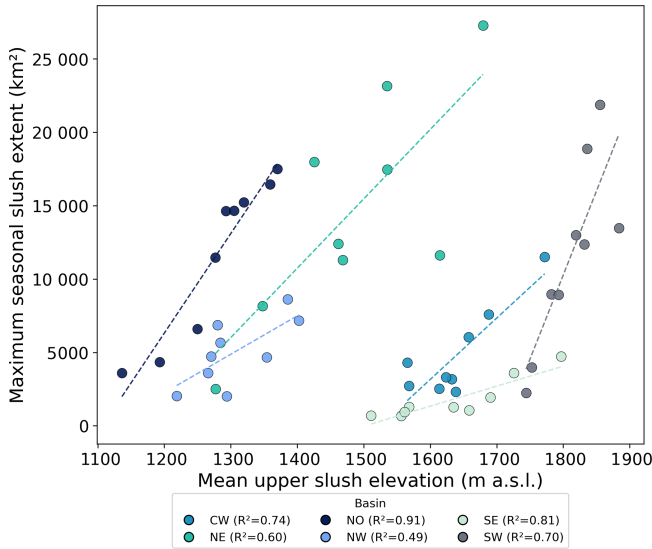
Figure 7. Relationship between mean upper slush-limit elevation and maximum seasonal slush extent by basin (2016–2024). Coloured points show seasonal values, and dashed lines show ordinary least-squares regressions fitted separately for each basin. Reported R^2 and p -values refer to these regressions; all relationships are statistically significant ( p < 0.05 ).
