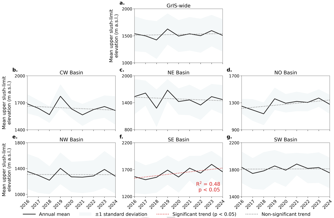
Figure 5. Inter-annual variability in mean upper slush-limit elevation across the GrIS from 2016 to 2024. Panel (a) shows ice-sheet-wide values, while panels (b)–(g) show values for the CW, NE, NO, NW, SE, and SW basins, respectively. Black lines show annual mean upper slush-limit elevation, and shading represents \pm 1 standard deviation of elevation measurements sampled along the mapped upper slush limit. Dotted lines show fitted linear temporal trends; statistically significant trends ( p < 0.05 ) are shown in red and non-significant trends in grey. Note that y-axis ranges differ among panels.
