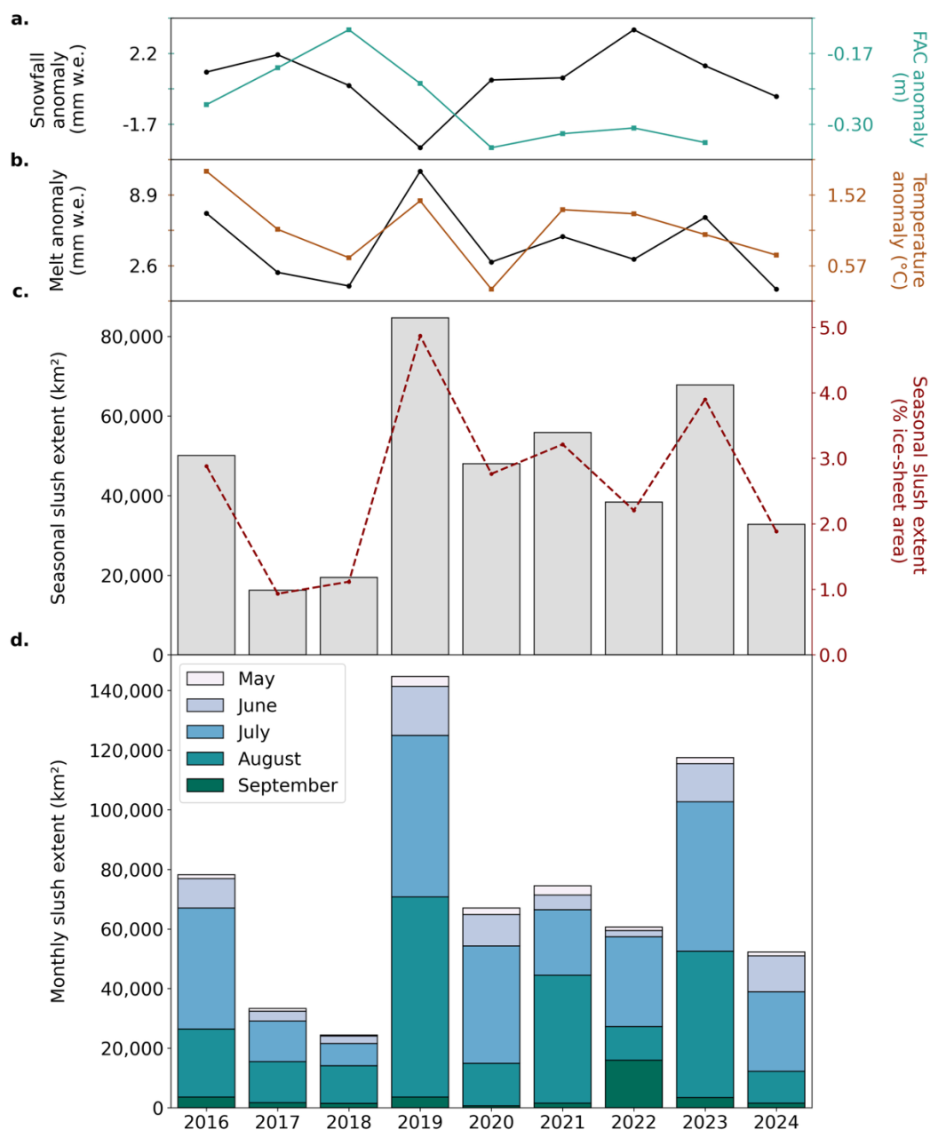
70 Figure 4: Mean annual climate and slush variability across the GrIS from 2016–2024. (a) Ice-sheet-wide mean snowfall 71 anomalies and FAC anomalies (teal) relative to the 1960–1989 mean. (b) Ice-sheet-wide mean snowmelt anomalies 72 (black) and 2 m air temperature anomalies (orange) relative to the 1960–1989 mean. (c) Seasonal slush extent for May– 73 September, shown as absolute area (left y-axis, grey bars) and as a percentage of total ice-sheet area (right y-axis; 74 dashed dark-red line). (d) Stacked monthly slush extent for May–September in each year (note: monthly segments are 75 not spatially additive). Snowfall, snowmelt, and 2 m air temperature are derived from RACMO, while FAC is derived 76 from the IMAU-FDM (available through 2023 only).
