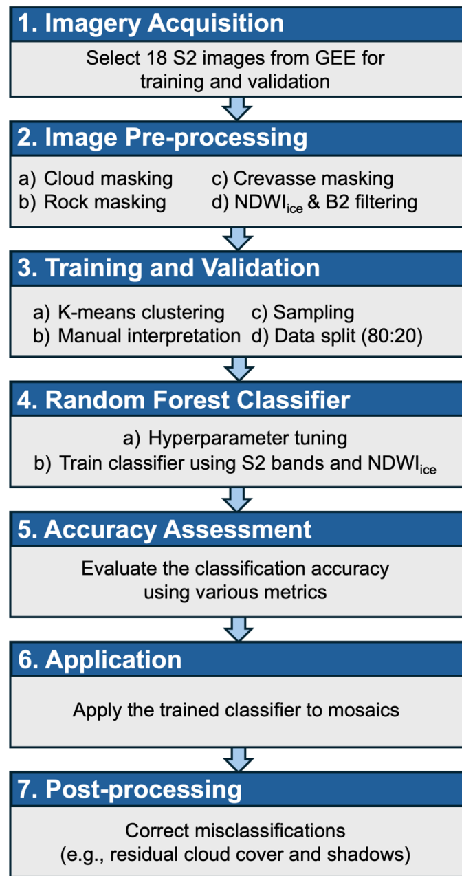
15 Figure 1: Flowchart of the slush-classification methodology adapted from Dell et al. (2022a, 2024), originally developed 16 for Antarctic ice shelves, for application to the GrIS in this study.
