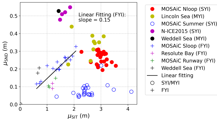
Figure 6. The relationship between the snow depth (SND) and sea ice thickness (SIT), where \mu_{SND} and \mu_{SIT} denote the mean SND and mean SIT values of each transect, respectively. The color and symbol ("o" and "+") represent different test sites and ice types, respectively.
