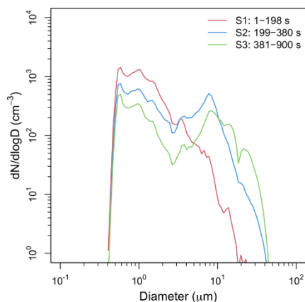
455 Figure 6. Size-resolved number concentrations for the experiments conducted using (a, b) NaCl and (c, d) CaCl 2 . S1 represents the under-saturated stage ( RH \leq 85\% , red line), S2 the pre-saturated stage ( 85\% < RH \leq 100\% , blue line), and S3 the supersaturated stage ( RH > 100\% , green line) with respect to the elapsed time.
