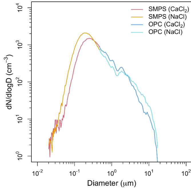
300 Figure 2. Distribution of size-resolved number concentration of NaCl and CaCl 2 powders based on the scanning mobility particle size (SMPS) and optical particle counter (OPC) observations.
