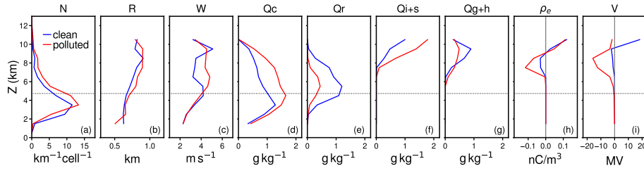
Figure 7. Vertical profiles of mean thermal properties: (a) thermal number density, (b) median thermal radius, (c) ascent rate, (d) cloud water mixing ratio, (e) rain water mixing ratio, (f) ice+snow mixing ratio, (g) graupel+hail mixing ratio, (h) volume charge density, and (i) electric potential. Dotted line indicates the 0°C level. Median values in (b)-(i) are only shown where the number of thermals is at least 0.5% of the total sample size (6996 time steps for clean cases and 3126 for polluted cases).
