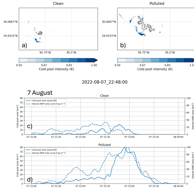
Figure 19. Instantaneous spatial distribution of cold pool intensity (blue shade) and intense rain-water path (RWP > 10 kg/m2) in the subdomain of Fig. 17 from a) the clean case and b) the polluted case at 22:48Z on 7 August case. Time series of cold pool area and intense RWP area from c) the clean case and d) the polluted case in the same subdomain.
