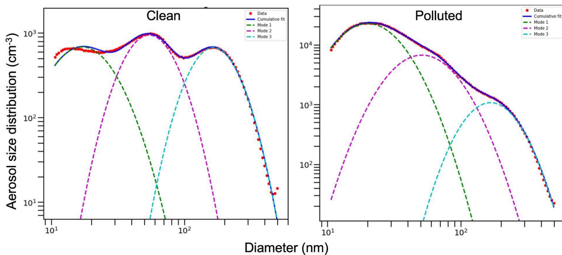
Figure R1-0 (same as Fig. S1 in supplementary material): Multimodal aerosol size distributions at the TRACER main site for clean ( <10\text{th} percentile) and polluted ( >90\text{th} percentile) conditions during 17 June to 07 August 2022. Red markers represent observations from scanning mobility particle sizer (SMPS) measurements, the blue line shows the cumulative lognormal fit, and dashed lines indicate the three fitted modes.
