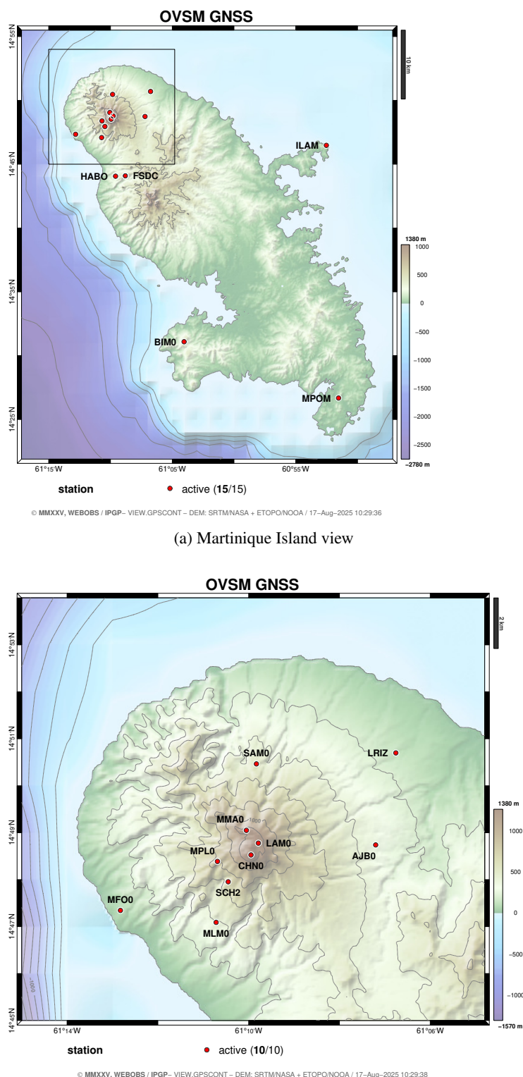
Figure 2. Map of the MQ GNSS Network, managed by the OVSM at Martinique island. For the sake of readability, the first four characters only of the station codes are represented.
