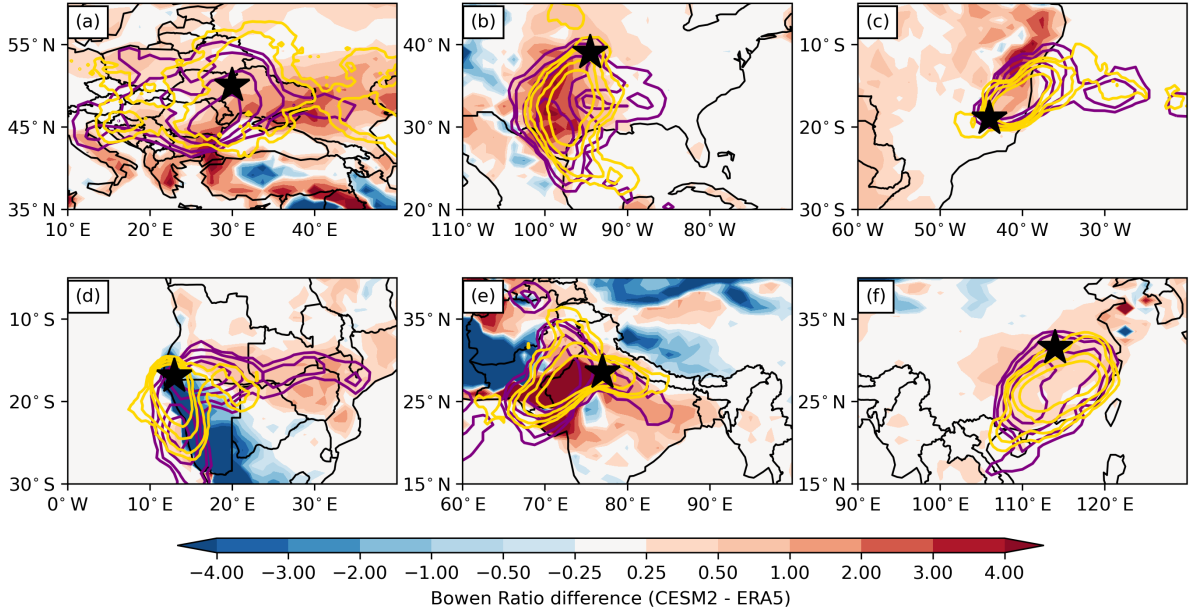
Figure 10. As Fig. ?? but Shading depict differences in the mean Bowen ratio averaged for all TX1day events at the location indicated with the black star. Red colors (i.e., larger Bowen ratios in CESM2 compared to ERA5) indicate a heat flux partitioning with more dominant sensible and attenuated latent heat fluxes during TX1day events in CESM2. Purple and yellow contours depict genesis densities of TX1day anomalies in CESM2 and ERA5, respectively, in the same units as in Fig. 6. Black stars denote the locations of (a) Kyiv, Ukraine, (b) Kansas City, United States, (c) Belo Horizonte, Brazil, (d) the Epupa Falls, at the border between Namibia and Angola, (e) Delhi, India, and (f) Wuhan, China.
