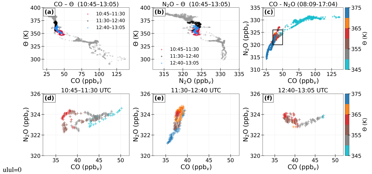
Figure 3. Vertical profiles of (a) CO (in ppbv) and (b) N 2 O (in ppbv) with grey circles showing data of the entire flight and color-coded markers indicating the time from 10:45–13:05 UTC. (c-f) Tracer-tracer correlation of the mixing ratios of N 2 O and CO for (c) the entire flight and for time periods between (d) 10:45–11:30 UTC, (e) 11:30–12:40 UTC and (f) 12:40–13:05 UTC, color-coded with potential temperature.
