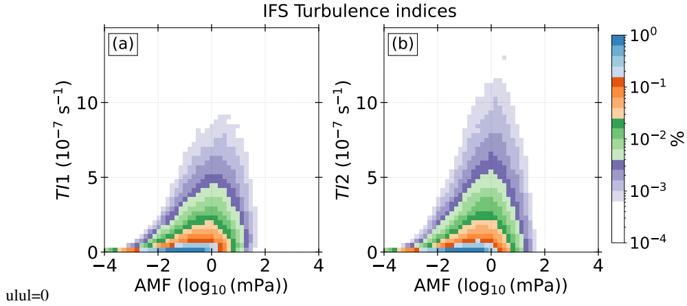
Figure 13. Frequency (%) distribution of absolute momentum flux-turbulent indices TI1 (a), TI2 (b) in pairs over the LMS for IFS data. Normalized counts of PDF distribution is shown. Logarithmic occurrence frequency color scale is applied.
