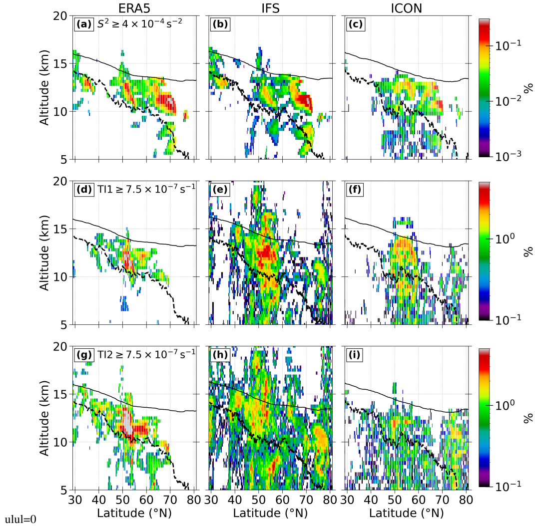
Figure 19. Relative occurrence frequency distribution of grid volumes that exhibit (a-c) S^2 \geq 4 \times 10^{-4} \text{ s}^{-2} , (d-f) \text{TI1} \geq 7.5 \times 10^{-7} \text{ s}^{-1} and (g-i) \text{TI2} \geq 7.5 \times 10^{-7} \text{ s}^{-1} over the North Atlantic domain on 23rd September 2017, 11:00 UTC for ERA5, IFS, and ICON. Panels (di) represent regions of moderate-intensity CAT occurrence. The occurrence frequencies are shown with logarithmic frequency contours, displaying the data in bins of sizes \Delta y = 0.2 and \Delta z = 500 \text{ m} . The zonal-mean dynamical tropopause (3.5 PVU isosurface; black dashed line) and the zonal-mean 380 K isentrope of potential temperature (solid line) are overlaid.
