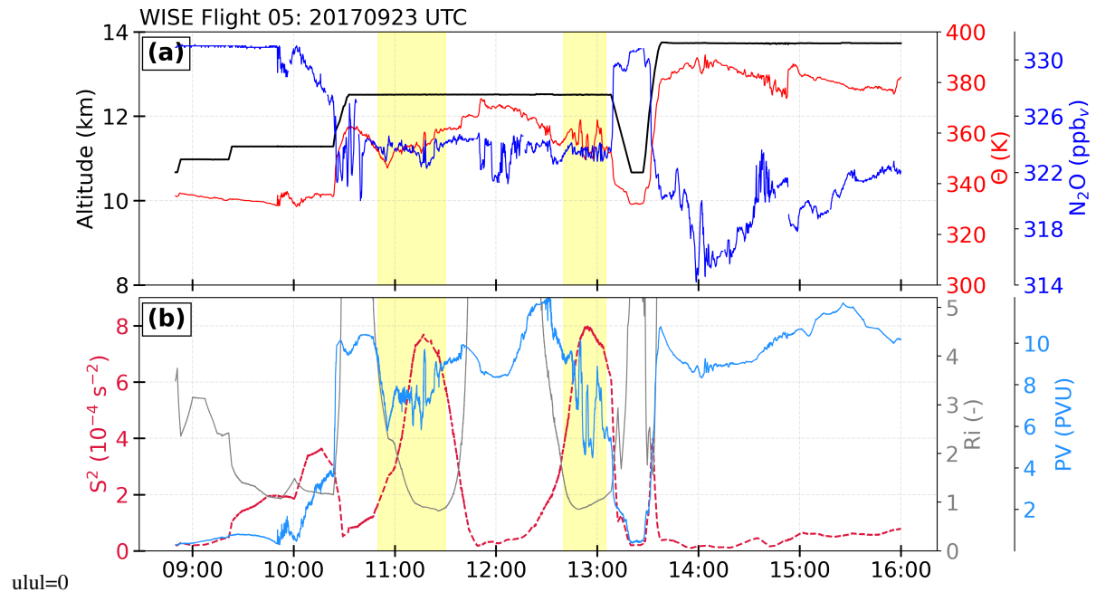
Figure 2. Time series of (a) observed flight altitude (in km, black), potential temperature (in K, red), and nitrous oxide (in ppbv, blue) as well as (b) ERA5 derived quantities along the flight path such as vertical shear (in 10^{-4} \text{ s}^{-2} , red), Richardson number (dimensionless, grey), and potential vorticity (in PVU, cyan). The light yellow bars and the white bar in between indicate the flight section of the consecutive detailed analysis of mixed air masses.
