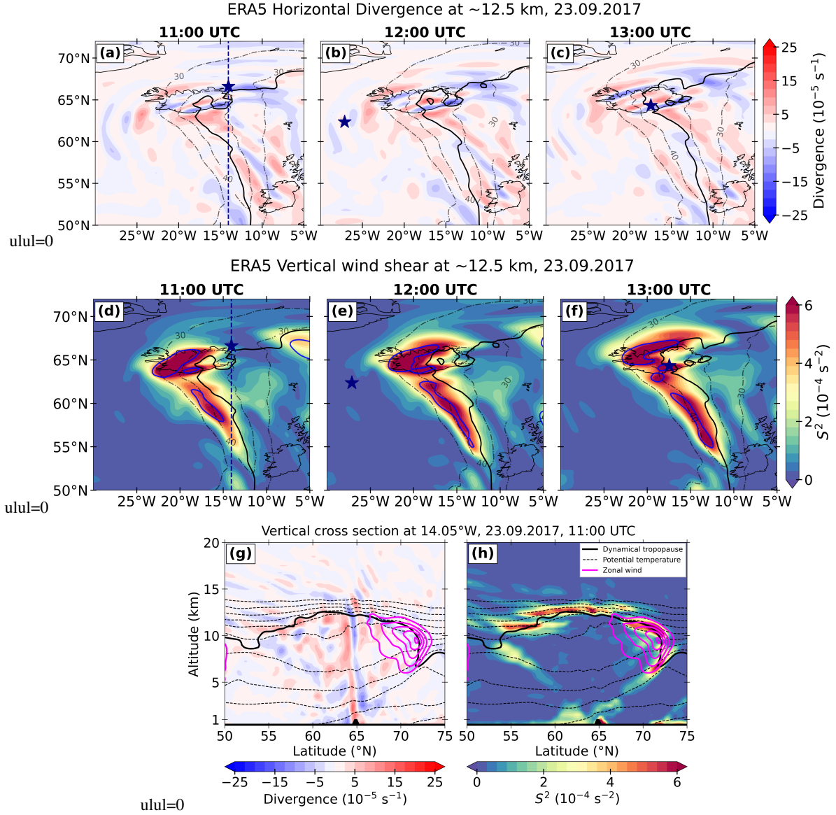
Figure 6. Distribution of horizontal divergence (upper panel) and vertical wind shear (middle panel) at \sim 12.5 km altitude for ERA5 reanalysis data at 11:00 UTC (a, d), 12:00 UTC (b, e) and 13:00 UTC (c, f). The dashed lines in upper and middle panels represent corresponding horizontal wind speed for values greater than 30 \text{ m s}^{-1} . The RF05 flight location during the time is marked by blue star. The vertical cross sections of divergence (g) and shear (h) at 14.05^\circ \text{W} during 11:00 UTC is shown in lower panel. The solid black line represent the 3.5 PVU as a dynamical tropopause whereas dotted lines in lower panel represent the potential temperature starting from 280 K (bottom) to 380 K (top) with 10 K increments. Magenta contours in (g, h) denote zonal wind speed (20, 30, 40, 50) in \text{m s}^{-1} and solid blue lines in middle panel represent Ri = 1 .
