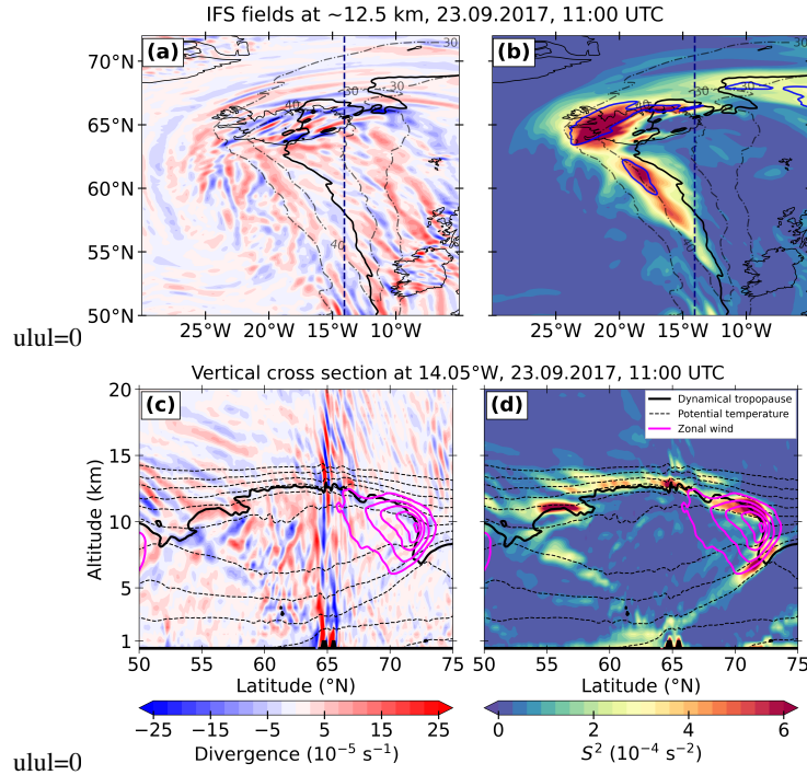
Figure 10. Distribution of horizontal divergence (a) and vertical wind shear (b) at ~12.5 km altitude for IFS data at 11:00 UTC. The dashed lines in upper and middle panels represent corresponding horizontal wind speed for values greater than 30 \text{ m s}^{-1} . The RF05 flight location during the time shown by blue star. The vertical cross sections of divergence (c) and shear (d) at 14.05^\circ \text{ W} during 11:00 UTC is shown in bottom panel. The solid black line represent the 3.5 PVU as a dynamical tropopause whereas dotted lines in lower panel represent the potential temperature starting from 280 K (bottom) to 380 K (top) with 10 K increments. Magenta contours in (g, h) denote zonal wind speed (20, 30, 40, 50) in \text{m s}^{-1} and solid blue lines in (c) represent the Ri = 1 .
