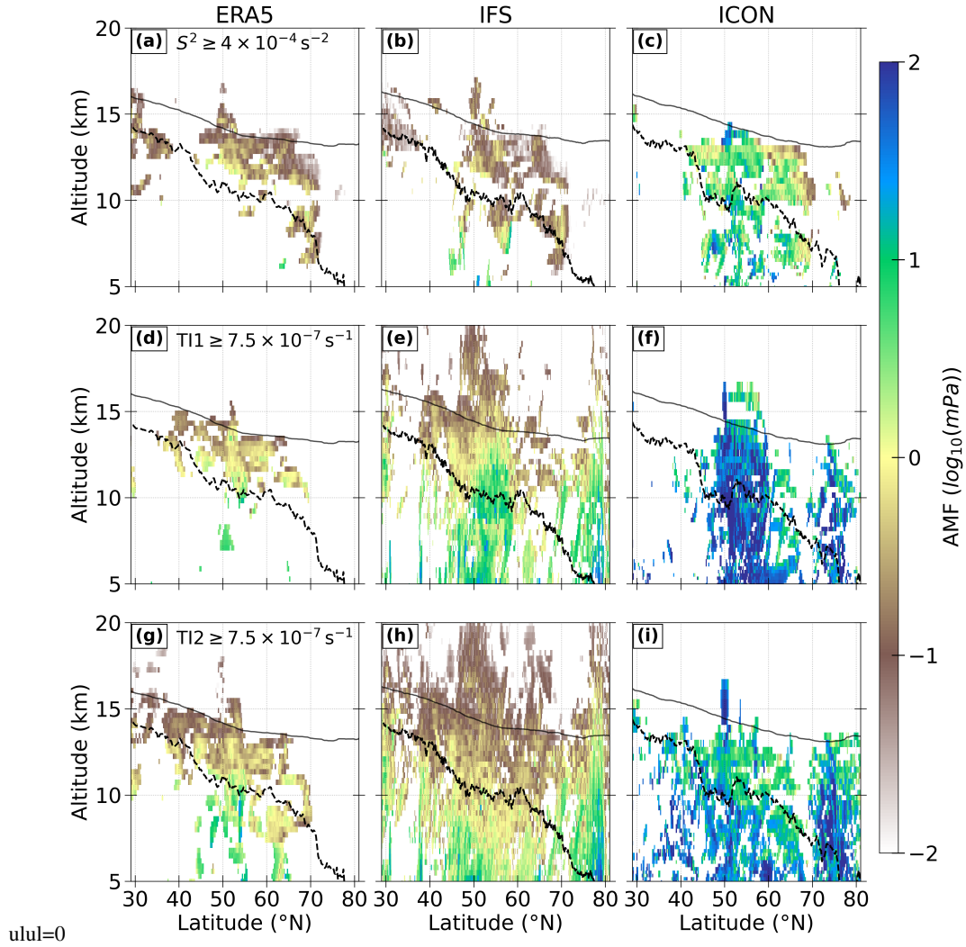
Figure 20. Zonal mean resolved GW absolute momentum flux (AMF, \log_{10}(\text{mPa}) ) values conditioned on regions where (a-c) S^2 \geq S_t^2 , (d-f) \text{TI1} \geq 7.5 \times 10^{-7} \text{ s}^{-1} and (g-i) \text{TI2} \geq 7.5 \times 10^{-7} \text{ s}^{-1} . All values are vertically binned with \Delta z = 500 \text{ m} . The zonal-mean dynamical tropopause (3.5 PVU isosurface; black dashed line) and the zonal-mean 380 K isentrope of potential temperature (solid line) are overlaid.
