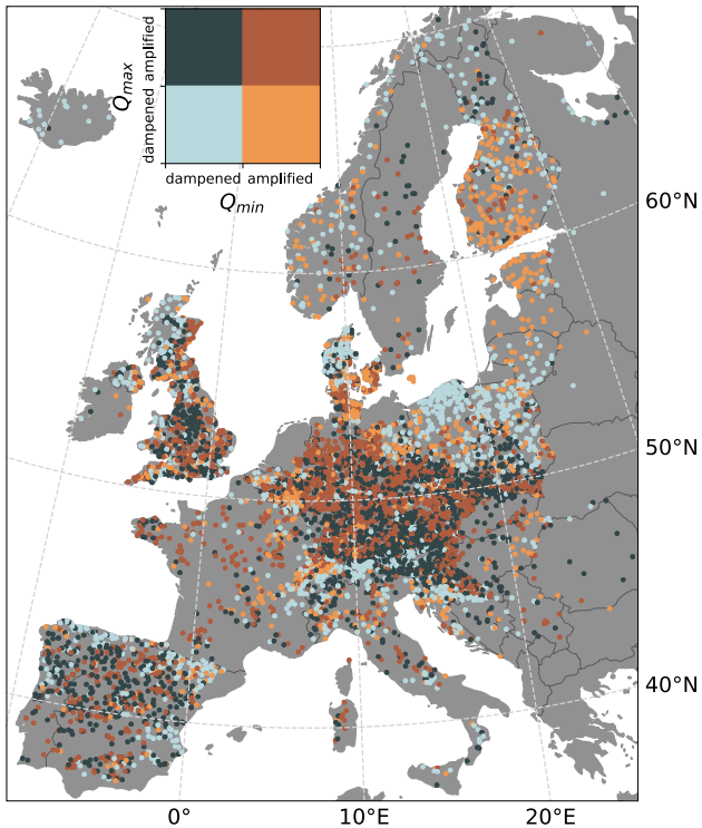
355 Figure 5: Combined elasticity of maximum and minimum flow to precipitation as a measure of resilience. The colour classes split the elasticities into whether the streamflow response is dampened/resilient ( \epsilon < 1 ), or amplified/sensitive ( \epsilon > 1 ).
