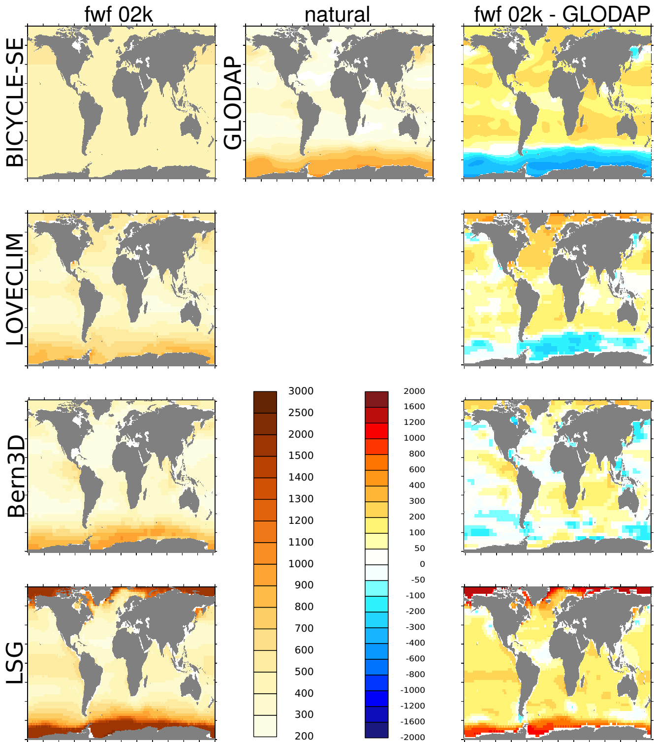
Figure 2. Surface MRA ( ^{14}\text{C} yr) from all models (left) at 2 kyr BP for runs with forced abrupt AMOC changes (scenarios: A3@BICYCLE-SE, fwf@LOVECLIM; PallSTD@Bern3D) and med@LSG; (right) differences in surface MRA from natural GLODAP (top middle). BICYCLE-SE: surface boxes; all else: mean values of roughly the top 50 m. Use left color-code (brownish) for absolute values and right color-code (blue-to-red) for differences.
