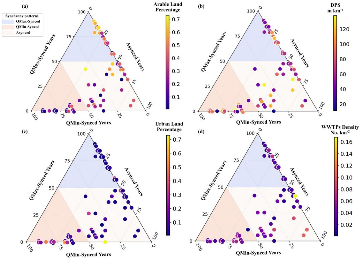
345 Figure 6: Ternary plots of percentage of synchronous years and key drivers for each catchment, coloured by (a) Arable land percentage, (b) DPS, (c) Urban land percentage, and (d) Density of WWTPs. Statistical correlations between synchrony composition and catchment descriptors are reported in Fig. S7.
