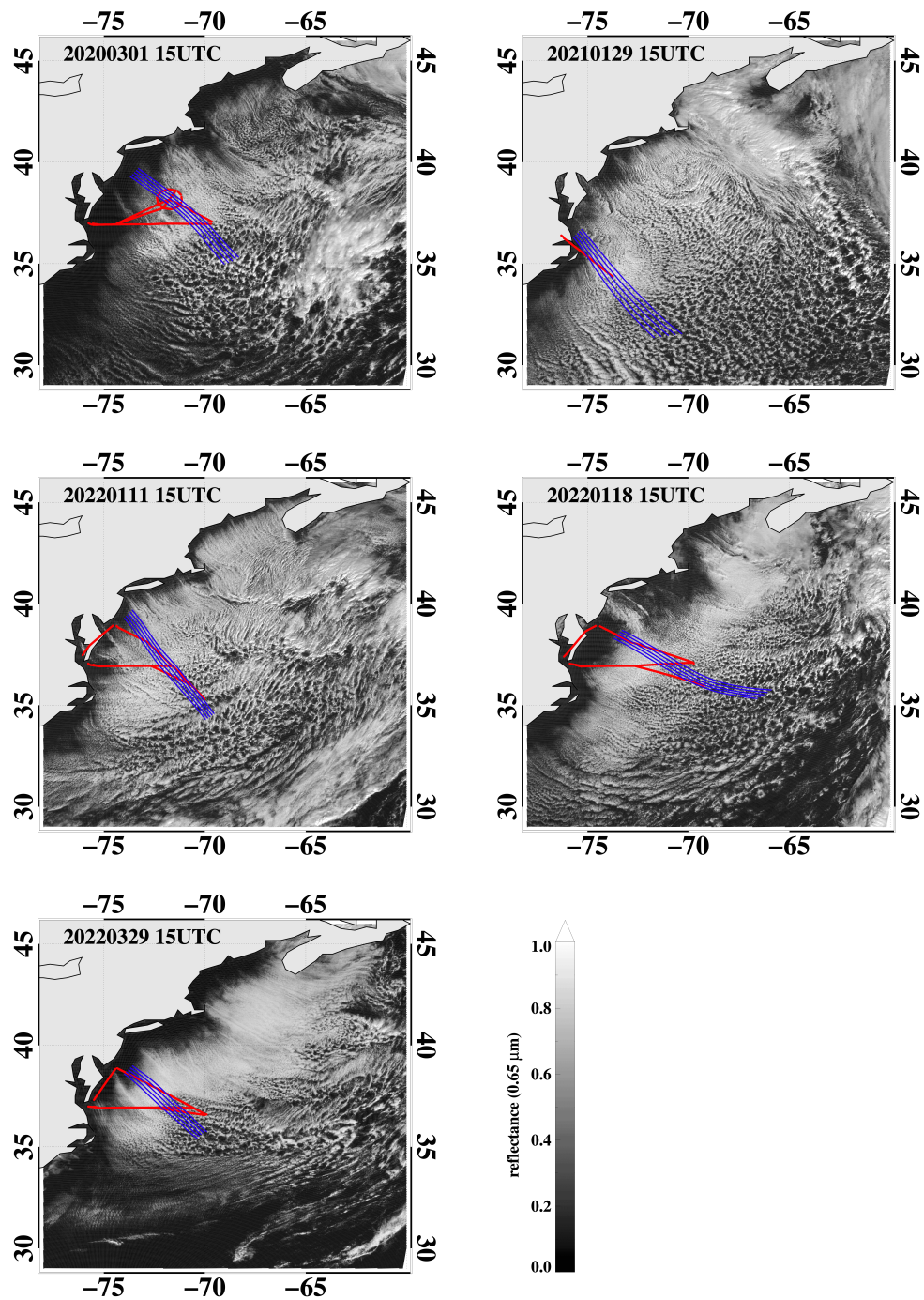
Figure S1. GOES-16 images of 0.65 \mu\text{m} reflectance overlaid with ACTIVATE flight tracks (KingAir) in red and 12-hr instantaneous trajectories at 15 UTC in blue for each MCAO events.
