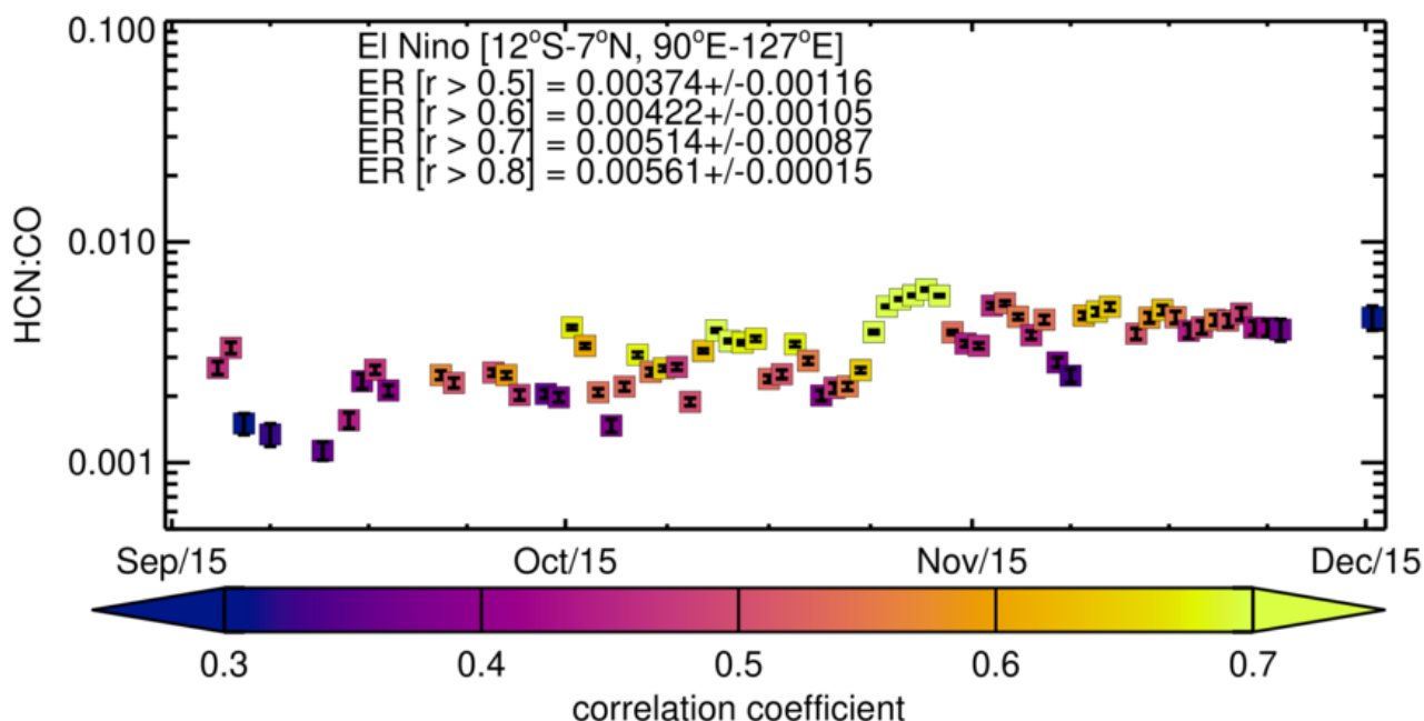
Figure 10. Daily HCN enhancement ratios (ER) relative to CO calculated from the slope of the linear regression of HCN against CO total columns between 1 September and 1 December 2015, over the Indian Ocean (12°S-7°N, 90°E-127°E). For completeness the error bars, although small, are included and correspond to the standard errors on the regression slope. Any data with a correlation coefficient <0.3 for the slope have been excluded.
