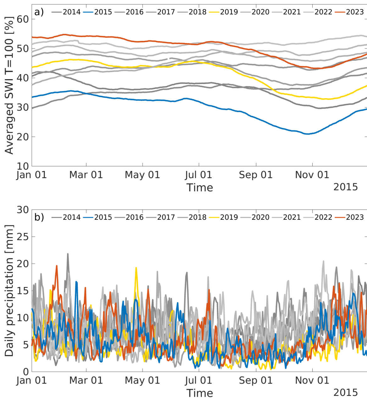
Figure 7. (a, top) Averaged SWI T=100, over Indonesia in the period 2014-2023. (b, bottom) Daily accumulated precipitation (combined microwave-IR) averaged over Indonesia estimate from the Integrated Multi-satellitE Retrievals for GPM (IMERG) in the period 2014-2023.
