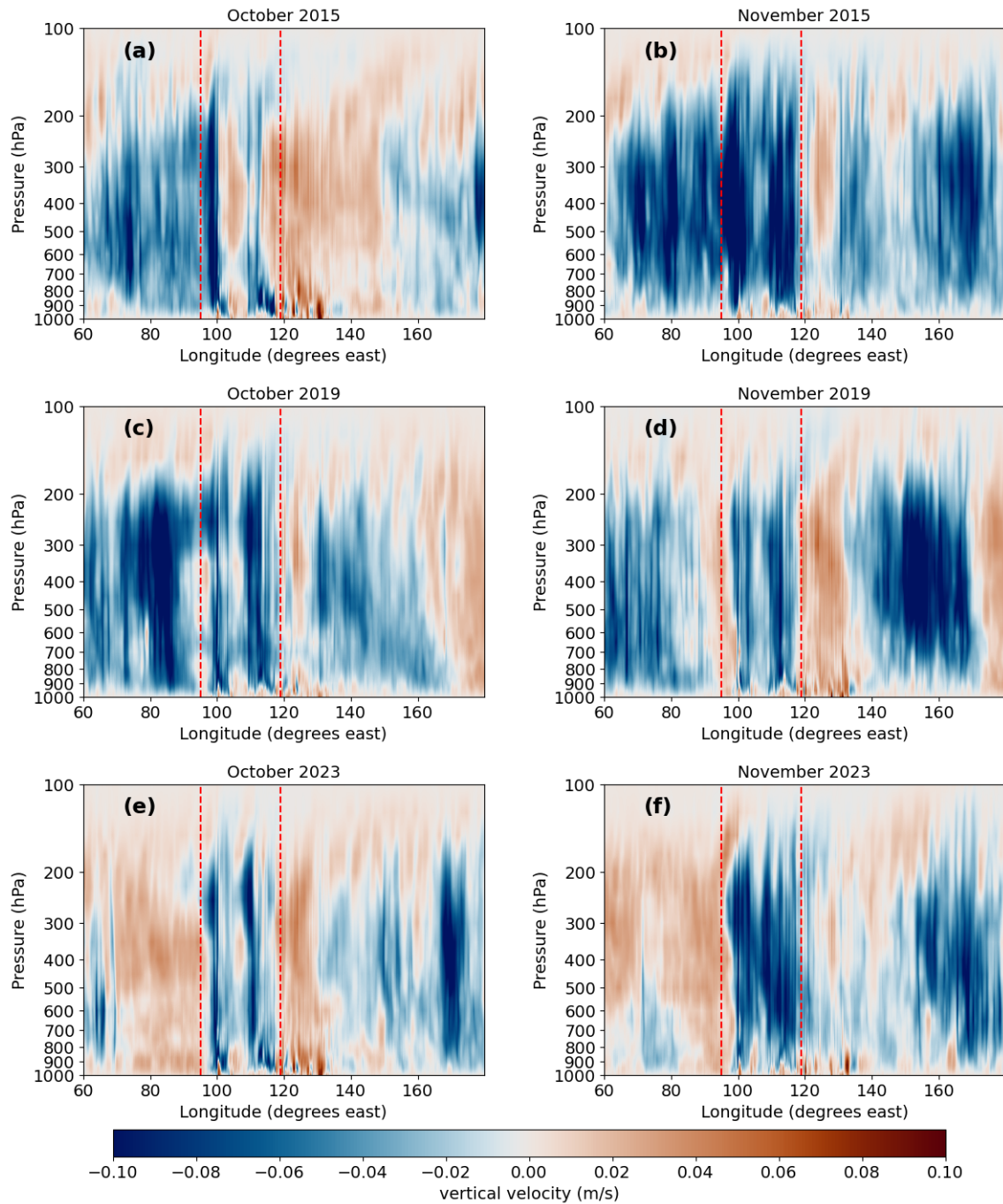
Figure 6. Monthly mean ERA5 vertical wind vectors (m s -1 ) averaged along the equator for (a) October 2015, (b) November 2015, (c) October 2019, (d) November 2019, (e) October 2023, and (f) November 2023 (Hersbach et al., 2023). Brown (blue) areas indicate where, on average, the air is descending (ascending) for that particular month. The red dashed lines highlight the approximate meridional extent of the Sumatra and Kalimantan regions.
