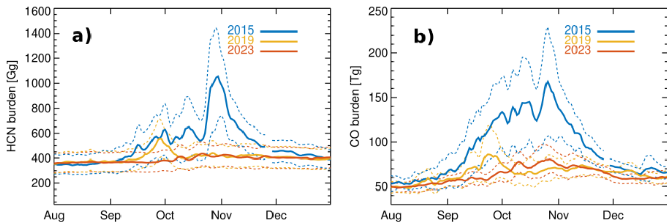
Figure 13. Daily Infrared Atmospheric Sounding Interferometer (IASI) derived a) HCN burden (Gg) and b) CO burden (Tg) between the 1 August and 31 December for three years: 2015 (blue line), 2019 (yellow line), and 2023 (red line). This is calculated for the region 12^{\circ}\text{S} - 7^{\circ}\text{N} , 90^{\circ}\text{E} - 127^{\circ}\text{E} .
