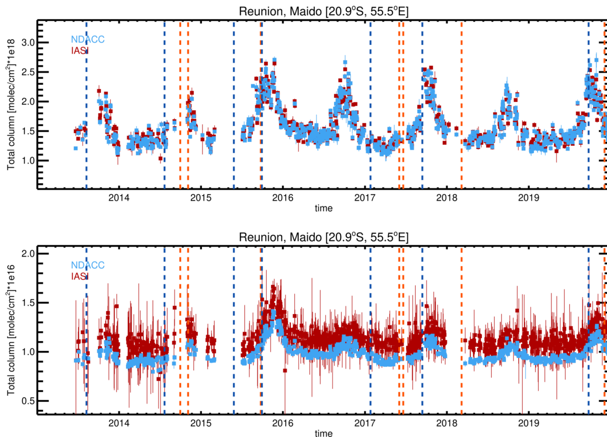
Figure 3. Time series of CO (top panel) and HCN (bottom panel) measurements for Reunion Maïdo. IASI measurements are shown in red with associated standard deviations (red lines). Ground-based FTIR measurements are shown in light blue with associated total error. The vertical blue (orange) dashed line represents where the IASI L2 (L1C) data processor version changed.
