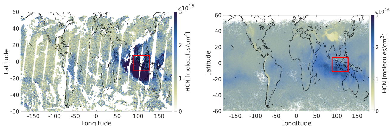
Figure 4. IASI global distribution of HCN total column (molecules \text{cm}^{-2} ) as retrieved by ULIRS for (a, left) 2 November 2015 during daytime and (b, right) the November 2015 monthly mean regridded on a 0.25^\circ \times 0.25^\circ grid. The red box indicates the region ( 12^\circ\text{S} - 7^\circ\text{N} , 90^\circ\text{E} - 127^\circ\text{E} ) over which the total column values are averaged.
