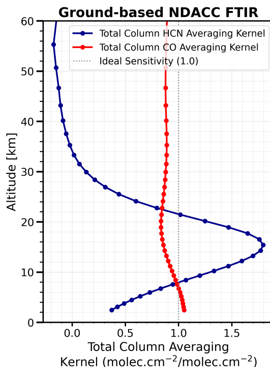
Figure 2. Average total column averaging kernels for ground-based FTIR at Reunion Maïdo for CO (red line) and HCN (blue line) for measurements made in 2015.
