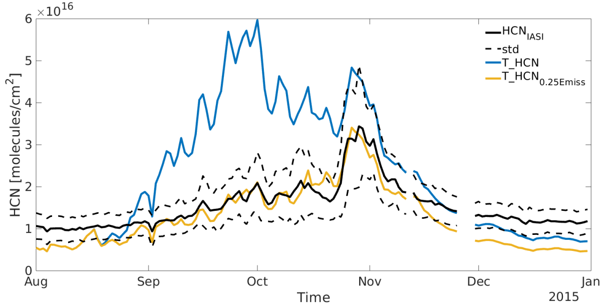
Figure 5. Comparison of the IASI measured HCN averaged total column time series (molecules \text{cm}^{-2} ) (black line), and HCN TOMCAT model run (T_HCN) using (i) monthly emissions from GFED v4.1 (blue line) and (ii) GFED v4.1 emissions with September values scaled to 25% (orange line). The errors are defined as the standard deviation of the averaged total columns over Indonesia within the region 12^{\circ}\text{S} - 7^{\circ}\text{N} and 90^{\circ}\text{E} - 127^{\circ}\text{E} .
