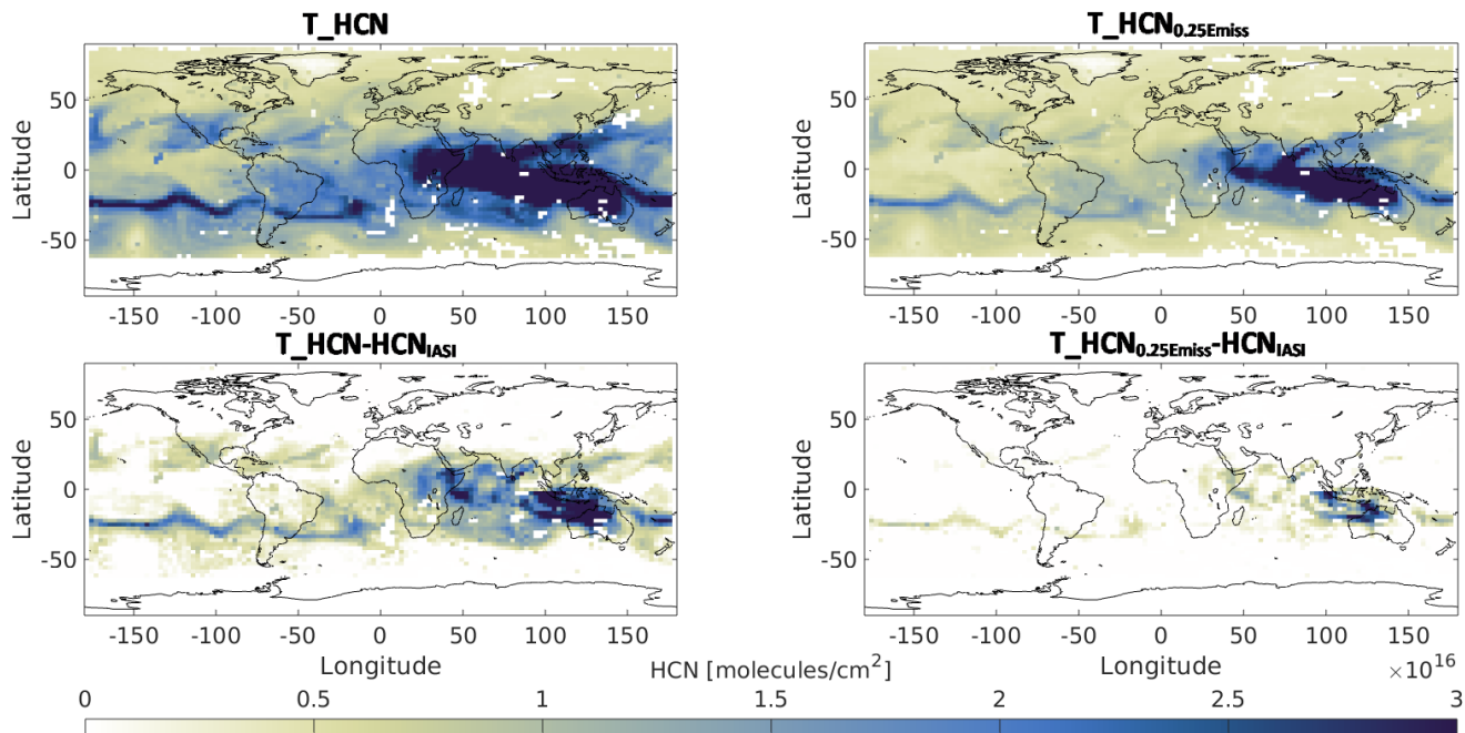
Figure 8. Global distribution of HCN total column (molecules \text{cm}^{-2} ) on 2 November 2015 produced from (a, top left) T\_HCN and (b, top right) T\_HCN_{0.25Emiss} . The bottom panels shows the total column difference between the two runs and the IASI measurements regridded on the TOMCAT grid.
