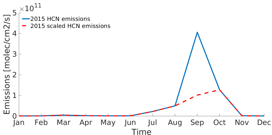
Figure 9. Monthly average HCN 2015 emissions (molecules \text{cm}^{-2} \text{s}^{-1} ) used in the T\_HCN TOMCAT model experiment (blue line) compared with the scaled emissions used in the T\_HCN_{0.25Emiss} experiment (red dashed line).
