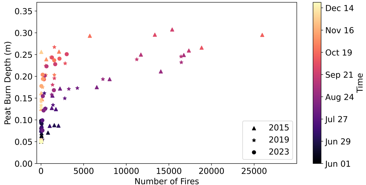
Figure 16. Weekly mean burn depth (m) of Indonesia peat fires between 1 June and 31 December in years 2015 (triangles), 2019 (stars) and 2023 (circles).
