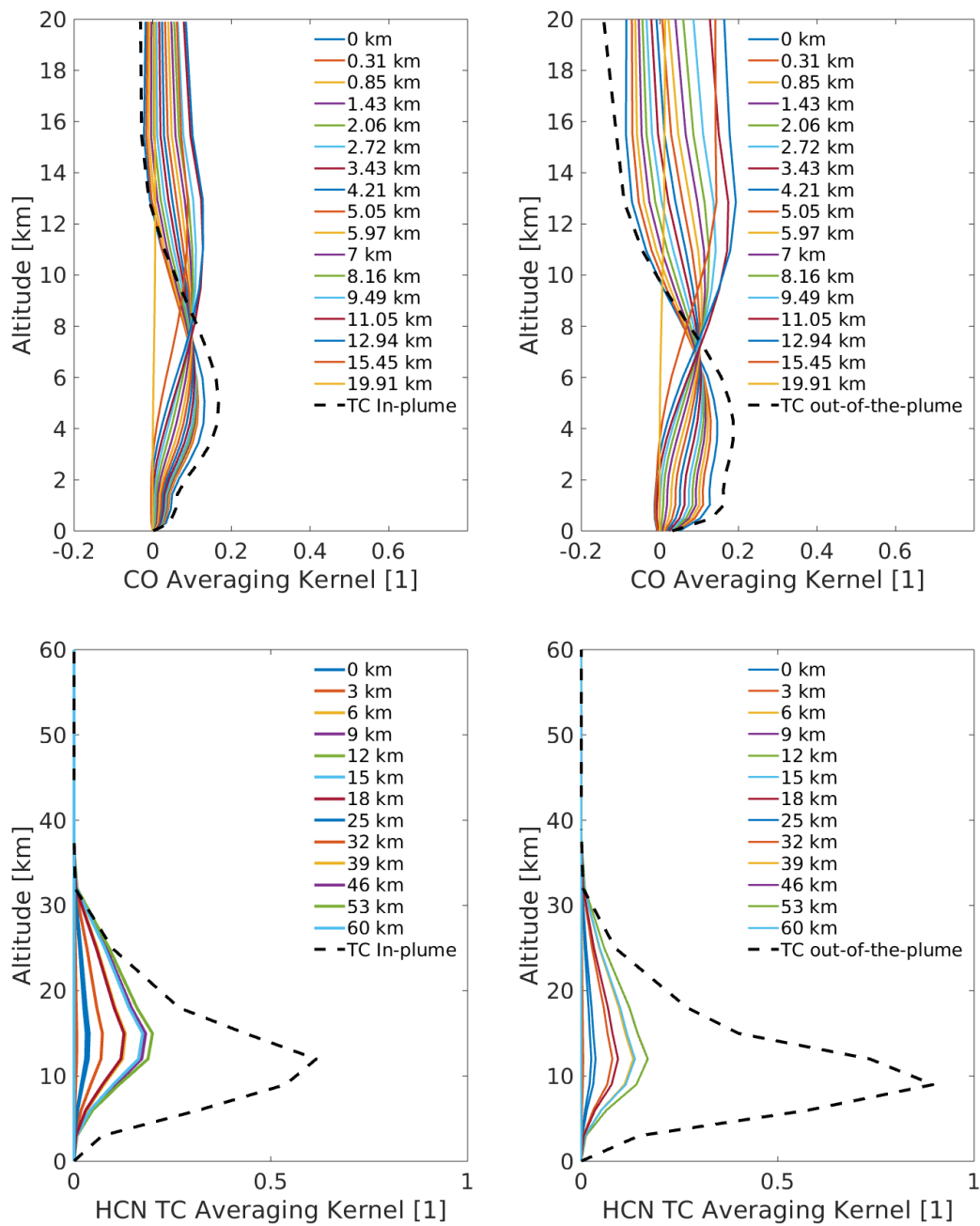
Figure 1. CO (top panels) and HCN (bottom panels) averaging kernels and total column averaging kernel for IASI measurements on the 2nd of November with the wildfire plume (110°E, 14.5°S) and outside the plume (95.4°E, 35°S).
