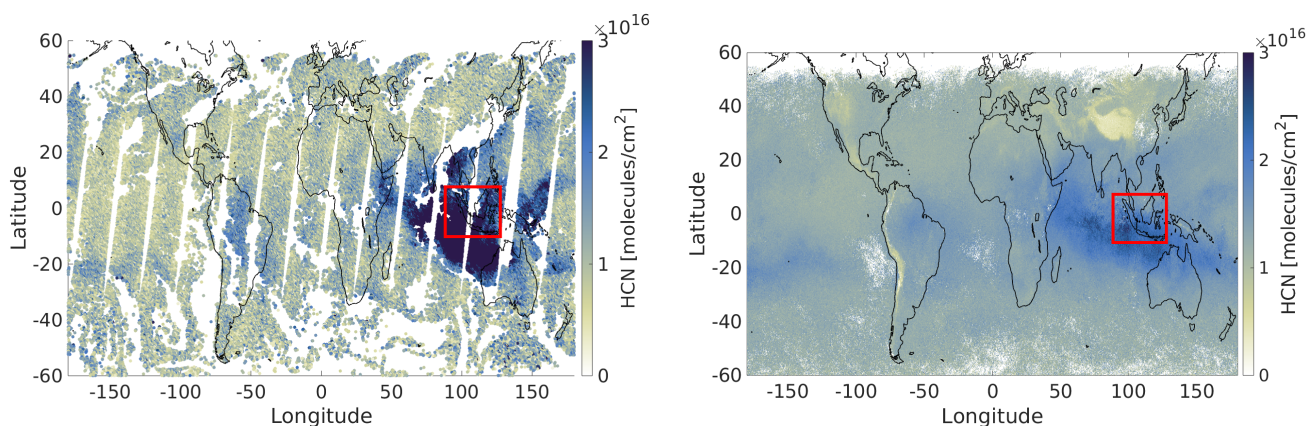
Figure 4. IASI global distribution of HCN total column (molecules cm -2 ) as retrieved by ULIRS for (a, left) +2 November 2015 during daytime and (b, right) the November 2015 monthly mean regridded on a 0.25° × 0.25° grid. The red box indicates the region (12°S-7°N, 90°E-127°E) over which the total column values are averaged.
