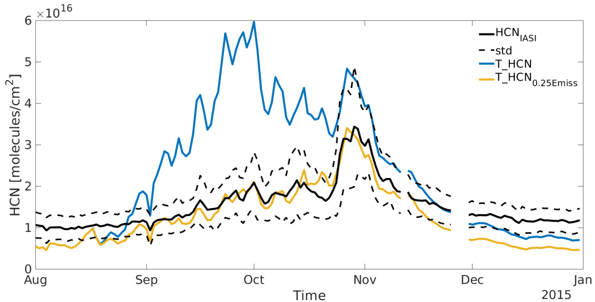
Figure 5. Comparison of the IASI measured HCN averaged total column time series (molecules \text{cm}^{-2} ) (black line), and HCN TOMCAT model run ( T_HCN ) using (i) monthly emissions from GFED v4.1 (blue line) and (ii) GFED v4.1 emissions with September values scaled to 25% (orange line). The errors are defined as the standard deviation of the averaged total columns over Indonesia within the region 12^{\circ}\text{S} - 7^{\circ}\text{N} and 90^{\circ}\text{E} - 127^{\circ}\text{E} .
