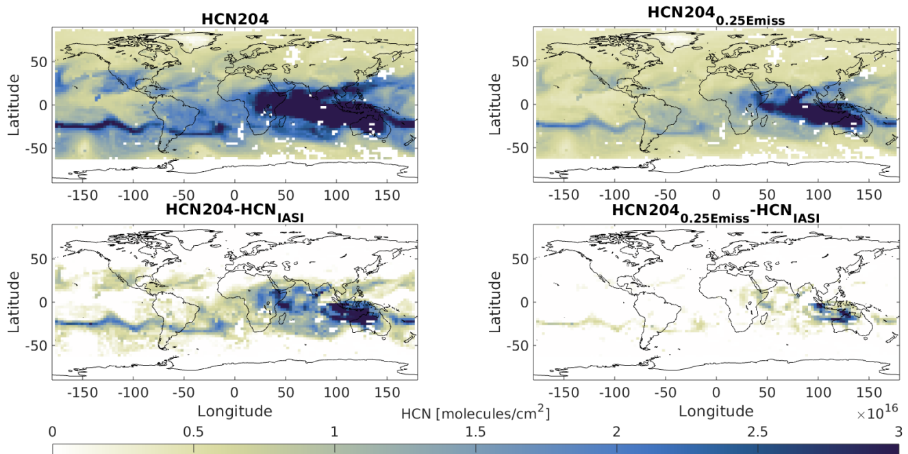
Figure 8. Monthly-average Global distribution of HCN 2015 emissions total column (molecules \text{cm}^{-2} ) based on GFED-v4.1 used in the 2 November 2015 produced from (a, top left) T_HCN TOMCAT model experiment and (blue line, top right) compared with the scaled emissions used in the T_HCN 0.25Emiss experiment (red dashed line). The bottom panels show the total column difference between the two runs and the IASI measurements regridded on the TOMCAT grid.
