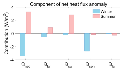
Figure 6. Composite anomalies of net heat flux and its components (W/m 2 ) in the North Sea during winters (blue bars) and summers (red bars) with positive values in the cluster-specific time series. Components include shortwave ( Q_{sw} ) and longwave ( Q_{lw} ) radiation, as well as the net latent ( Q_{la} ) and sensible ( Q_{sen} ) heat flux anomalies. Positive values indicate ocean heat gain from the atmosphere, while negative values indicate heat loss.
