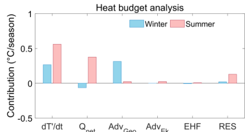
471 Figure 8. Quantitative contribution (°C/season) of atmospheric and oceanic processes to the upper ocean temperature 472 anomaly tendency for two clusters identified by the K-means algorithm. The atmospheric and oceanic variables are 473 shown as composite patterns during positive phases of the cluster-specific time series in winter (blue) and summer 474 (red). The temperature tendency ( dT'/dt ) represents the difference in the sea surface temperature anomaly between 475 February and December for winter and between August and June for summer, respectively. Contributions from the 476 net heat flux anomaly ( Q_{net} ), geostrophic heat advection ( Adv_{Geo} ), Ekman heat advection ( Adv_{Ek} ), entrainment heat 477 flux (EHF), and residual term (RES), averaged over the same periods, are also shown.
