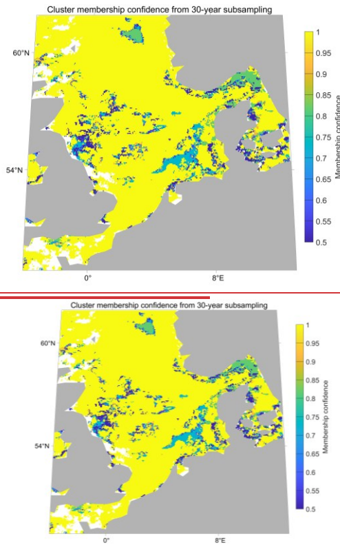
Figure A2. Robustness of the K-means clustering based on temporal subsampling.
