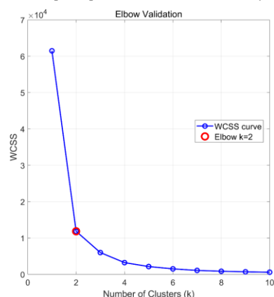
746 Figure. A1. Elbow method validation of K-means clustering of marine heatwave cumulative intensity (MHWCI) in 747 the North Sea. The within-cluster sum of squared correlation distances (WCSS) is shown as a function of cluster 748 numbers. The red circle indicates the optimal number of clusters determined by the Elbow method. WCSS denotes 749 the within-cluster sum of squared correlation distances and is a dimensionless clustering metric.
