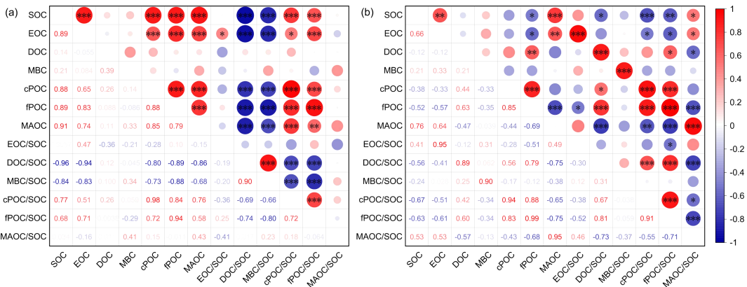
Figure 4: Pearson correlations among soil organic carbon (SOC) fractions and their relative proportions in greenhouses for (a) loam and (b) sandy loam. Note: SOC fractions represent concentrations (g kg -1 ), include total SOC, easily oxidizable organic carbon (EOC), dissolved organic carbon (DOC), microbial biomass carbon (MBC), coarse particulate organic carbon (cPOC), fine particulate organic carbon (fPOC), and mineral-associated organic carbon (MAOC). Their relative proportions to SOC include EOC/SOC, DOC/SOC, MBC/SOC, cPOC/SOC, fPOC/SOC, and MAOC/SOC. * Correlation was significant at P \leq 0.05 ; ** Correlation was significant at P \leq 0.01 ; *** Correlation was significant at P \leq 0.001 .
