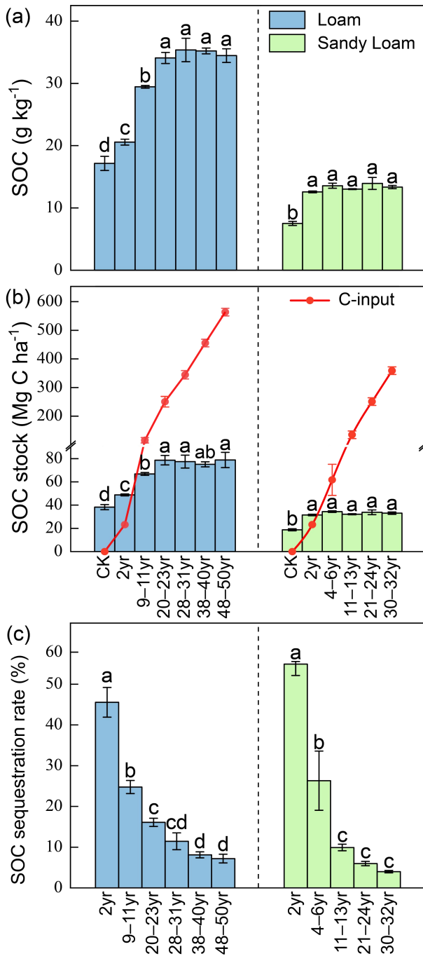
Figure 1: Changes in (a) soil organic carbon (SOC), (b) manure-derived carbon input and SOC stock, and (c) SOC sequestration rate following manure application over various years in greenhouses. Bars represent the standard errors. Within each soil texture, bars with different lowercase letters indicate significant differences among years of manure application ( P < 0.05 ).
