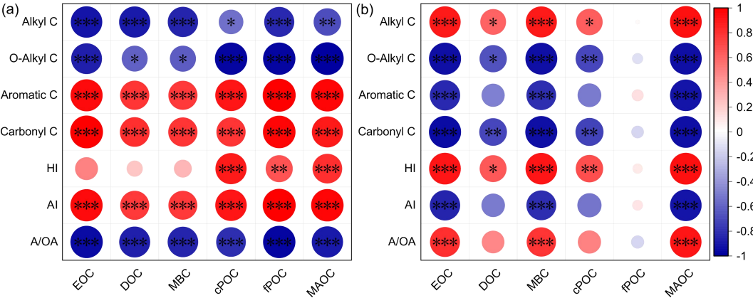
Figure 6: Pearson correlations between soil organic carbon (SOC) fractions based on their concentrations ( \text{g kg}^{-1} ) and SOC chemical structure and stability indices in greenhouses (a) loam and (b) sandy loam. Note: SOC fractions include total SOC, easily oxidizable organic carbon (EOC), dissolved organic carbon (DOC), microbial biomass carbon (MBC), coarse particulate organic carbon (cPOC), fine particulate organic carbon (fPOC), and mineral-associated organic carbon (MAOC). SOC stability indices include aromaticity index (AI), hydrophobicity index (HI), and the ratio of alkyl C to O-alkyl C (A/OA). * Correlation was significant at P \leq 0.05 ; ** Correlation was significant at P \leq 0.01 ; *** Correlation was significant at P \leq 0.001 .
