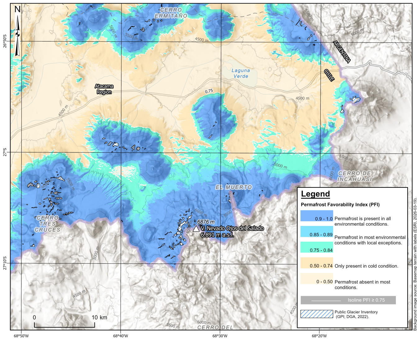
Figure A1. Permafrost favorability index map for a sample area in the dry Andes, Atacama region, at 27° S. Basemap Esri Terrain with Labels.
