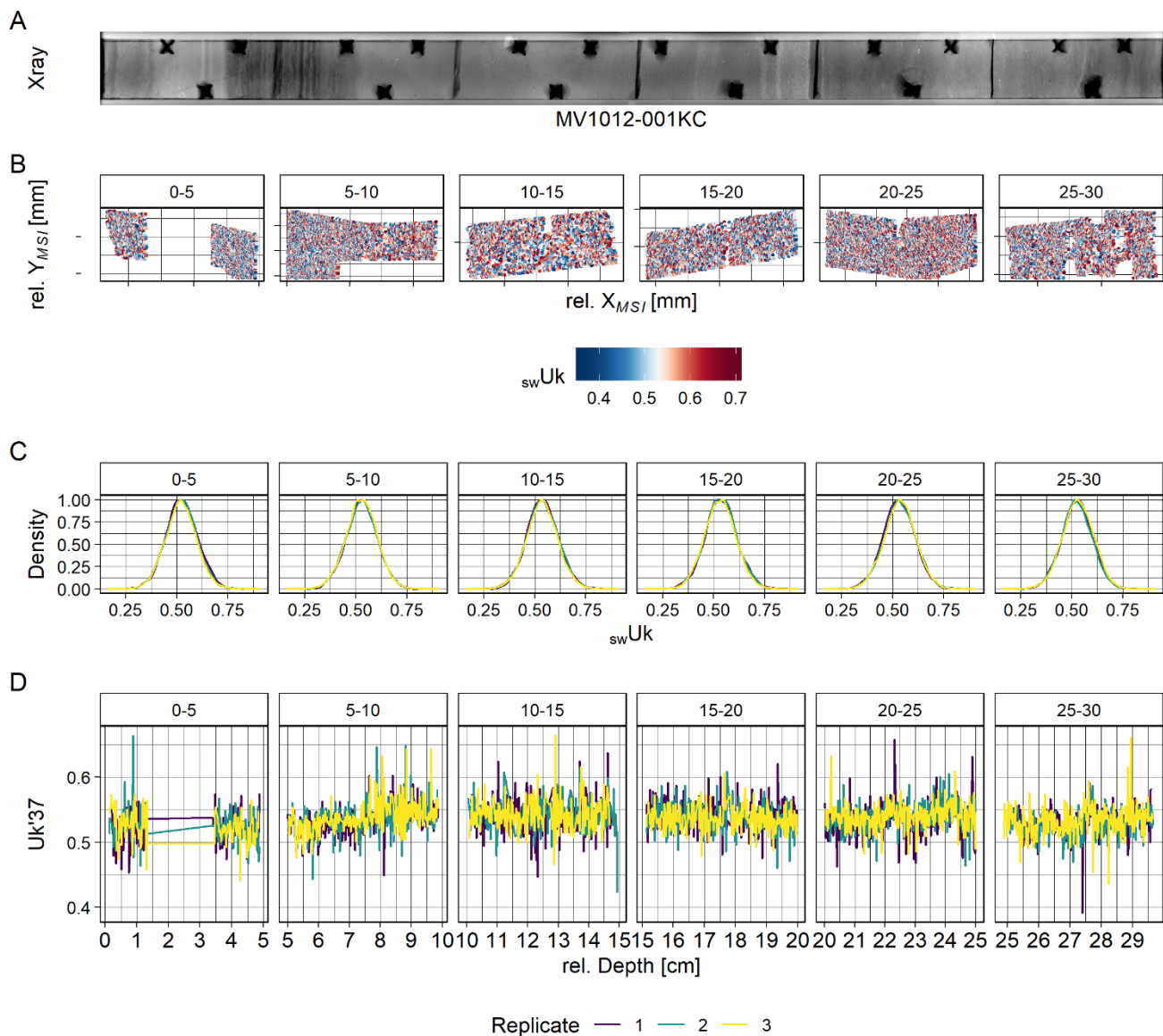
220 Figure 2: Maps and time-series of sediment section KC1. (A) X-ray density map with black crosses or rectangles where material was removed as markers for orientation of the samples, (B) exemplary swUk (spotwise U_{37}^{K'} ) maps of one replicate per depth interval. Maps are shown on the MSI coordinate grid before affine transformation onto X-ray coordinates. swUk values below the 1% and above the 99% quantiles were removed for improved color scaling during plotting. (C) Scaled density plots of the spatial swUk maps per replicate. (D) Resulting U_{37}^{K'} time-series per replicate and depth interval. Note that the area corresponding to the 1761 AD floodlayer in depth interval 0-5 cm was removed prior to analyses. For A, B and D the directionality is from left (“modern”) to right (“past”). An exposure artefact was
