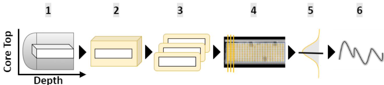
95 Figure 1: Schematic representation of the triplicate workflow. 1) Subsampling from sediment cores via 30 cm LL-channels (Suigetsu 2006 Project Members and Nakagawa, 2014), used for X-ray photography; 2) freeze-drying and embedding of 5-cm subsections (“pieces”), 3) cryomicrotome cutting onto ITO slides of 3 subsequent 100-µm “slices” per piece; 4) MSI scans; 5) data processing, horizon-wise aggregation & conversion to time series; 6) time series analyses. Orientation of sediment samples and time series is left to right: core top (“recent”) to depth (“past”).
