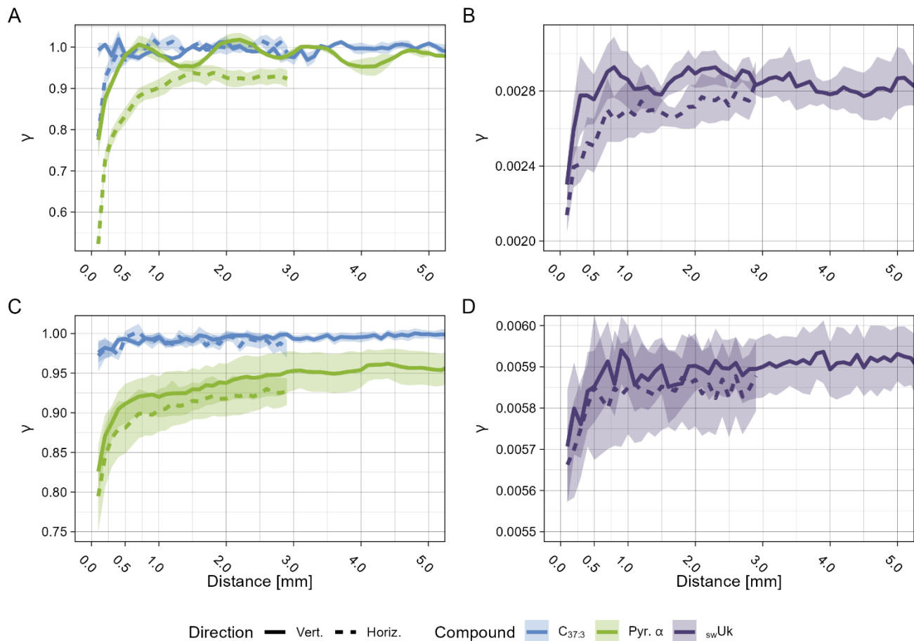
270 Figure 4: Variogram estimates of pyropheophorbide \alpha and C37:3 intensities and swUk (spotwise U_{37}^{K'} ) temperatures, showing the semivariance or dissimilarity of pairwise spot comparisons ( \gamma ) as a function of distance. Solid lines indicate sample variogram estimates along the vertical, downcore direction of the original sediment position; dashed lines indicate within-layer estimates, parallel to the sediment surface. A and B are obtained for the exemplary varved section of SBX, averaged over 3 replicates. C and D for sediment segment KC1, averaged over all replicates and depth intervals (3 x 6 x 5 cm). Note that each panel has individual y-axes, as pyropheophorbide \alpha and C37:3 values in A, C were scaled 275 prior to calculation and are not in their native units, whereas in B, D \gamma values correspond to U_{37}^{K'} units.
