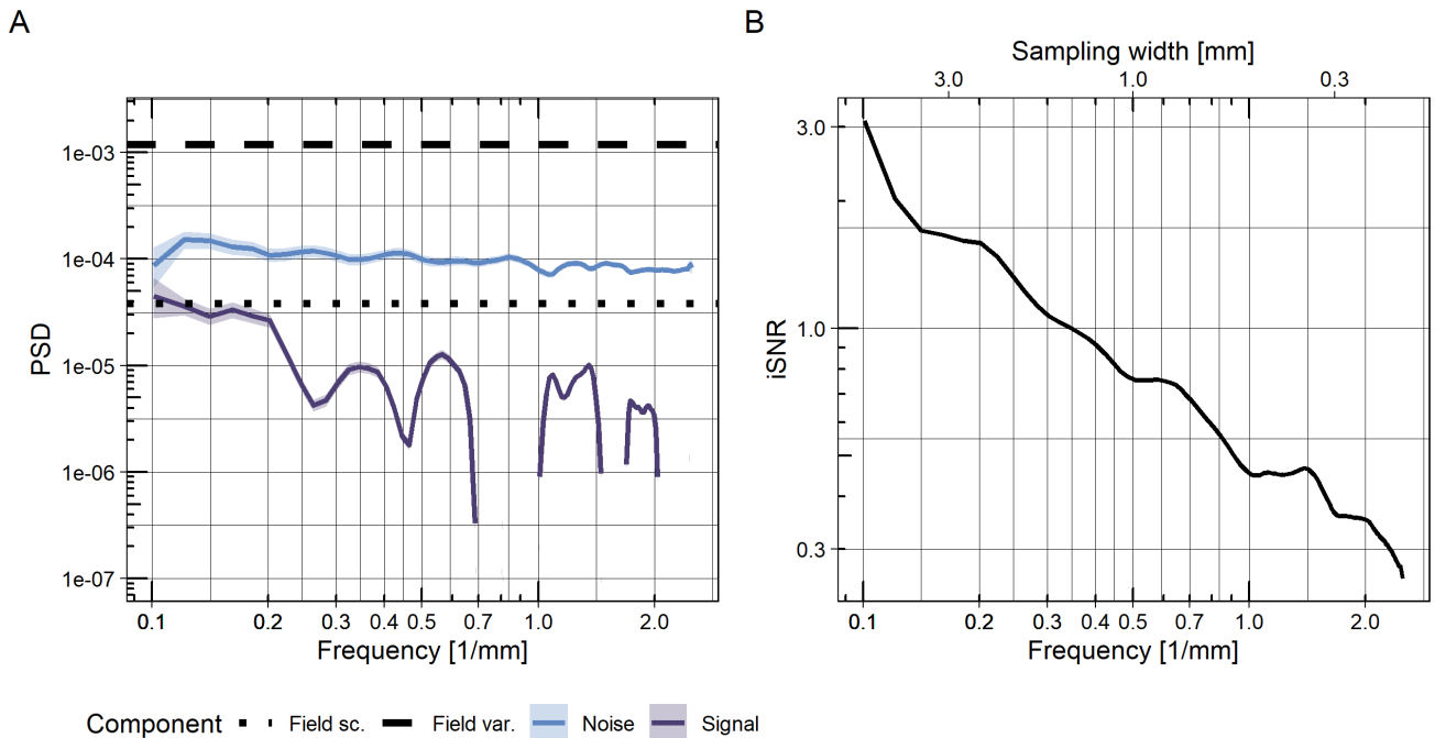
295 Figure 5: Frequency-dependent signal and noise components in comparison to field variance (A) and the resulting integrated SNR (iSNR) estimate (B). The dashed line shows the average variance of the swUk field in black; the dotted line is the field variance downsampled by the average number of swUk shots per horizon, imitating the noise reduction during time series processing.
