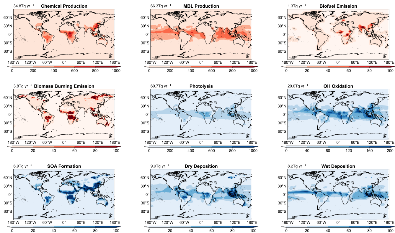
Figure 4. Annual mean sources and sinks of simulated atmospheric glyoxal in the GC-TM-EC simulation [unit: \text{kg km}^{-2} \text{ year}^{-1} ]. Global annual sums of individual sources and sinks are shown inset.
