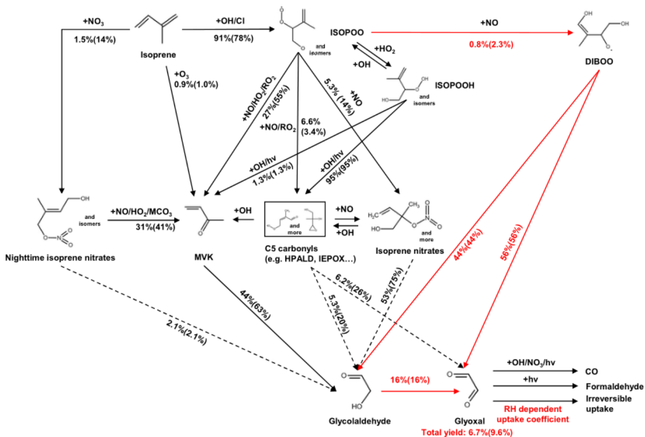
Figure 5. Gas-phase production of glyoxal and glycolaldehyde from the oxidation of isoprene as represented in the standard RCIM (black arrows) and as revised in this work (red arrows). Branching ratios outside and inside parentheses were calculated under NO concentrations of 0.1 ppb and 5 ppb, respectively. The solid or dashed arrows denote pathways comprehensively or partially constrained by experiments, respectively. We set [\text{OH}] = 1.8 \times 10^6 \text{ molecules cm}^{-3} , [\text{O}_3] = 40 \text{ ppb} , and \text{RH} = 55\% ; other environmental conditions were representative of a subtropical site in fall. Pathways with glyoxal yields less than 1% are not shown in this figure.
