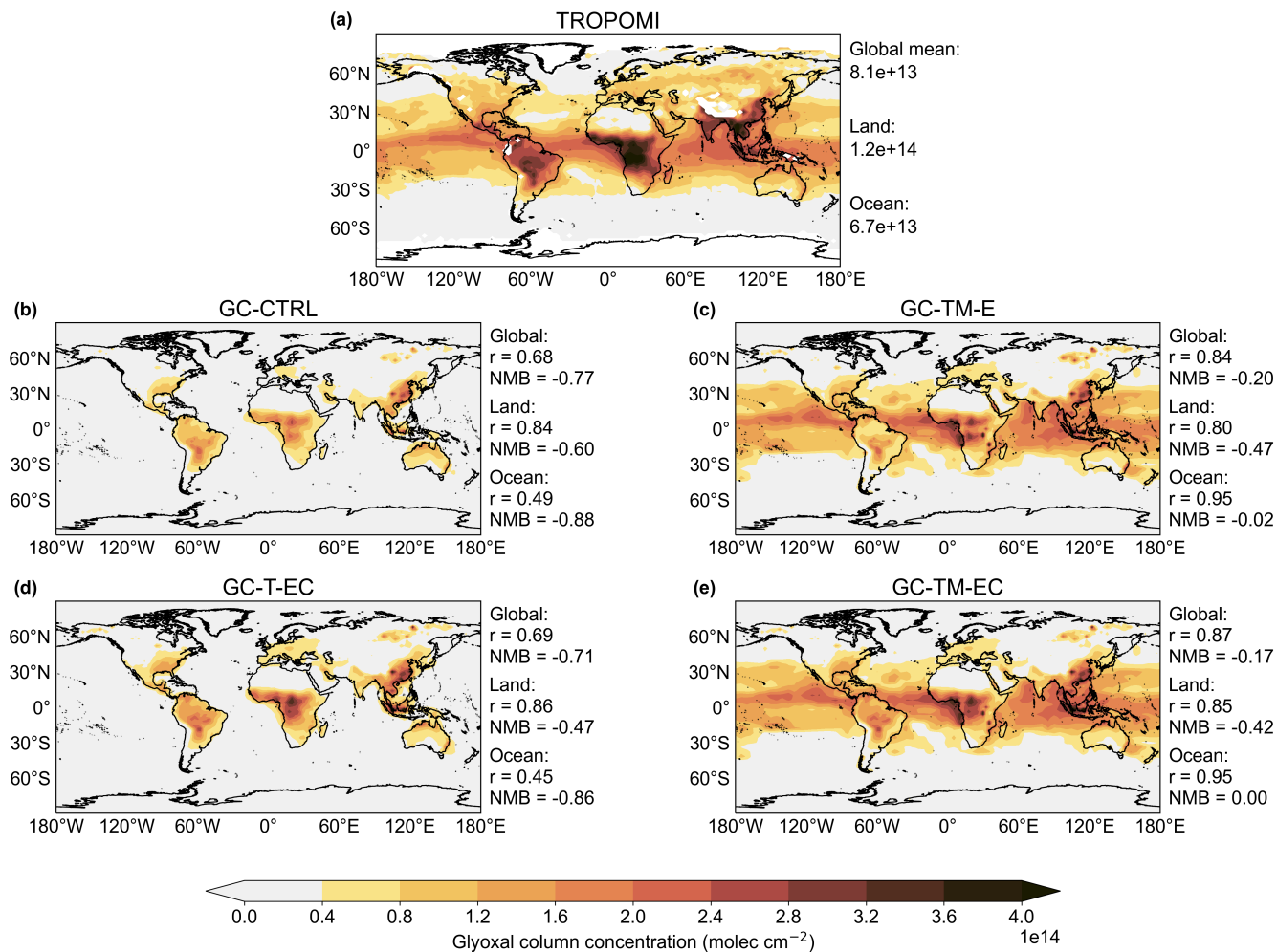
Figure 1. Annual mean (July 2019—une 2020) atmospheric glyoxal column concentrations as (a) observed by TROPOMI, and as simulated in the (b) GC-CTRL , (c) GC-TM-E , (d) GC-T-EC , and (e) GC-TM-EC experiments. Model statistics against the TROPOMI observations over land, ocean, and globally are shown on the side of panels (b) to (e). The simulated VCDs were sampled at the daily satellite overpass time (13:30 local time) and then averaged to annual means.
