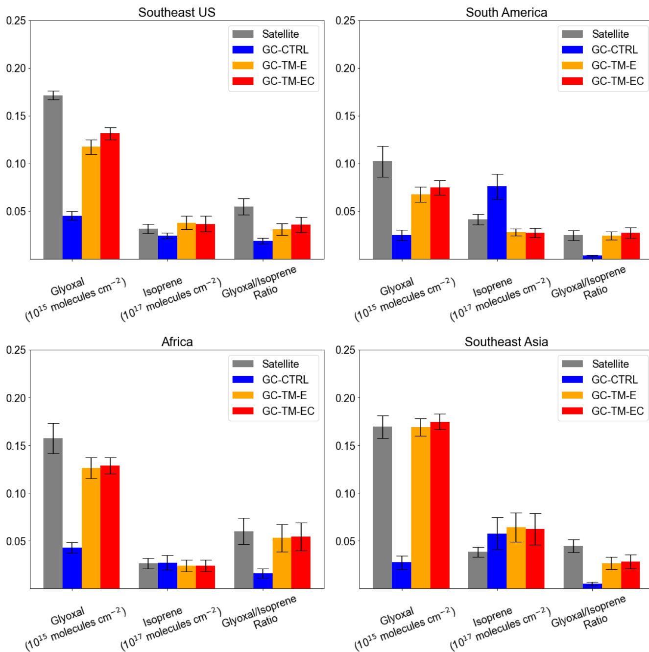
Figure 7. Comparison of the satellite-retrieved and simulated column concentrations-VCDs of glyoxal (from TROPOMI) and isoprene (from CrIS-ANN) and their ratios over regions dominated by seasonal biogenic NMVOC emissions: (a) Southeast U.S. (August to October), (b) South America (annual mean), (c) Africa (annual mean), and (d) Southeast Asia (annual mean). Error bars indicate standard deviation of monthly mean column concentrations-VCDs and ratios, respectively.
