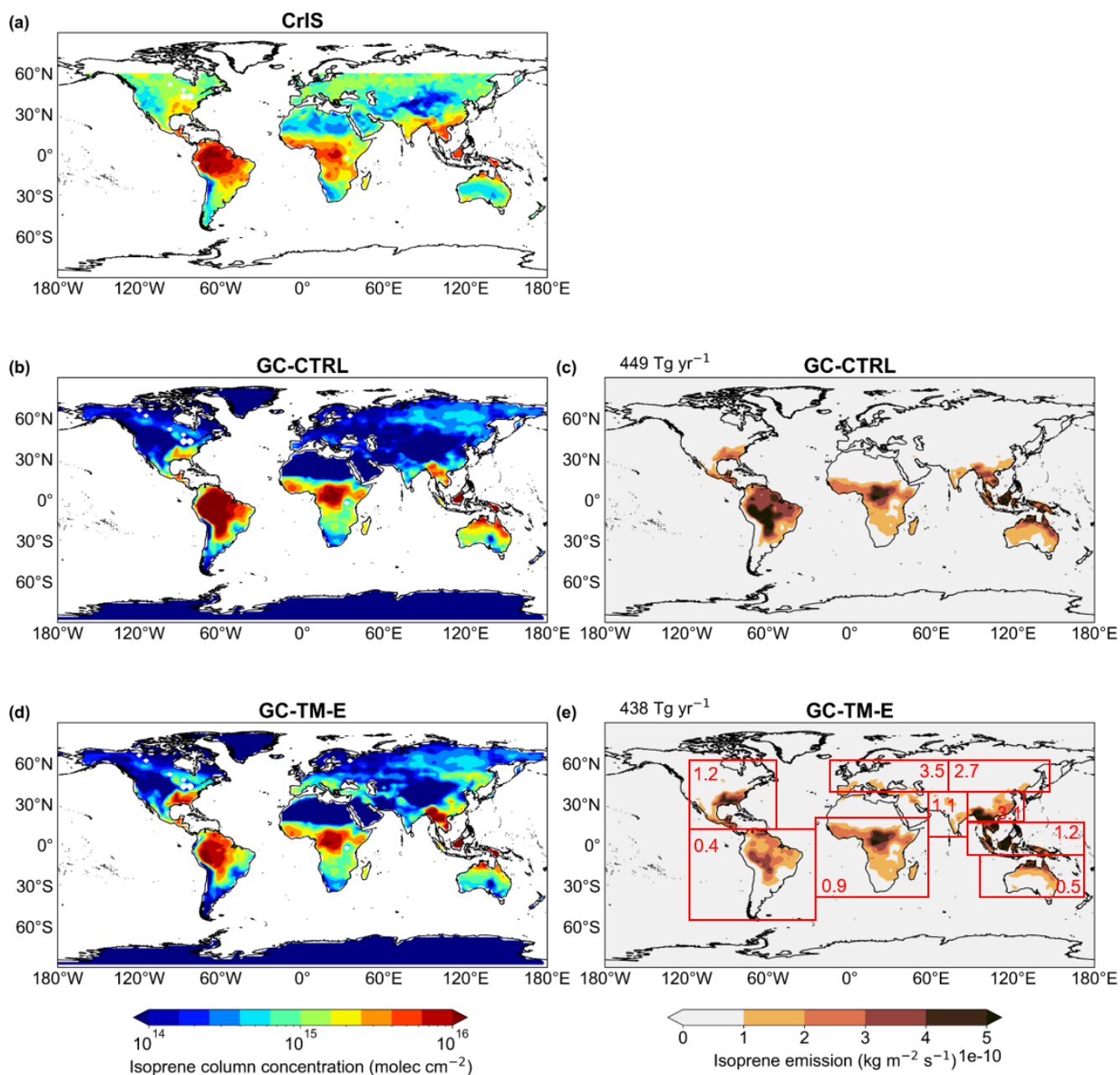
Figure 3. Annual mean tropospheric isoprene column concentrations VCDs (a) as observed by CrIS and as simulated in the (b) GC-CTRL and (d) GC-TM-E experiments, respectively. Also shown are the annual mean isoprene emissions (c) from the GC-CTRL simulation and (e) those scaled and used in the GC-TM-E simulation (also used in GC-T-EC and GC-TM-EC). The areas over water or with no data are shaded white in (a) (b) and (d). The numbers in red boxes indicate the regional mean ratios of isoprene emissions in (e) relative to those in (c).
