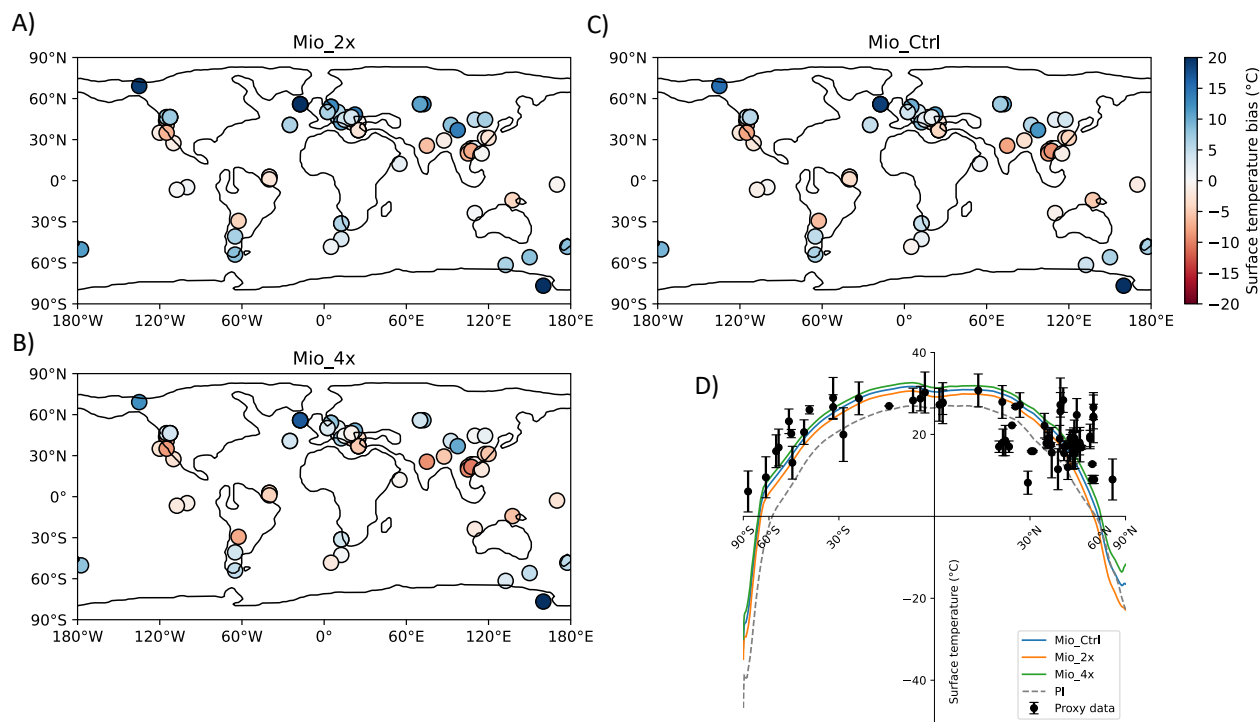
Figure 5. Surface temperatures temperature biases relative to the proxy record at A) 2 (Mio_2x), B) 4 (Mio_4x) and C) 3 (Mio_Ctrl) times pre-industrial PI CO 2 concentrations relative to the proxy record , at proxy sites and D) zonally. Proxy sites are rotated on the mid-Miocene geography with the tectonic model of Getech Plc.
