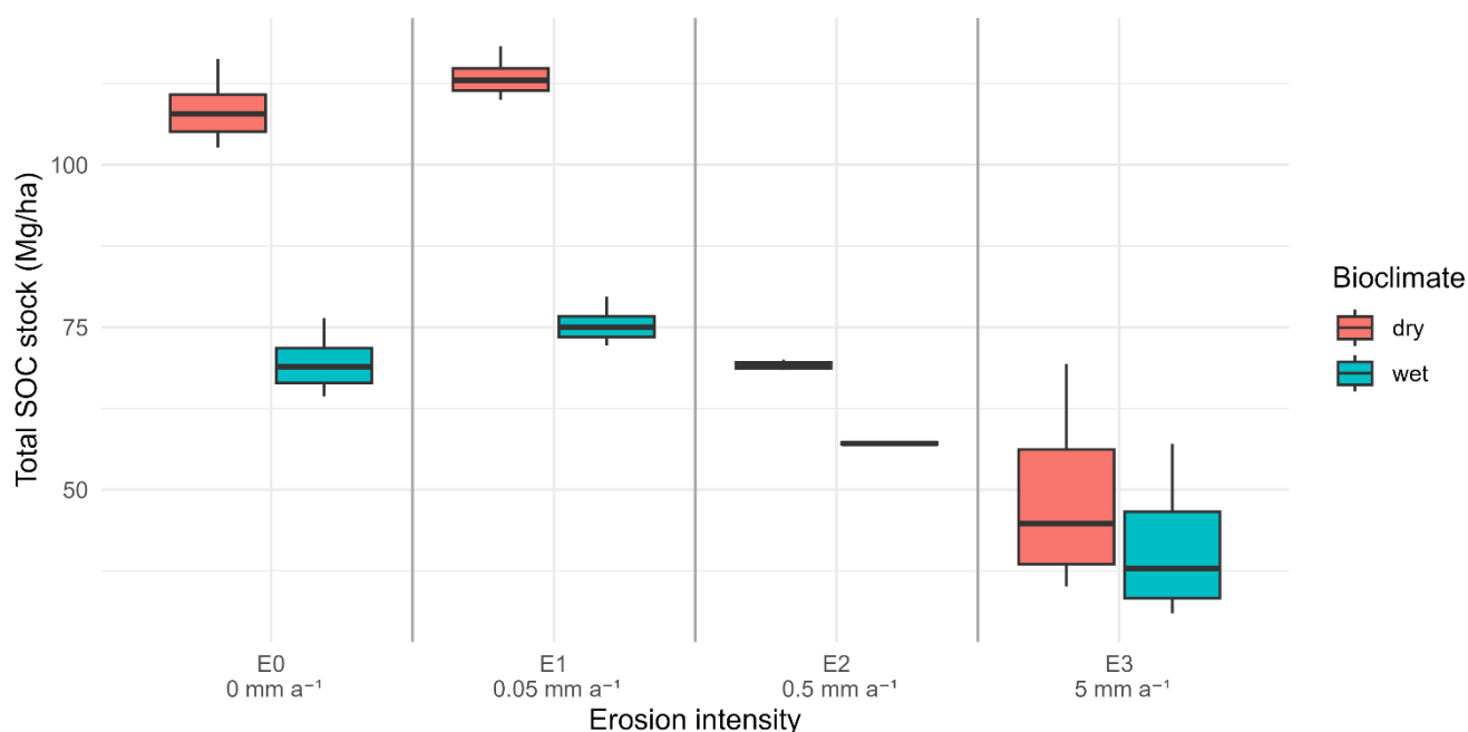
Figure 3: Distribution of annual SOC stocks in the intensive agricultural phase (years 9900 – 10000), grouped per erosion intensity and bioclimate. The visualized scenarios are with all protection mechanisms combined (x).
