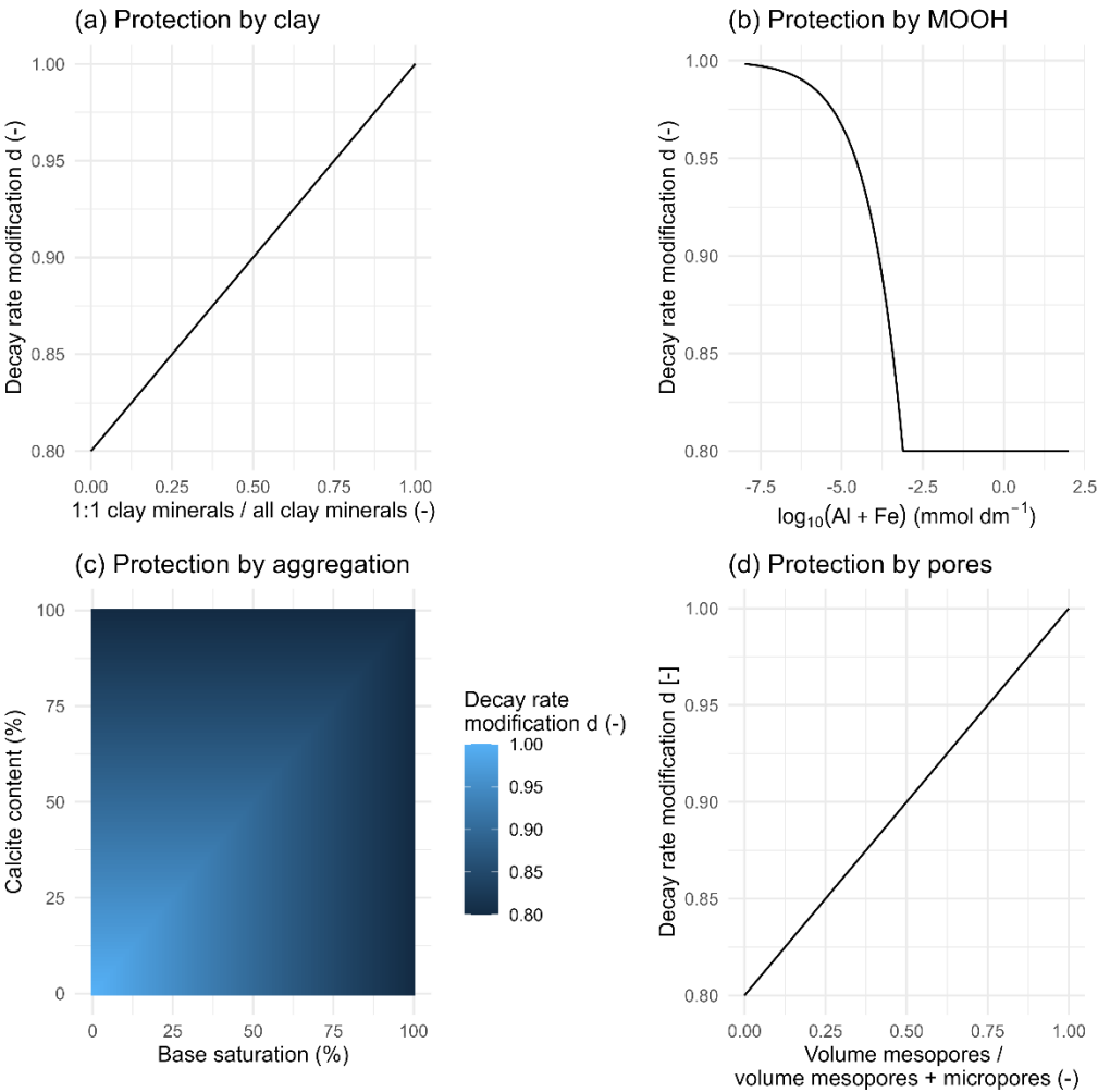
Figure A3: SOC decay rate modifiers for (a) clay mineralogy, (b) metal oxyhydroxides (MOOHs), (c) aggregation and (d) porosity as influenced by soil variables. Rate modifiers vary between 0.8 (protection) to 1 (no protection).
