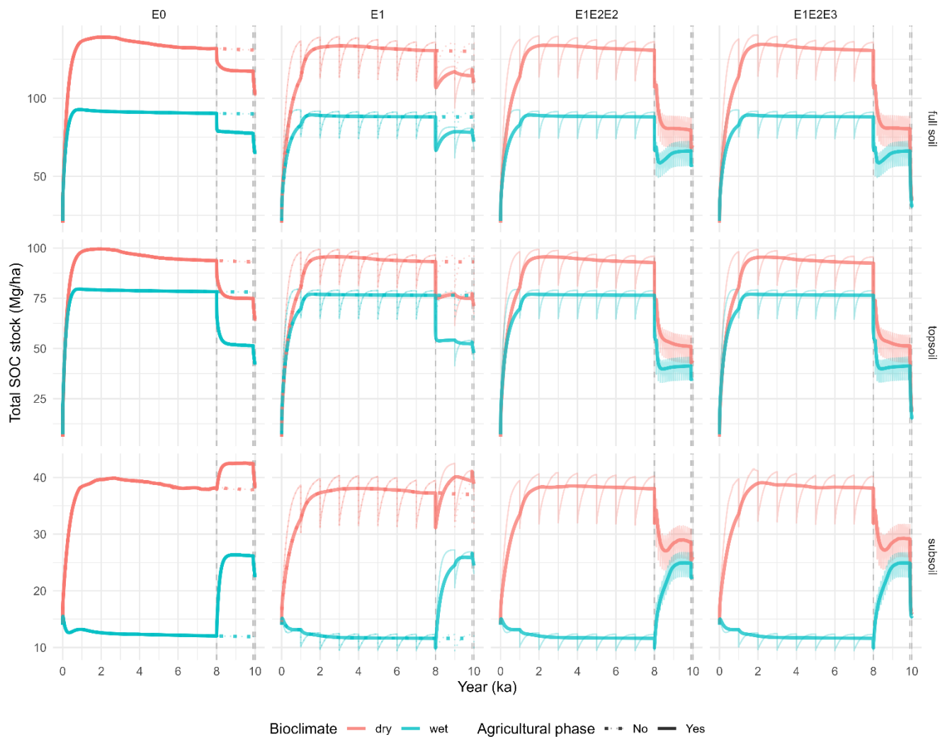
Figure B2: Simulated SOC stock dynamics under different erosion scenarios (columns) separated for the entire soil profile, topsoil (< 25 cm) and subsoil (25-100 cm, rows), for both bioclimate scenarios (colours) and anthropogenic effects (line types). The simulations are based on all protection mechanisms combined (x). Note the different ranges on the Y axis. The thin lines visualize the raw model output, while the bold lines show the SOC stocks that are smoothed using a moving average. The dotted bold line depicts continued natural evolution.
