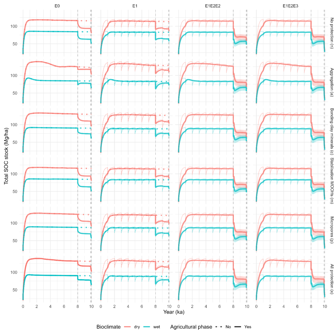
Figure B1: Simulated SOC stock dynamics for different protection mechanisms (rows), erosion scenarios (columns), bioclimates (colours) and anthropogenic effects (line types). The thin lines visualize the raw model output, while the bold lines show the SOC stocks that are smoothed using a moving average. The dotted bold line depicts continued natural evolution.
