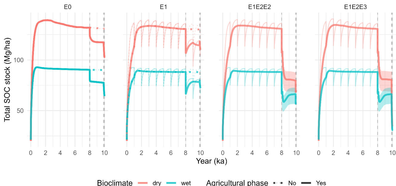
Figure 2: Simulated SOC stock dynamics for different erosion scenarios (columns), bioclimates (colours) and anthropogenic effects (line types). The erosion rates corresponding to the erosion scenarios are provided in Table 2. The visualized scenarios are with all protection mechanisms combined (x). The thin lines visualize the raw model output, while the thick lines show the SOC stocks that are smoothed using a moving average. The dotted bold line depicts continued natural evolution.
