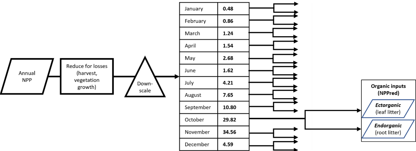
520 Figure A1: Litter inputs ( NPP_{red} ) derived from annual Net Primary Production (NPP), reduced for losses and downscaled to monthly litter production. The values (user input) are monthly percentages (here: for deciduous forest).
