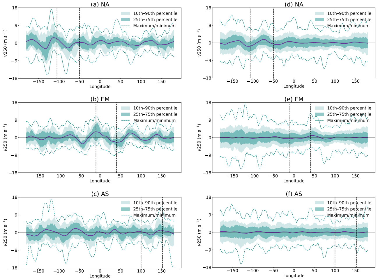
Figure A3: Meridional component of the wind at 250 ( v_{250} ), averaged over the 57.5°N - 37.5°N belt. On the left column, composites of 19 high FA events; on the right column, composites of 92 low FA events, in (a,d) North America (NA), (b,e) Euro-Mediterranean (EM) and (c,f) Eastern Asia (AS). Purple lines indicate the composite mean, dark green bands indicate the interquartile range, light green bands indicate the 10 th -90 th percentile range, dashed green lines indicate maxima and minima, while vertical black dashed lines indicate the longitudinal extension of the selected regions.
