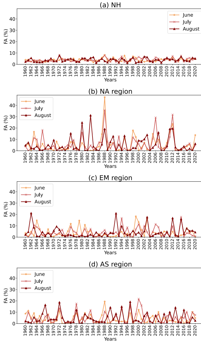
245 Figure 4: Fraction of Area (FA) affected by COHDEs during June, July and August, from 1960 to 2020, in a) the Northern Hemisphere, b) North America (NA), c) Euro-Mediterranean (EM) and d) eastern Asia (AS).
