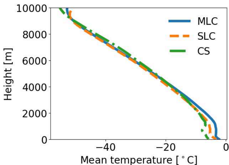
Fig. A Mean vertical temperature profiles.
