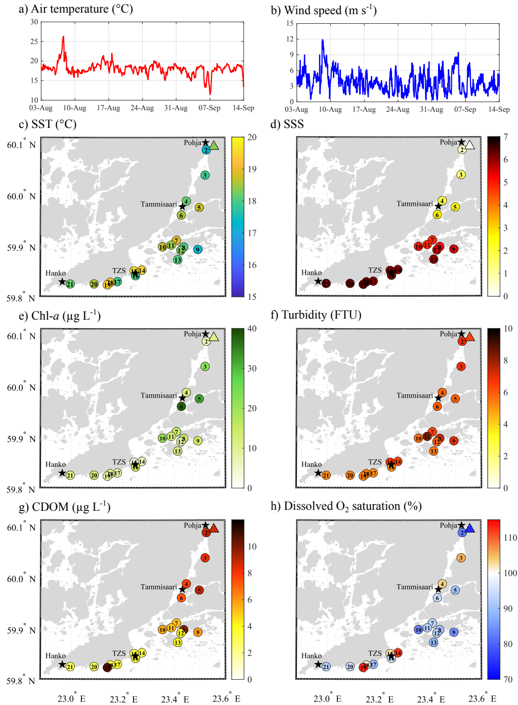
Figure 1: Atmospheric conditions: a) air temperature (°C) and b) wind speed (m/s) recorded at the ICOS station FI-Tvm established at the Tvärminne Zoological Station. Spatial variation of c) surface seawater temperature (SST, °C), and d) salinity (SSS), e) chlorophyll- a (Chl- a , \mu\text{g L}^{-1} ) concentration, f) turbidity (FTU), g) colored dissolved organic carbon (CDOM, \mu\text{g L}^{-1} ), and h) dissolved oxygen saturation (%) across the sampling area. Triangles represent the surface water conditions at the mouth of the Karjaanjoki River.
