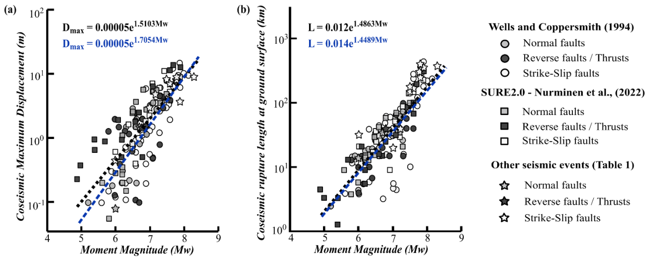
Figure 2: Scaling laws correlating coseismic geometric fault attributes (maximum displacement and rupture length at the ground surface) and earthquake magnitude (a, b, respectively). Blue trend lines are calculated from Wells and Coppersmith (1994), black trend lines are calculated considering also data from the SURE2.0 database (Nurminen et al., 2022) and Table 1.
