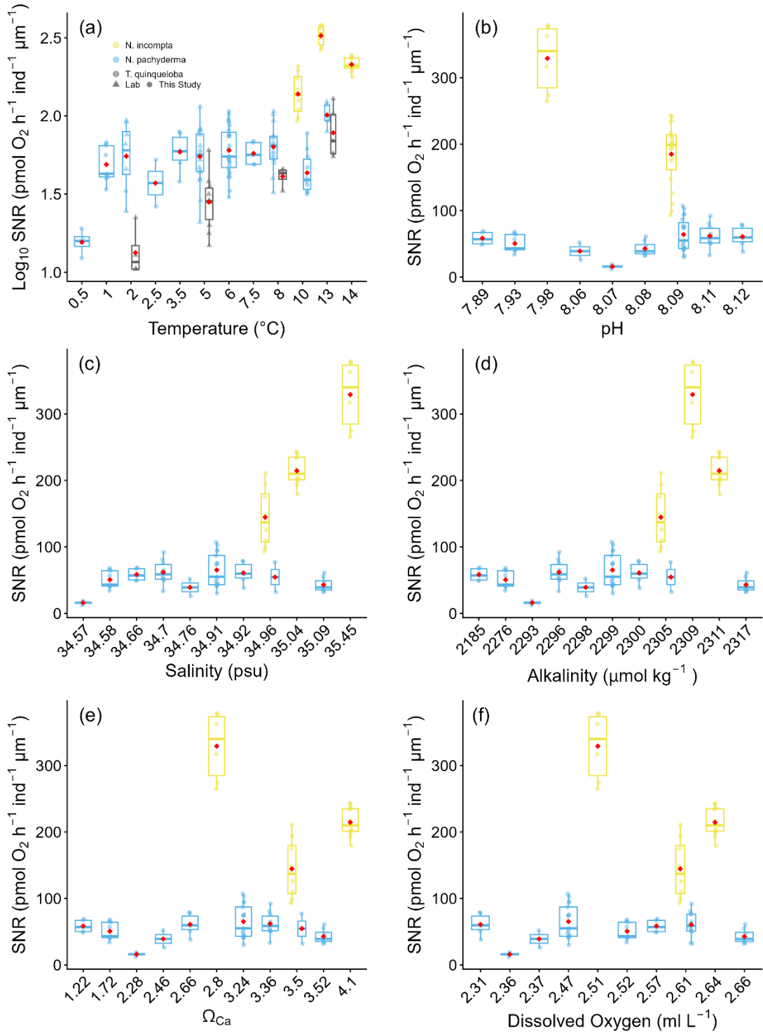
405 Figure 5: Box and whisker plots of the effect of essential climate variables on Size Normalised Respiration (SNR) based on \sqrt[3]{\text{cavity volume}} (pmol O 2 hr -1 ind -1 μm -1 ) in N. pachyderma , N. incompta and T. quinqueloba (a) Temperature °C and (b) pH; (c) Salinity (psu) and (d) Alkalinity (μmol kg -1 ); (e) Ω Ca and (f) Dissolved 410 Oxygen (ml L -1 ). Boxes extend from the data's lower to upper quartile values, with a line at the median. Whiskers indicate 1.5 times the interquartile distance. Red dots mark the mean. Log 10 Size normalised respiration and laboratory data are only available for (a). The source data for this figure is available in Tables S9 and S10.
