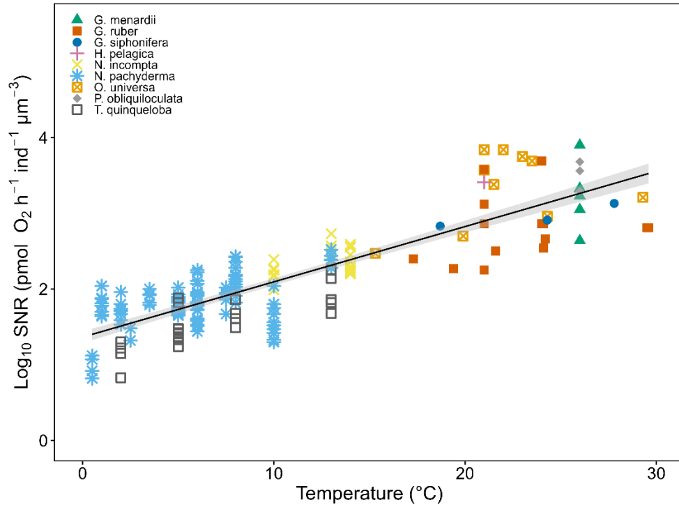
445 Figure 7: The effect of temperature (°C) on \log_{10} size-normalised respiration rate ( \text{pmol O}_2 \text{ hr}^{-1} \text{ ind}^{-1} \mu\text{m}^{-3} ) in this study and previously published data (Rink et al., 1998; Lombard et al., 2009 and Burke et al., 2025). The grey shaded regions represent the 95% confidence interval of the regression model. The source data for this figure is available in Table S11
