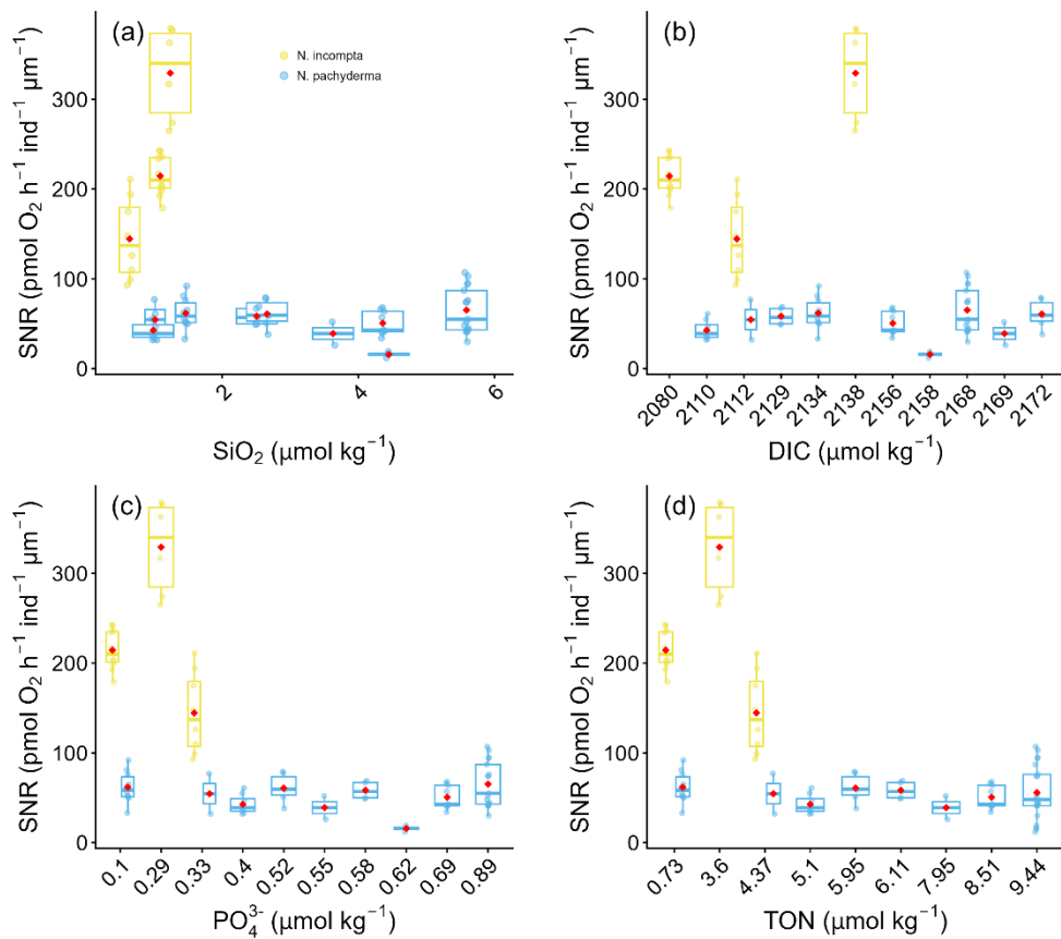
415 Figure 6: Box and whisker plots of the effect of nutrients on Size Normalised Respiration (SNR) based on \sqrt[3]{\text{cavity volume}} ( \text{pmol O}_2 \text{ hr}^{-1} \text{ ind}^{-1} \mu\text{m}^{-1} ) in N. pachyderma and N. incompta . (a) \text{SiO}_2 ( \mu\text{mol kg}^{-1} ) and (b) Dissolved Inorganic Carbon ( \mu\text{mol kg}^{-1} ); (c) \text{PO}_4^{3-} ( \mu\text{mol kg}^{-1} ) and TON ( \mu\text{mol kg}^{-1} ). Boxes extend from the lower to upper quartile values of the data, with a line at the median. Whiskers indicate 1.5 times the inter-quartile distance. The red dots mark the means. The source data for this figure is available in Table S9 and S10
