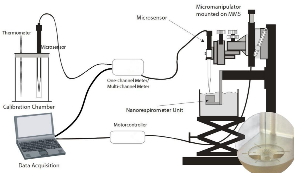
185 Figure 2 Diagram adapted from Unisense (2025) showing the nano respiration set-up used to measure oxygen gradients on single foraminifera. The image on the bottom right shows a close-up of the Nanorespirometer Unit (e.g., rosette) and microsensor entering one of the glass capillaries.
