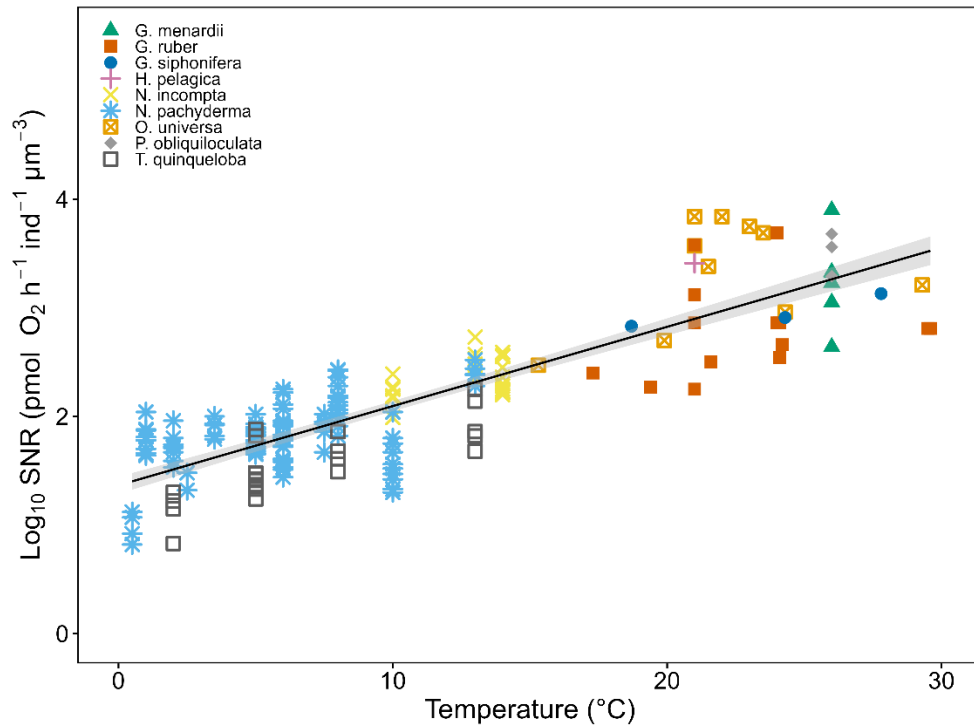
Figure 7: The effect of temperature (°C) on \log_{10} size-normalised respiration rate ( \text{pmol O}_2 \text{ hr}^{-1} \text{ ind}^{-1} \mu\text{m}^{-3} ) in this study and previously published data (Rink et al., 1998; Lombard et al., 2009 and Burke et al., 2025). The grey shaded regions represent the 95% confidence bounds interval of the regression model. The source data for this figure is available in Table S11
