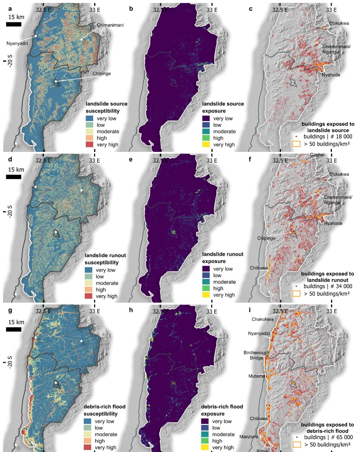
355 Fig. 7. Susceptibility and exposure levels. | Susceptibility, population and building exposure to a-c. landslide source, d-f. landslide runout, g-i. debris-rich flood. Hotspots of building exposure (> 50 buildings/km 2 ) are circled in orange. # indicates estimates of the number of buildings in moderate to very high exposure zones. Colour scales are comparable across the susceptibility and exposure maps.
