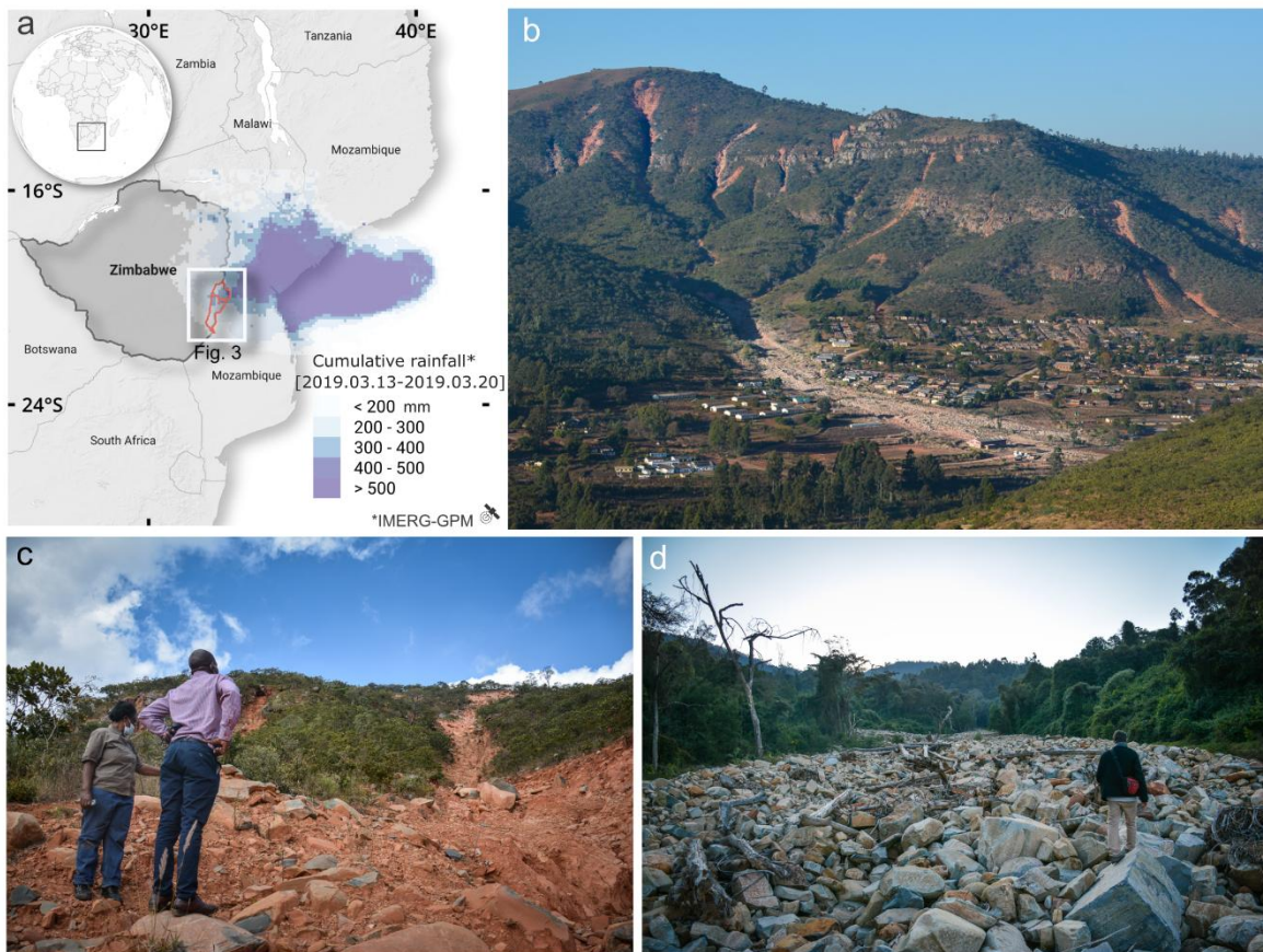
120 Fig. 1. Landslides and debris-rich flood triggered by Cyclone Idai in eastern Zimbabwe | a. Cumulative rainfall from March 13–20, 2019, estimated by IMERG-GPM satellite ( 0.1^\circ \times 0.1^\circ resolution; (Huffman et al., 2019)). Focus districts in eastern Zimbabwe are highlighted in red. b. Highly mobile landslides triggered by Cyclone Idai near Ngangu Township, Chimanimani (July 2021), with c. zoom on their runout zones and d. related debris-rich flood deposits. Panel b shows clear debris trails from shallow landslides, with evidence of erosion and entrainment, particularly visible in panel c, which contributed to severe impacts in Chimanimani Town. Photos taken ~2.5 years after the event (© M. Vanmaercke). 125
