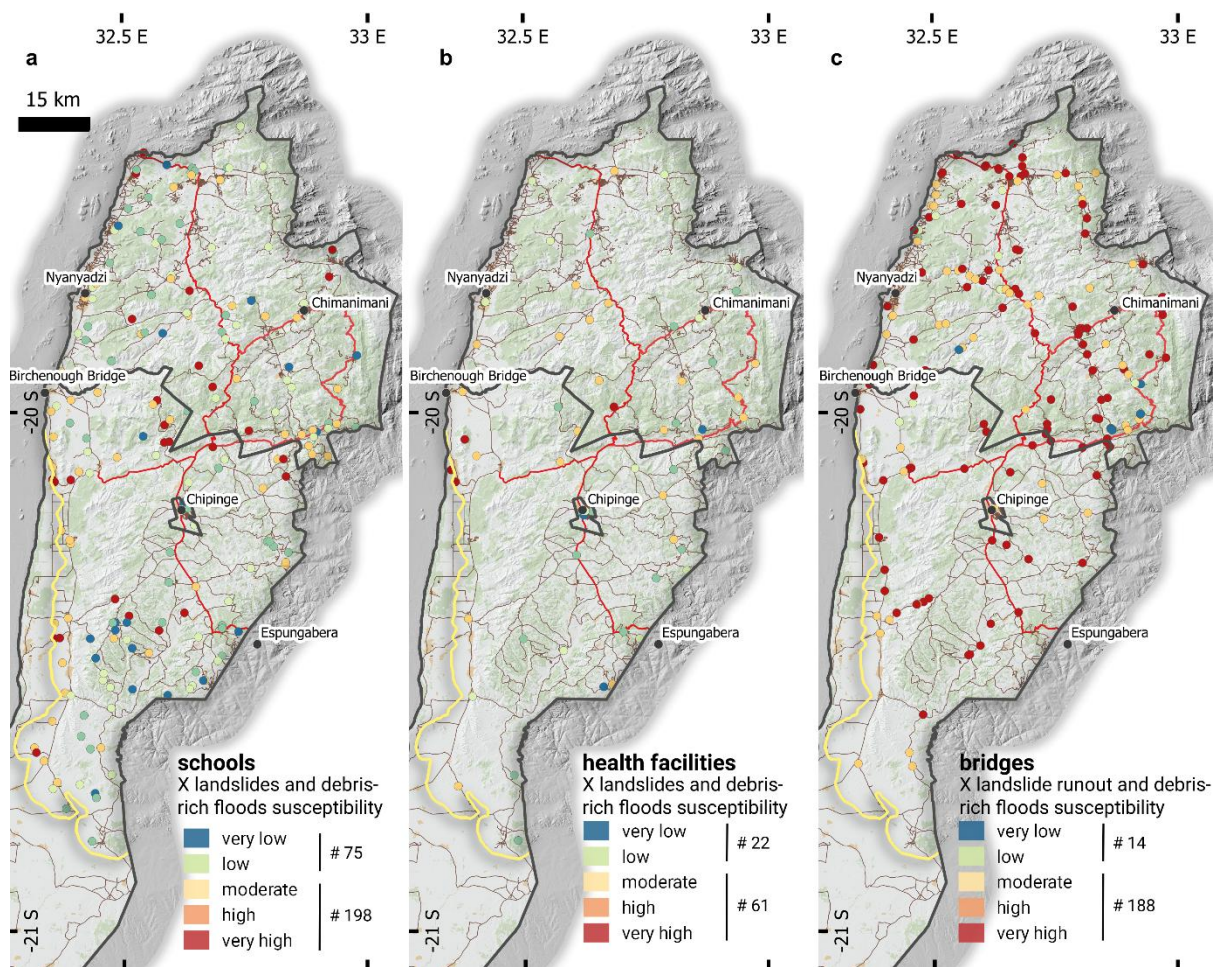
510 Fig A2. Infrastructure exposure. | a. Level of exposure of schools to landslides (source and runout) and debris-rich-floods. b. Level of exposure of health facilities to landslides (source and runout) and debris-rich-floods. c. Level of exposure of bridges to landslide runouts and debris-rich-floods. The # numbers indicate how many infrastructures are exposed per susceptibility classes. Bridge data © OpenStreetMap contributors 2024. Distributed under the Open Data Commons Open Database License (ODbL) v1.0.
