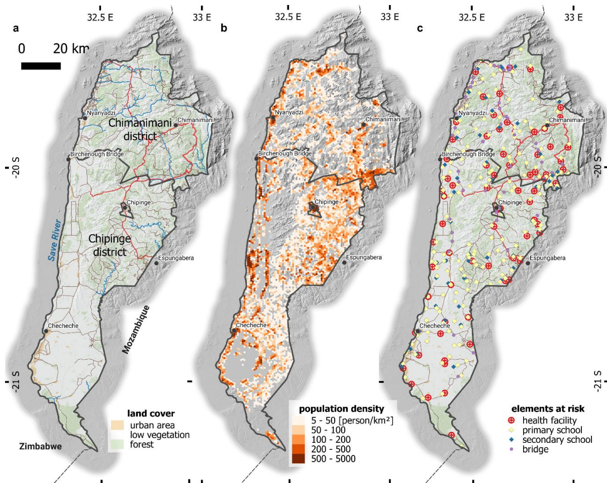
495 Fig. A1. Land cover, population density and key infrastructure in Chimanimani and Chipinge districts. | These layers were used to calculate the population and infrastructure exposure to landslide and debris-rich flood. Land cover: © ESA; population: © Facebook High Resolution Population Density Maps; key infrastructure: © UNESCO and © OpenStreetMap contributors 2024. Distributed under the Open Data Commons Open Database License (ODbL) v1.0.
