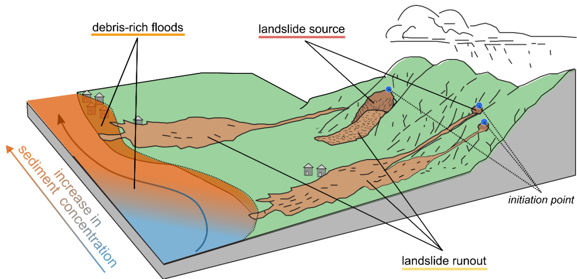
145 Fig. 2. | Illustration and definition of the landslide–debris-rich flood continuum, showing landslide source, landslide runout, and associated debris-rich flood zones as mapped in this study. Locations of the initiation points used during the manual inventory ( INV_02-POINT ) are also indicated. Adapted from Highland and Bobrowsky (2008).
