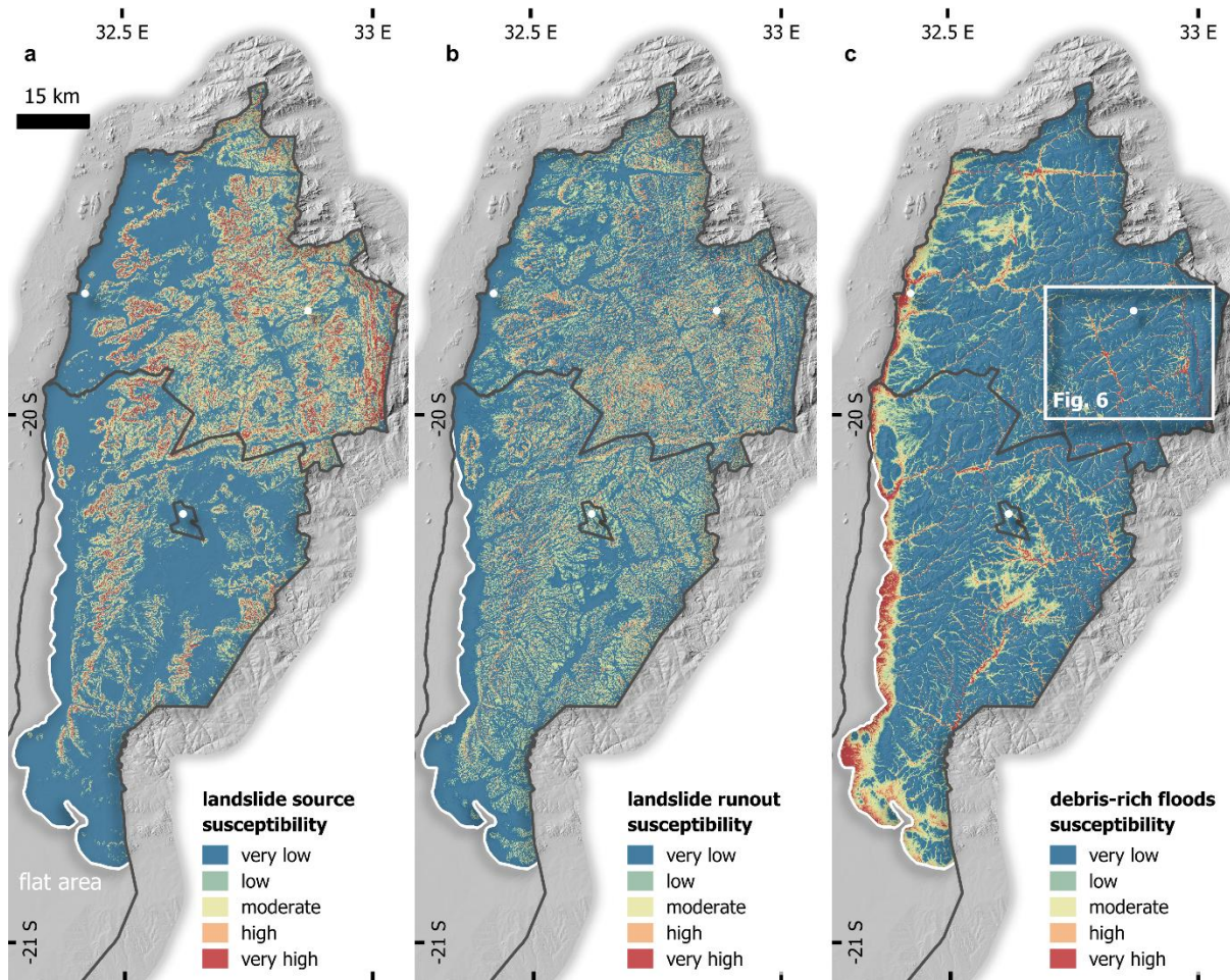
Figure 5. Susceptibility maps. | Maps showing susceptibility to a. landslide source, b. landslide runout and c. debris-rich flood in Chimanimani and Chipinge districts.
