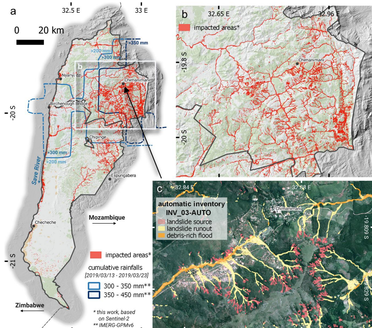
290 Fig. 4. Automatically detected impacted areas and classification (INV_03-AUTO). | a. Red zones indicates 295 areas affected by landslides or debris-rich floods (i.e., zones where the vegetation has been damaged, removed and/or covered by sediments) alongside Idai for Chimanimani (North) and Chipinge (South) districts. These zones were identified by comparing of pre and post-event Sentinel-2 composites. Pale blue and dark blue contours show cumulative rainfall >300 and >350 mm (satellite estimates) from 13–20 March 2019; other areas received \geq 200 mm. b. Zoom on impacted areas in Chimanimani district. Elongated shapes indicate debris-rich flood zones, while small features on upper hillslopes are landslides; long runouts often connect the two. c. Detailed zoom on Nangu Township, Chimanimani, showing automatic classification of landslide source, runout, and debris-rich flood (INV_03-AUTO). Definitions of these zones are illustrated in Fig. 2.
