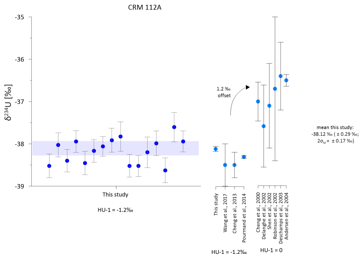
Figure 2: The CRM112A standard was repeatedly measured via the bracketing method with the HU-1 standard = -1.2 \text{ ‰} . The mean value of -38.12 \text{ ‰} \pm 0.29 \text{ ‰} is in line with other studies normalized to HU1 = -1.2 \text{ ‰} (Cheng et al., 2013; Pourmand et al., 2014; Wang et al., 2017) and is comparable with studies that normalise to HU-1 = 0 if the offset of +1.2 \text{ ‰} is applied (Cheng et al., 2000; Delanghe et al., 2002; Robinson et al., 2002; Shen et al., 2002; Deschamps et al., 2003; Andersen et al., 2004).
