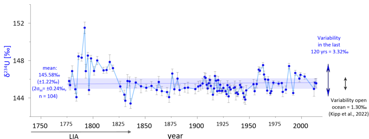
Figure 3: Annual \delta^{234}\text{U} measurements ( n = 104 ) of a 237-year-old coral. The mean of 145.58 ‰ is identical to the open ocean value of 145.55 ‰ ( \pm 0.28 ‰) (Kipp et al., 2022). The largest deviations from 143.40 ‰ to 151.50 ‰ were observed from 1778–1846 at the end of the Little Ice Age (LIA), with the peak value occurring in 1792. The variability in the coral \delta^{234}\text{U} over the last 165 years is approximately 2.5 times greater than the variance expected from observations in the open ocean (Kipp et al., 2022).
