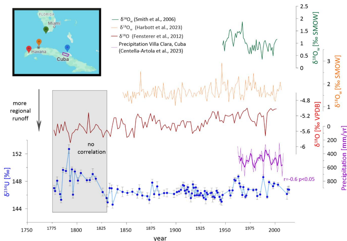
Figure 4: The \delta^{234}\text{U} values from the analysed coral in central northern Cuba (blue) are negatively correlated ( r = -0.60 , p < 0.05 ) with a precipitation record from the same region, starting in 1960 (purple; inverted y-axis) (Centella-Artola et al., 2023). Similar patterns are observed with \delta^{18}\text{O}_w values calculated from corals from southern Florida (green) (Smith et al., 2006) and northern Cuba (orange) (Harbott et al., 2023), with high \delta^{234}\text{U} values corresponding to high \delta^{18}\text{O}_w values. Additionally, since 1860, there has been a similar trend in the \delta^{18}\text{O} values from a stalagmite in northwestern Cuba, which are interpreted as a precipitation indicator (red) (Fensterer et al., 2012). These alignments show a visible influence of precipitation on the \delta^{234}\text{U} values of the coastal waters in which the coral lived, with low \delta^{234}\text{U} values representing greater runoff influences. In the period from 1778–1860, there appears to be no such trend between the stalagmite record and the coral record, likely indicating a substantial marine influence on the coral during the end of the Little Ice Age.
