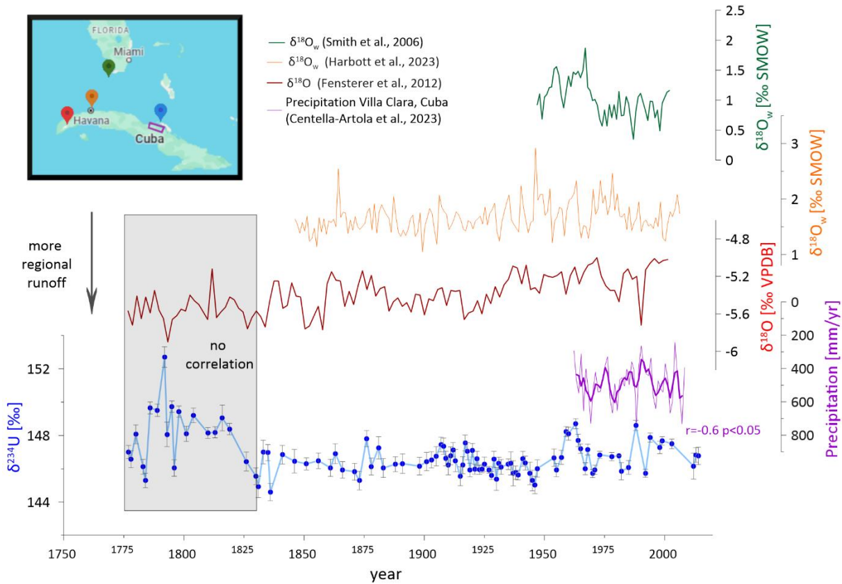
215 Figure 4: The \delta^{234}\text{U} values from the analysed coral in central northern Cuba (blue) are negatively correlated ( r = -0.60 , p < 0.05 ) with a precipitation record from the same region, starting in 1960 (purple; inverted y-axis) (Centella-Artola et al., 2023). Similar patterns are observed with \delta^{18}\text{O}_w values calculated from corals from southern Florida (green) (Smith et al., 2006) and northern Cuba (orange) (Harbott et al., 2023), with high \delta^{234}\text{U} values corresponding to high \delta^{18}\text{O}_w values. Additionally, since 1860, there has been a similar 220 trend in the \delta^{18}\text{O} values from a stalagmite in northwestern Cuba, which are interpreted as a precipitation indicator (red) (Fensterer et al., 2012). These alignments show a visible influence of precipitation on the \delta^{234}\text{U} values of the coastal waters in which the coral lived, with low \delta^{234}\text{U} values representing greater runoff influences. In the period from 1778–1860, there appears to be no such trend between the stalagmite record and the coral record, likely indicating a substantial marine influence on the coral during the end of the Little Ice Age.
