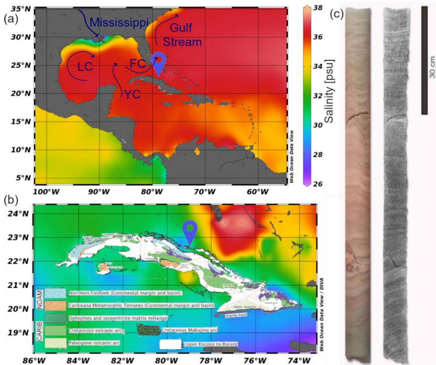
95 Figure 1: (a) Caribbean annual sea surface salinity with the location of the selected coral core on the northern shore of Cuba, directly 100 influenced by the Florida Current (FC) travelling eastwards from Yucatan Current (YC) and the Gulf of Mexico forming the Gulf Stream. The Loop Current (LC) carries the less saline Mississippi water towards the coral. (b) Annual sea surface salinity off the coast of Cuba; less salinity is observed at the core location due to terrestrial runoff. With generalized geologic-tectonic map of Cuba modified from (Iturralde-Vinent et al., 2016) (c) X-ray image of the slab used in the optical densitometry analysis and photograph of the analysed core (CSM-1) with visible green banding.
