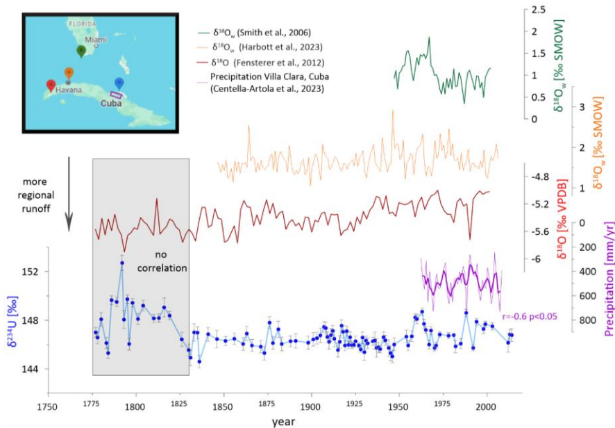
230 Figure 4: The \delta^{234}\text{U} values from the analysed coral in central northern Cuba (blue) are negatively correlated ( r = -0.60 , p < 0.05 ) with a precipitation record from the same region, starting in 1960 (purple; inverted y-axis) (Centella-Artola et al., 2023). Similar patterns 235 are observed with \delta^{18}\text{O}_w values calculated from corals from southern Florida (green) (Smith et al., 2006) and northern Cuba (orange) (Harbott et al., 2023), with high \delta^{234}\text{U} values corresponding to high \delta^{18}\text{O}_w values. Additionally, since 1860, there has been a similar trend in the \delta^{18}\text{O} values from a stalagmite in northwestern Cuba, which are interpreted as a precipitation indicator (Fensterer et al., 2012). These alignments show a visible influence of precipitation on the \delta^{234}\text{U} values of the coastal waters in which the coral lived, with low \delta^{234}\text{U} values representing greater runoff influences. In the period from 1778–1860, there appears to be no such trend between the stalagmite record and the coral record, likely indicating a substantial marine influence on the coral during the end of the Little Ice Age.
