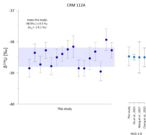
Figure 2: The CRM112A standard was repeatedly measured via the bracketing method with the HU-1 standard = -1.2 ‰. The measured mean value of -38.512 \pm 0.329 \text{ ‰} is in line with other studies normalized to HU1 = -1.2 ‰ (Cheng et al., 2013; Wang et al., 2017; Hu et al., 2025) and is comparable with studies that normalise to HU-1 = 0 if the offset of +1.2 ‰ is applied (Cheng et al., 2000; Delanghe et al., 2002; Robinson et al., 2002; Shen et al., 2002; Deschamps et al., 2003; Andersen et al., 2004).
