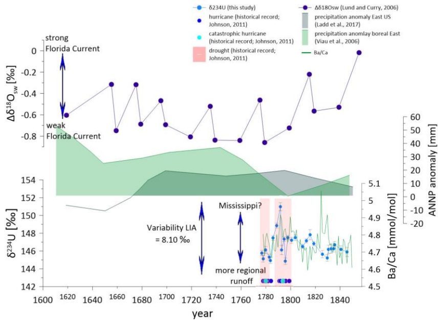
325 Figure 5: \delta^{234}\text{U} values (blue) from 1778–1850 plotted together with the timing of hydrological events documented in historical records (Johnson, 2011), indicating times of high hydrological fluctuation with droughts (red), hurricanes (dark blue), and catastrophic hurricanes (light blue). The green line shows Ba/Ca ratios of the coral core corresponding to the \delta^{234}\text{U} values. During these times, the \delta^{234}\text{U} values exhibited high variability, ranging from 143.40 ‰ to 151.50 ‰ in 1792. According to the present age model this high value occurred during a period of recurrent major hurricanes. Florida Current strength is inferred from \Delta\delta^{18}\text{O}_{\text{sw}} differences between the Gulf of Mexico and the Bahamas Channel (purple; (Lund & Curry, 2006)), where more negative values indicate a weaker current during the LIA. Superimposed precipitation anomalies over eastern North America (dark green; (Ladd et al., 2018)) and the boreal east (light green; (Viau et al., 2006)) show enhanced precipitation during this same interval, consistent with a weakened Florida Current and elevated variability in \delta^{234}\text{U} values.
