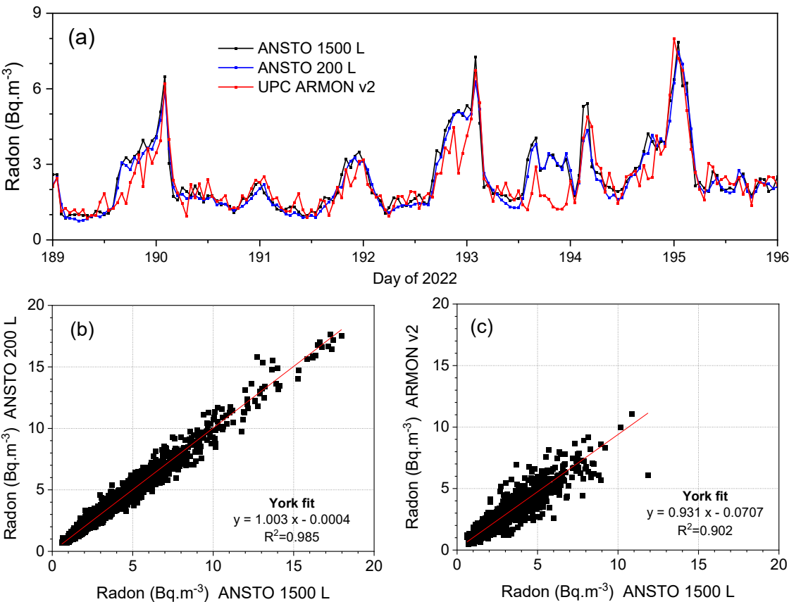
850 Figure 18: (a) 7-day comparison of hourly radon observations from 100 m on the Saclay tower between ANSTO 1500 L and ANSTO 200 L two-filter detectors and the UPC ARMON v2. (b) linear regressions between the ANSTO 200 L and ANSTO 1500 L monitor (over the complete 4-month ICP), and (c) linear regressions between the ARMON v2 and the ANSTO 1500 L for only 38 days of the ICP (ICOS, 2018, 2025; Ramonet et al., 2025). Full ICP dataset for the ARMON v2 will be presented in a subsequent manuscript currently in review.
